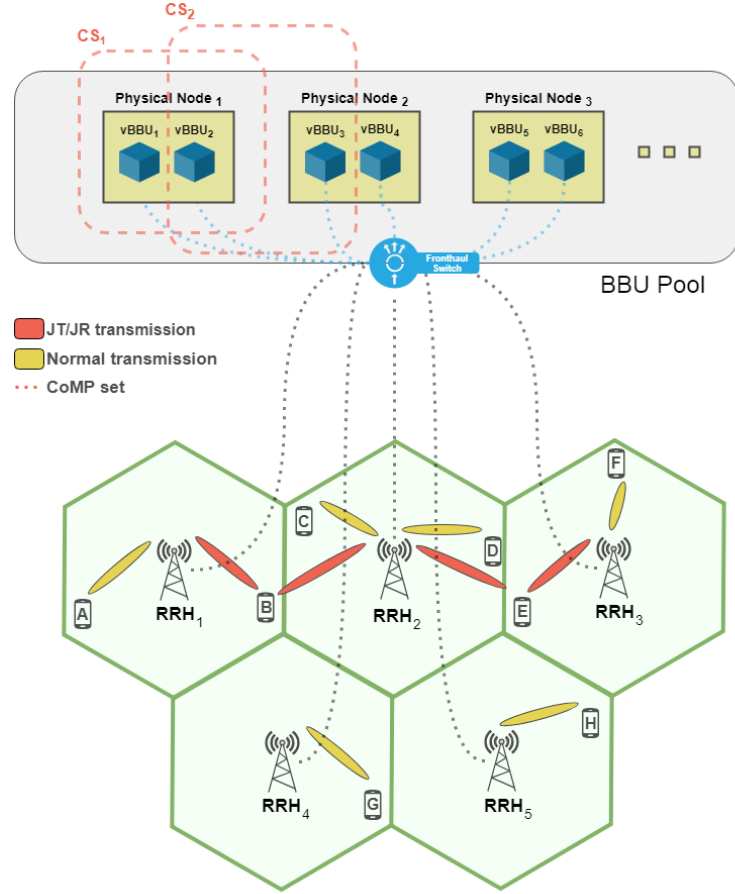
Figure 4.2. CoMP activity for two user equipment
