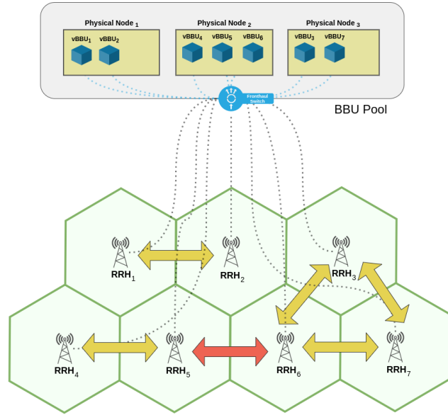
Figure 5.4. A new CoMP configuration changes vBBU clusters vBBU clusters become \{vBBU_1, vBBU_2\} and \{vBBU_3, vBBU_4, vBBU_5, vBBU_6, vBBU_7\}
