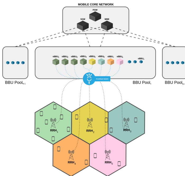
Figure 3.1. CloudRAN architecture
