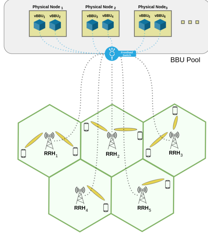
Figure 4.1. CloudRAN architecture with virtual BBUs in the BBU pool
