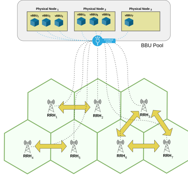
Figure 5.1. CoMP pairings between RRHs
