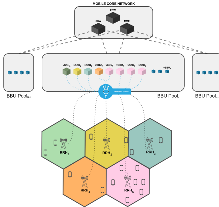
Figure 3.2. CloudRAN architecture after a population shift
