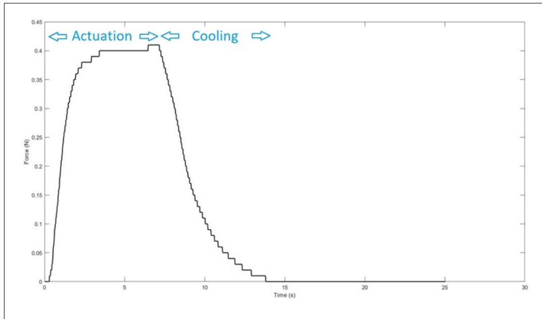
Figure 3.7 Force profile of the spring actuated with 370 mA.
