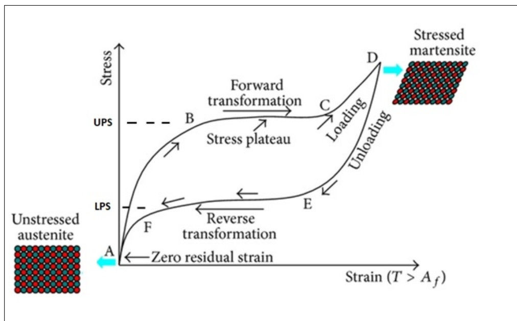
Figure 1.4 Typical stress curve of a SMA at a temperature above A_f [5].
