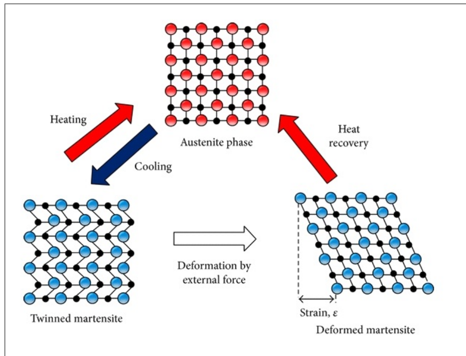
Figure 1.1 Phase transformation of a SMA in crystal structure [2].
