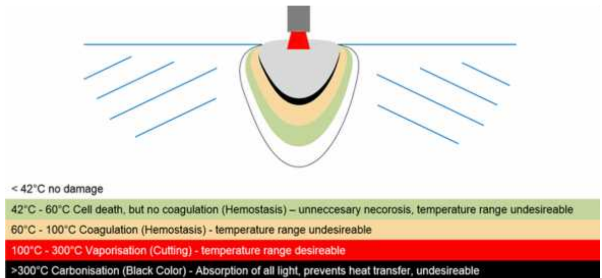
Figure 2.8. Photothermal effect [17]
