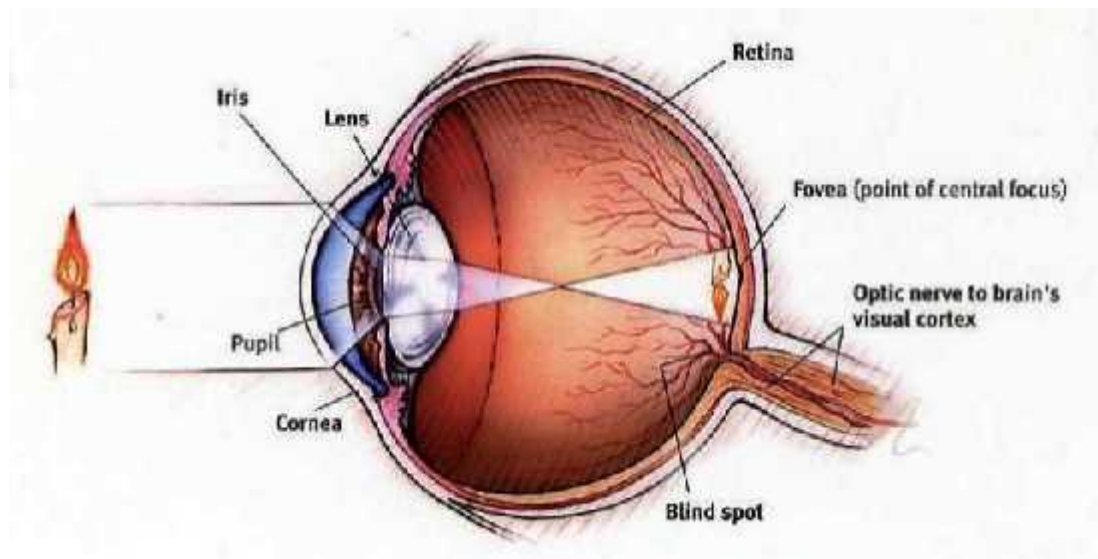
Figure 2.2. Focusing Light rays [7]
