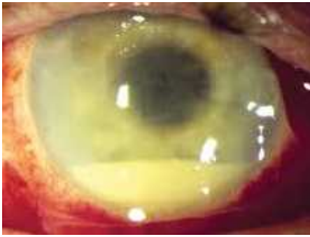
Figure 2.20. Endophthalmitis [40]
