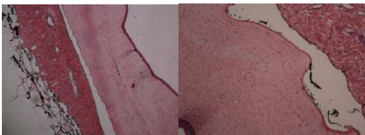
Figure 4.7. 1070nm 1,5W-10sec.
