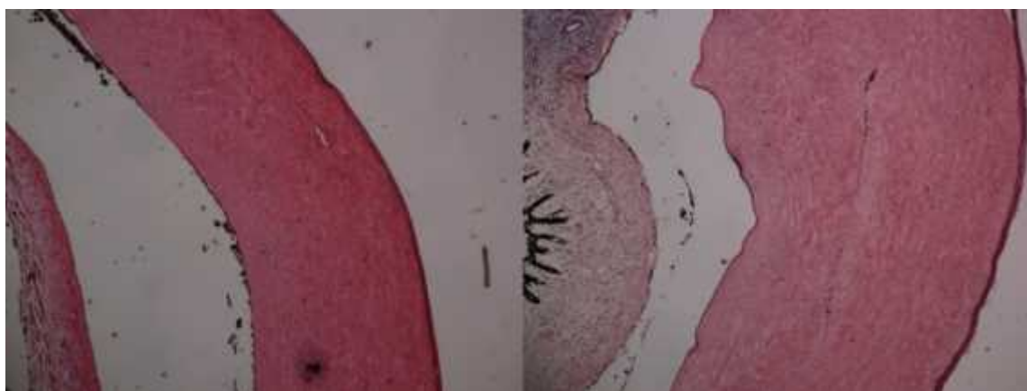
Figure 4.5. 980nm 2W-20sec.
