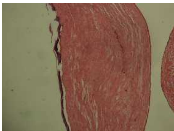
Figure 4.11. 1070nm 1,5W-5sec.
