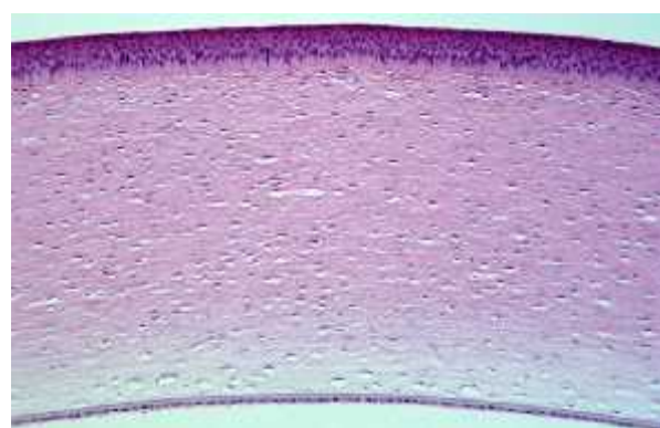
Figure 2.17. Stromal collagen [37]
