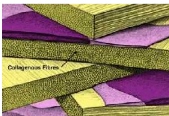
Figure 2.16. Collagen arrangement [36]
