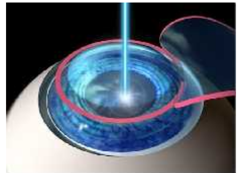
Figure 2.7. LASIK [16]
