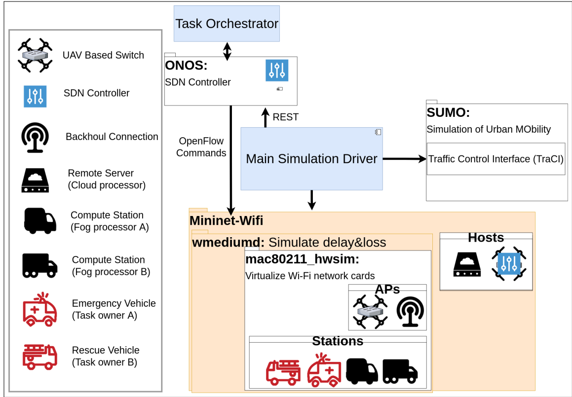
Figure 4.1. System components.
