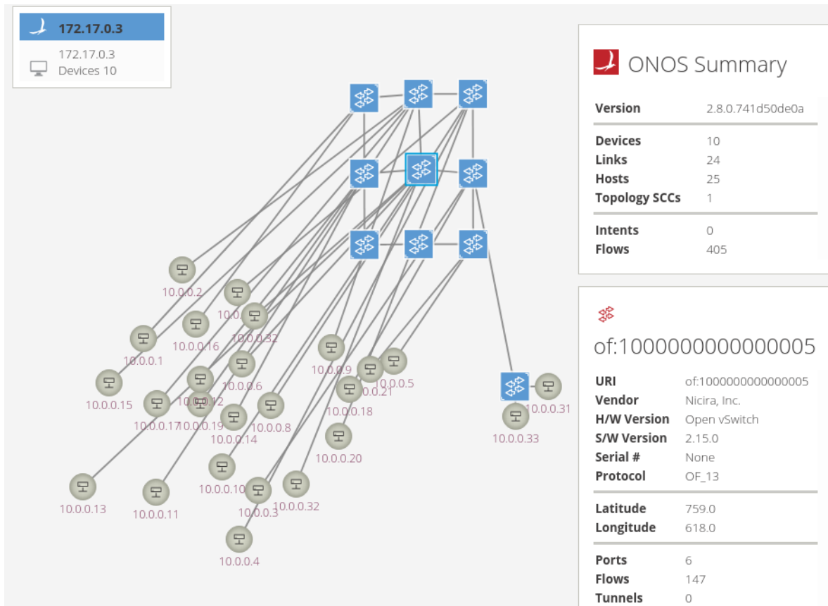
Figure 4.4. Network topology.
