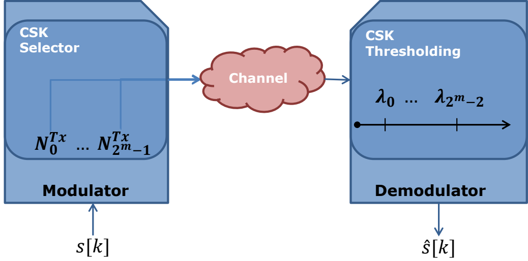
Figure 5.2. Concentration-based modulator and demodulator.
