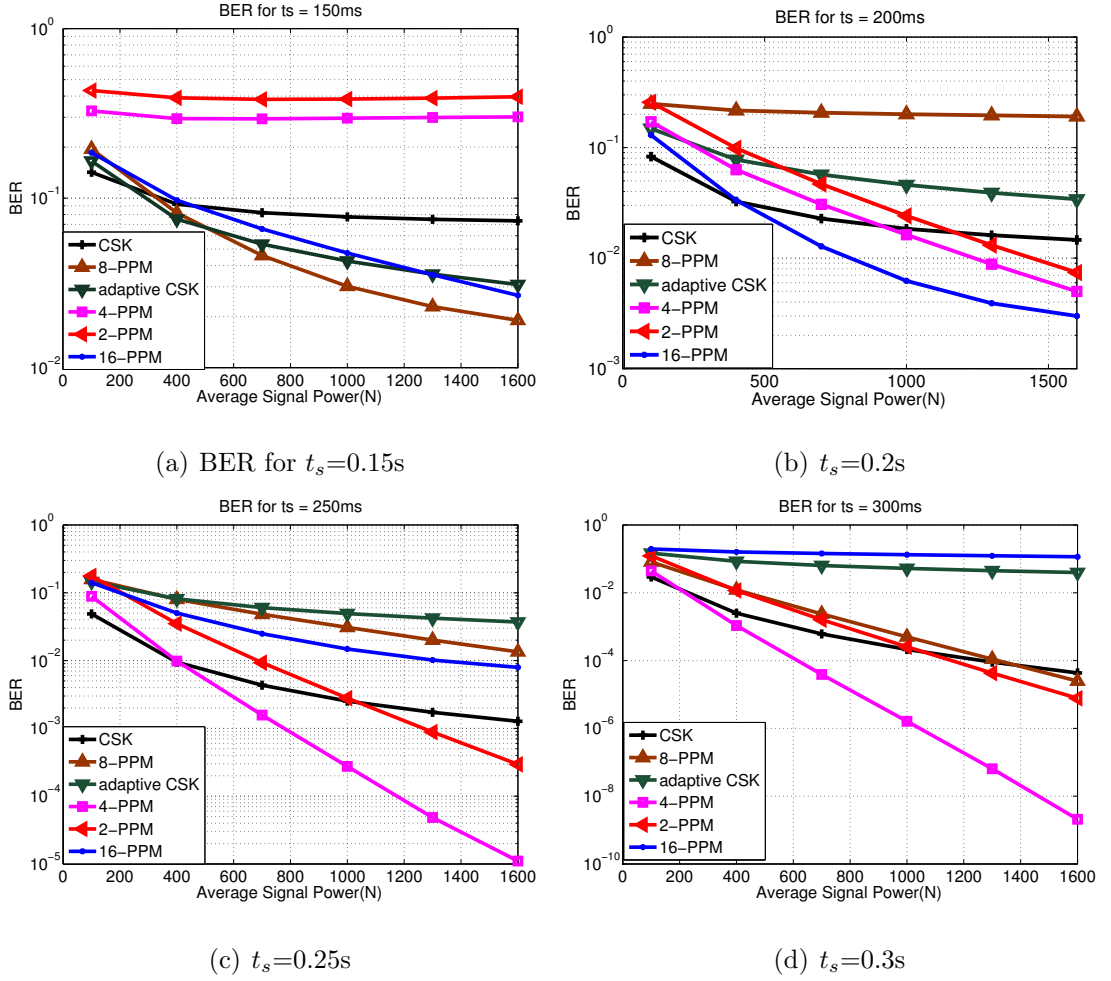
Figure 2.3. BER of the PPM modulations and CSK for different t_s . The t_s indicated on each figure corresponds to slot duration of CSK (hence bit duration for CSK) and it is adjusted for other modulations for fair comparison
