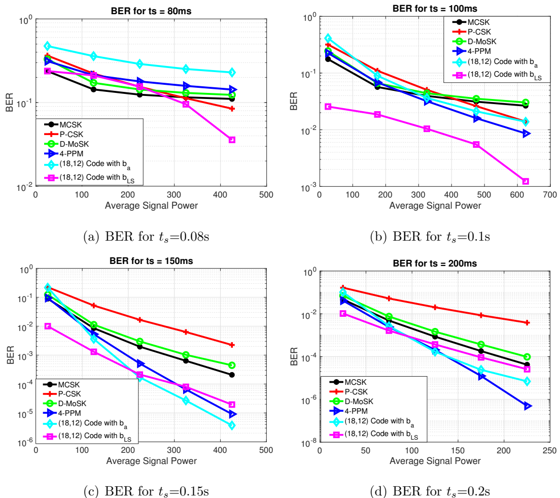
Figure 3.1. BER comparison of the our proposed coding method with 4-PPM, MCSK, D-MoSK and P-CSK for different t_s values. The t_s indicated on each figure belongs to MCSK, P-CSK and 4-PPM and it is adjusted for D-MoSK as 2t_s for fair comparison
