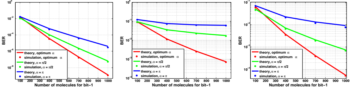
(a) BER curves for t_s=300\text{ms} and d = 5 \mu\text{m} (b) BER curves for t_s=300\text{ms} and d = 7 \mu\text{m} (c) BER curves for t_s=400\text{ms} and d = 7 \mu\text{m}
