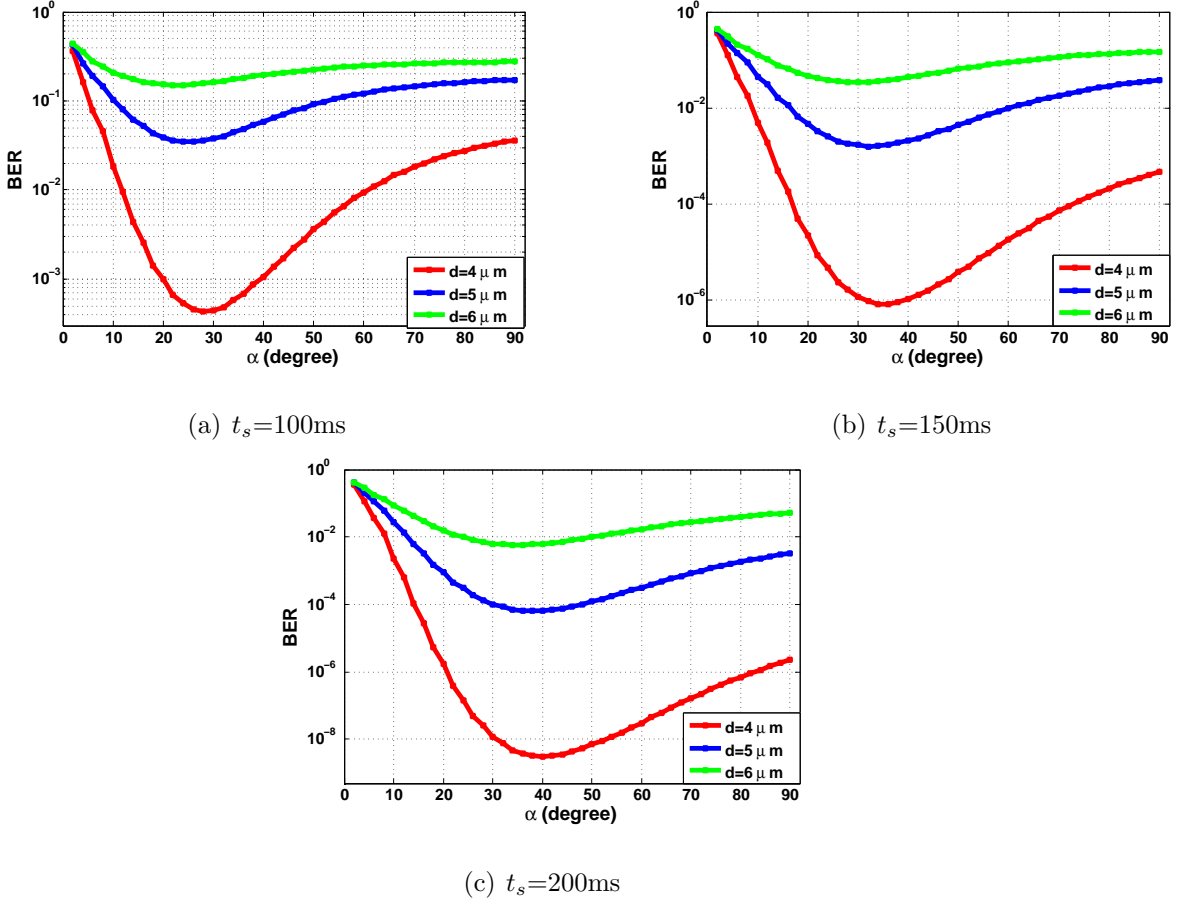
Figure 5.12. BER vs \alpha curves for r_r = 5 \mu\text{m} , D = 80 \mu\text{m}^2/\text{s} and N_1^{\text{Tx}} = 500 with different d=r_0-r_r values.
