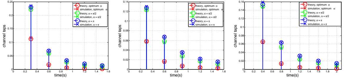
(d) channel taps for t_s=300\text{ms} and d = 5 \mu\text{m} (e) channel taps for t_s=300\text{ms} and d = 7 \mu\text{m} (f) channel taps for t_s=400\text{ms} and d = 7 \mu\text{m}
