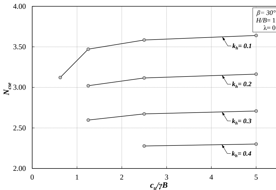
Figure 4.4. Variation of N_{cse} with c_u/\gamma B for all k_h values ( \beta = 30^\circ , H/B = 1 , \lambda = 0 ).
