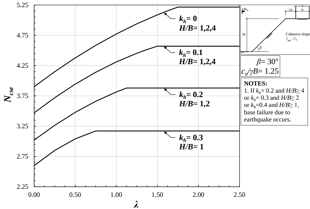
Figure 4.19. Design chart for seismic bearing capacity factor of surficial strip footings near cohesive slopes ( \beta = 30^\circ , c_u/\gamma B = 1.25 , H/B = 1, 2, 4 ).
