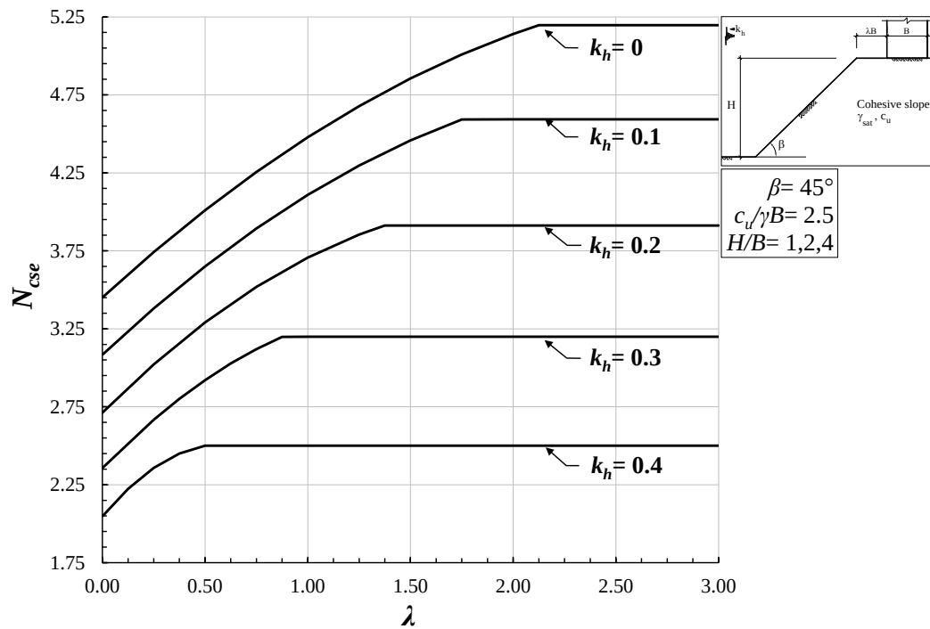
Figure 4.22. Design chart for seismic bearing capacity factor of surficial strip footings near cohesive slopes ( \beta = 45^\circ , c_u/\gamma B = 2.5 , H/B = 1, 2, 4 ).
