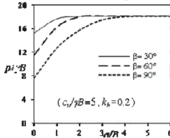
Figure 2.43. Variation of seismic bearing capacity with a/B (Farzaneh et al. , 2013).
