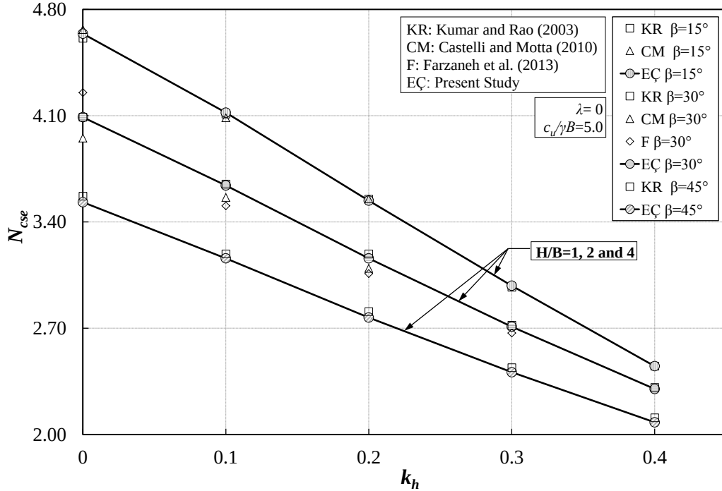
Figure 3.20. Variation of N_{cse} with k_h for all slope angles (For \lambda = 0 , c_u/\gamma B = 5 ).
