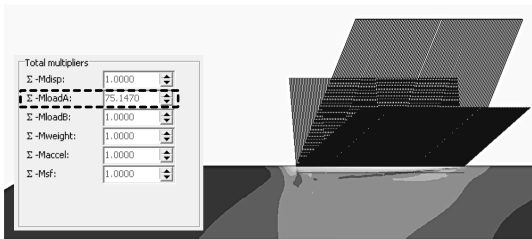
Figure 4.49. Load multiplier ( \Sigma -MloadA) and the failure mechanism obtained by Plaxis 2D for the design example 6.
