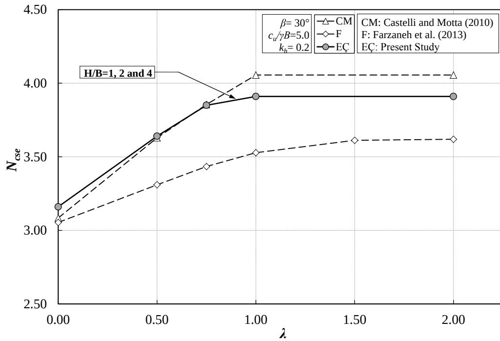
Figure 3.21. Variation of N_{cse} with \lambda (For \beta = 30^\circ , c_u/\gamma B = 5 , k_h = 0.2 ).
