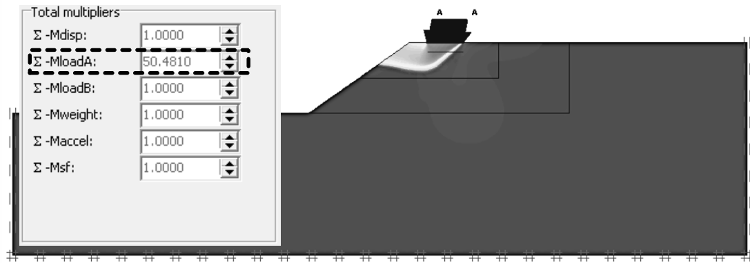
Figure 4.34. Load multiplier ( \Sigma -MloadA) and the failure mechanism obtained by Plaxis 2D for the design example 2.
