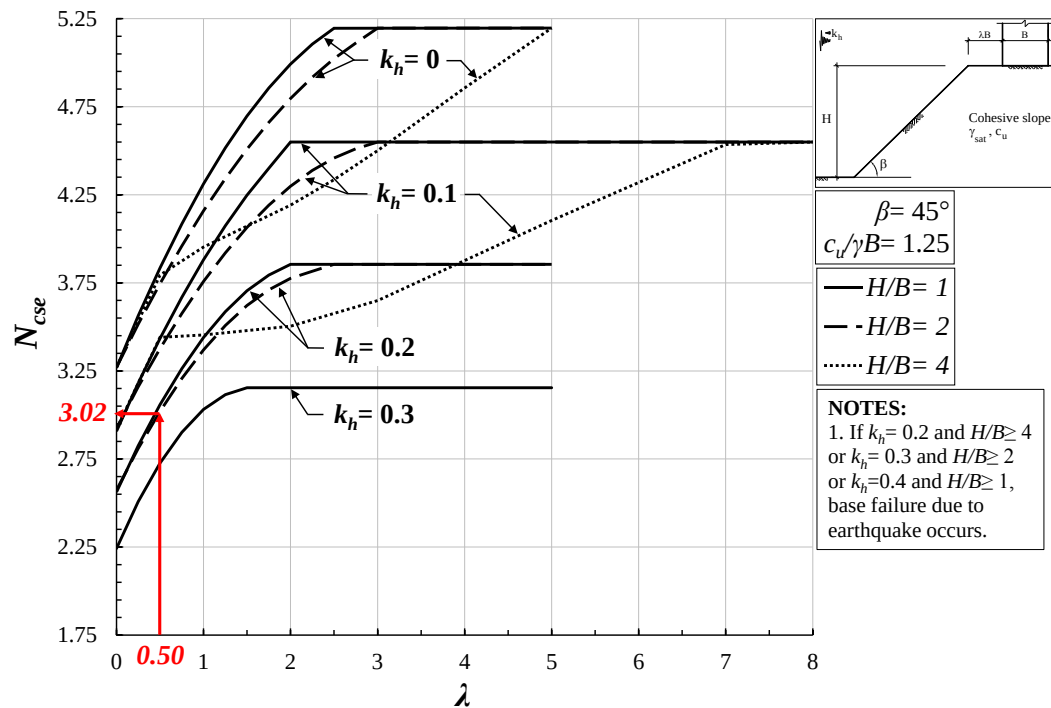
Figure 4.33. The second N_{cse} value to be used in linear interpolation for the design example 2.
