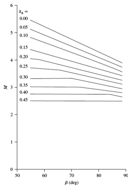
Figure 2.49. Variation of N_2 with \beta \geq 55 and k_h (Koppula, 1984) (Adapted from Das and Ramana, 2010).
