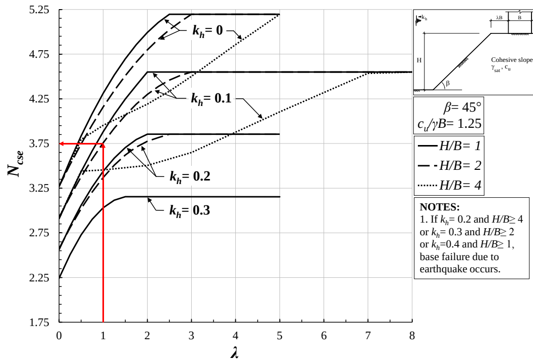
Figure 4.38. The second N_{cse} value to be used in linear interpolation for the design example
