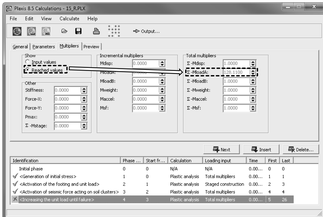
Figure 3.15. The load multiplier ( \Sigma - MloadA ) obtained by using Calculations module of Plaxis 2D for the ultimate limit state.
