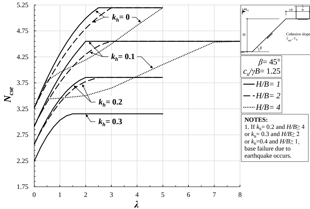
Figure 4.23. Design chart for seismic bearing capacity factor of surficial strip footings near cohesive slopes ( \beta = 45^\circ , c_u/\gamma B = 1.25 , H/B = 1, 2, 4 ).
