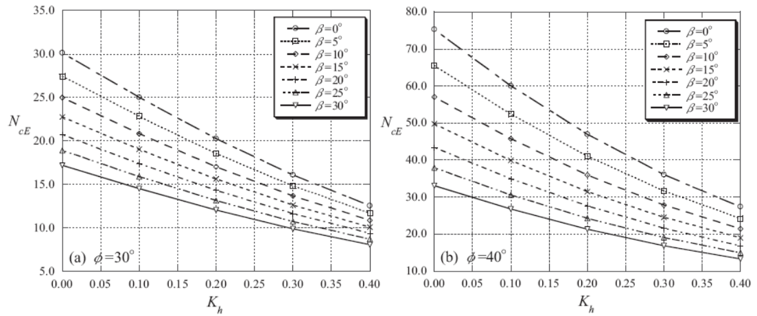
Figure 2.37. Design charts for N_{ce} ( \Phi = 30^\circ, 40^\circ, D/B = 0, a = 0.5 ) (Yamamoto, 2010).
