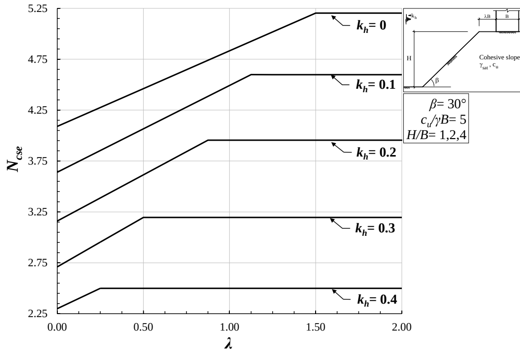
Figure 4.17. Design chart for seismic bearing capacity factor of surficial strip footings near cohesive slopes ( \beta = 30^\circ , c_u/\gamma B = 5 , H/B = 1, 2, 4 ).
