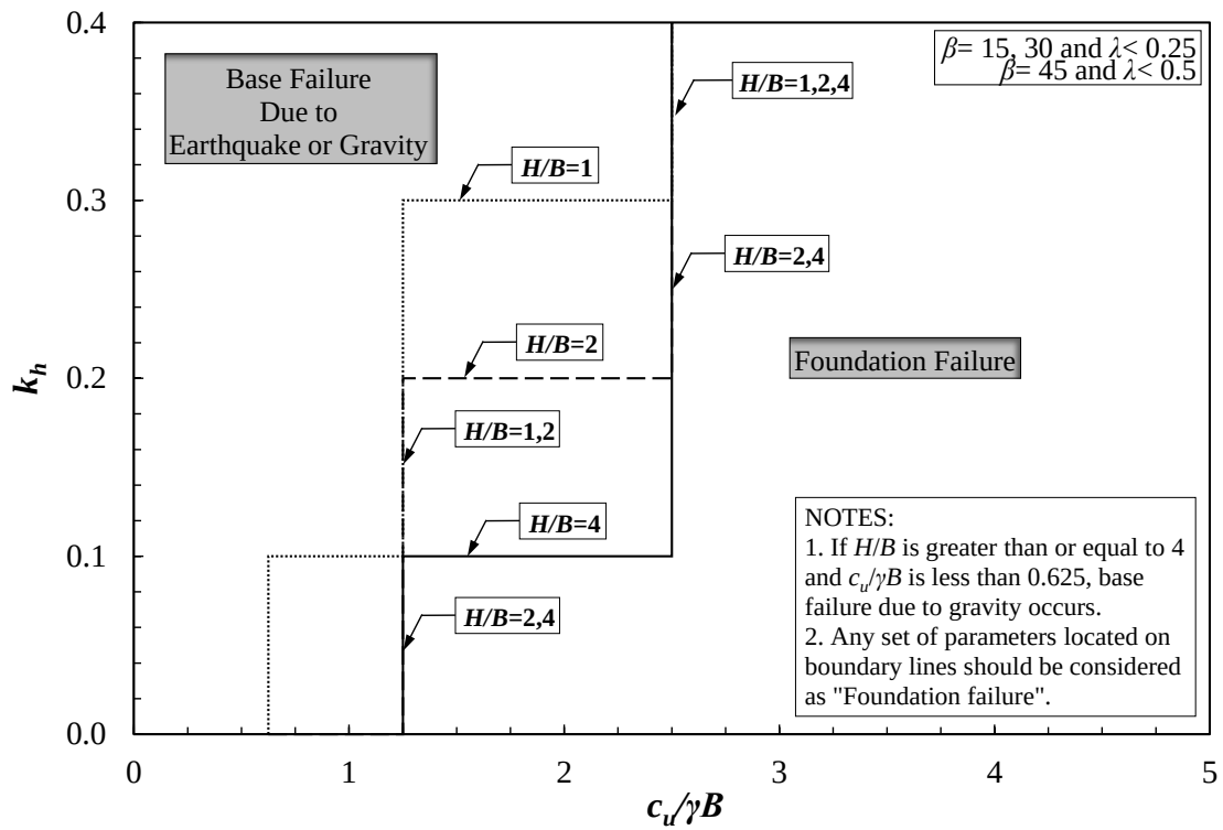
Figure 4.11. Variation of failure modes with influential parameters ( \lambda < 0.25 or 0.5 ).
