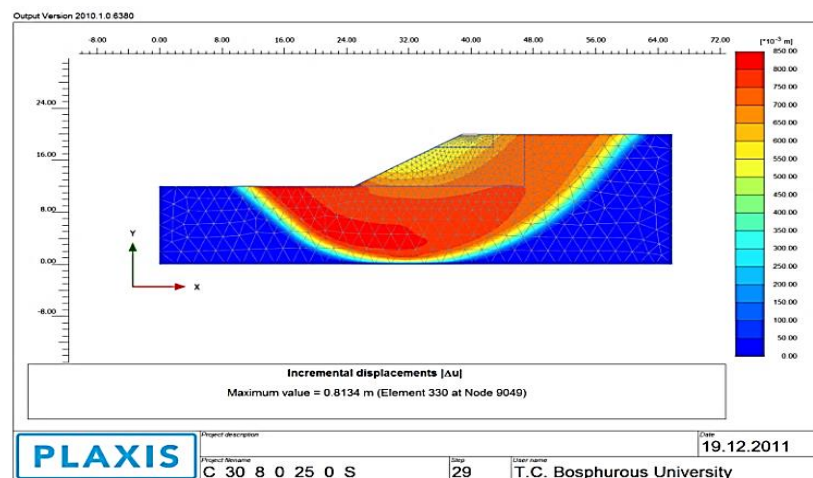
Figure 3.23. Failure mechanism of unstable cohesive slope in static condition ( \beta=30^\circ , H=8.0 m and c_u=25 kPa).
