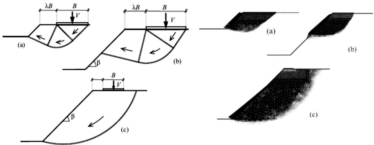
Figure 2.11. Failure modes (a) and (b) bearing capacity failure and (c) overall slope failure (Georgiadis, 2010).
