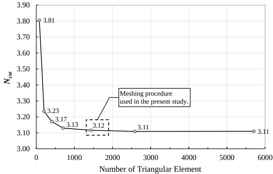
Figure 3.13. Variation of N_{cse} with the number of triangular elements ( \beta= 30^\circ , H= 4.0\text{m} , \lambda= 0 , c_u= 100\text{kPa} , k_h= 0.2 ).
