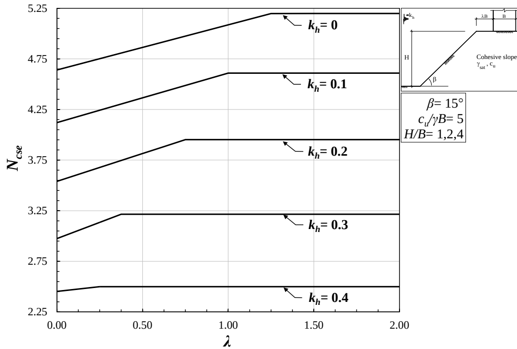
Figure 4.13. Design chart for seismic bearing capacity factor of surficial strip footings near cohesive slopes ( \beta = 15^\circ , c_u/\gamma B = 5 , H/B = 1, 2, 4 ).
