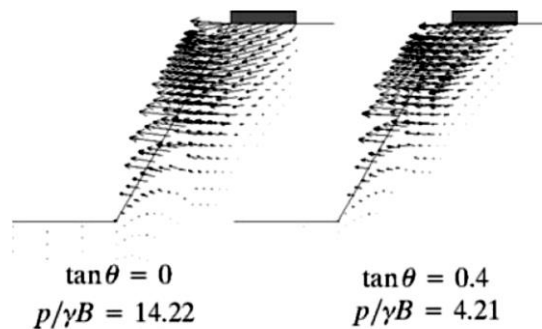
Figure 2.30. Comparison of upper bound velocity diagrams for the effect of inertia forces (Shiau et al. , 2006).
