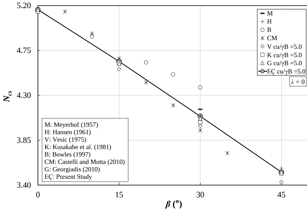
Figure 3.18. Variation of N_{cs} with \beta (For \lambda=0 , c_u/\gamma B=5 ).
