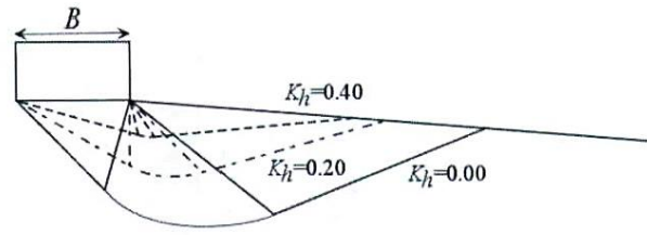
(a) \phi = 30^\circ , \beta = 5^\circ , \alpha = 0.0 , K_h = 0.00, 0.20 and 0.40 .
