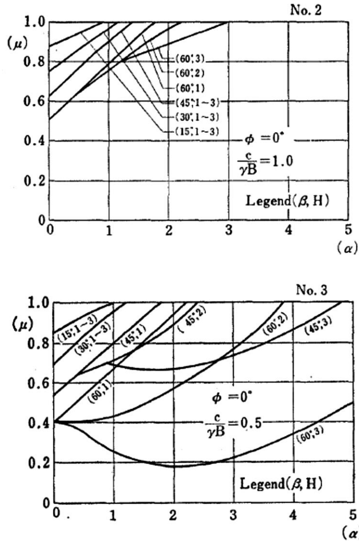
Figure 2.9. No.2 and No.3 design charts presented to calculate dimensionless factor (\mu) (Kusakabe et al. , 1981).
