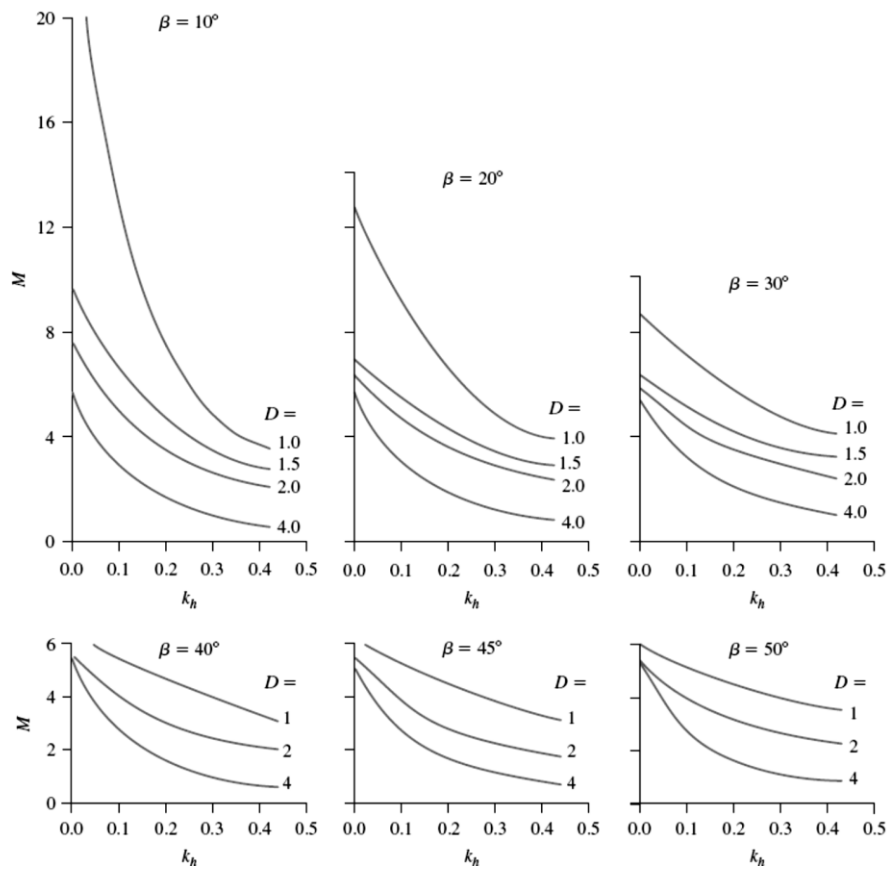
Figure 2.48. Variation of N_2 with k_h and \beta (Koppula, 1984) (Adapted from Das and Ramana, 2010).
