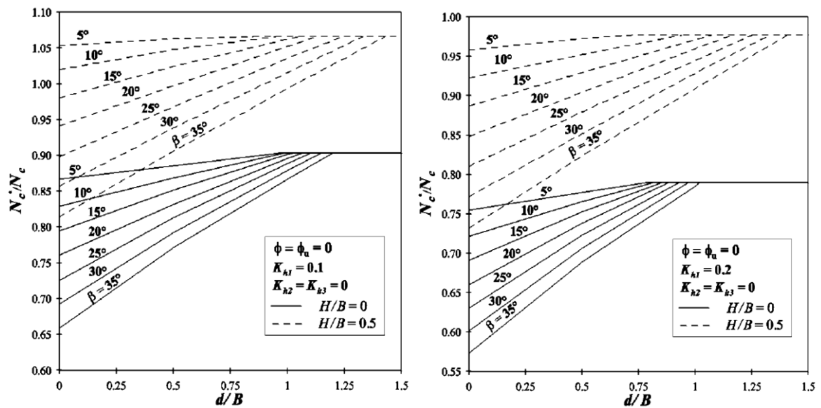
Figure 2.41. N_c^*/N_c ratios as a function of the normalized d/B slope distance (Castelli and Motta, 2010).
