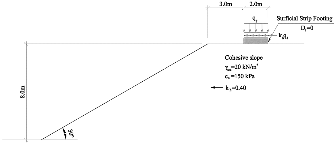
Figure 4.47. Schematic representation of the design example 5
