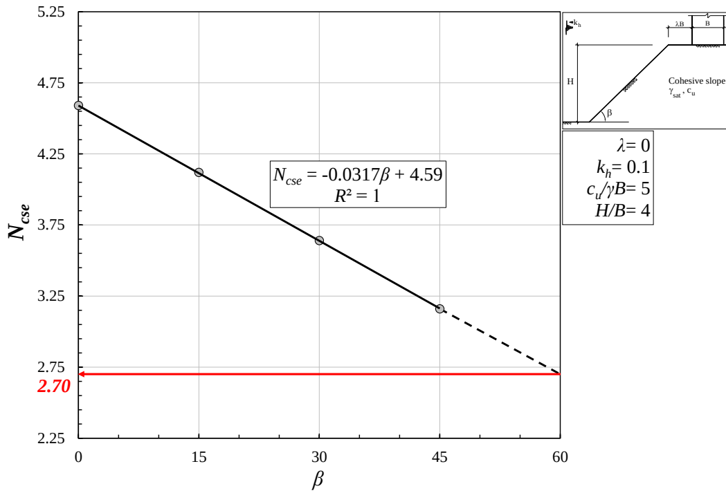
Figure 4.41. Linear relationship between N_{cse} - \beta .
