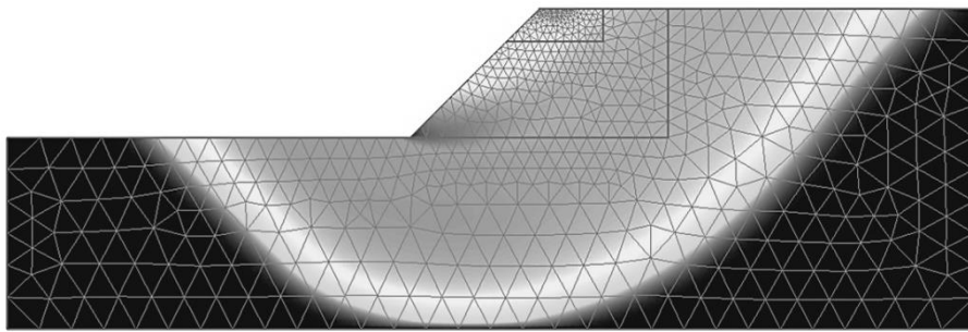
Figure 4.5. Base failure due to self-weight of cohesive slope ( \beta = 45^\circ , H/B = 4 , c_u/\gamma B = 0.625 ).
