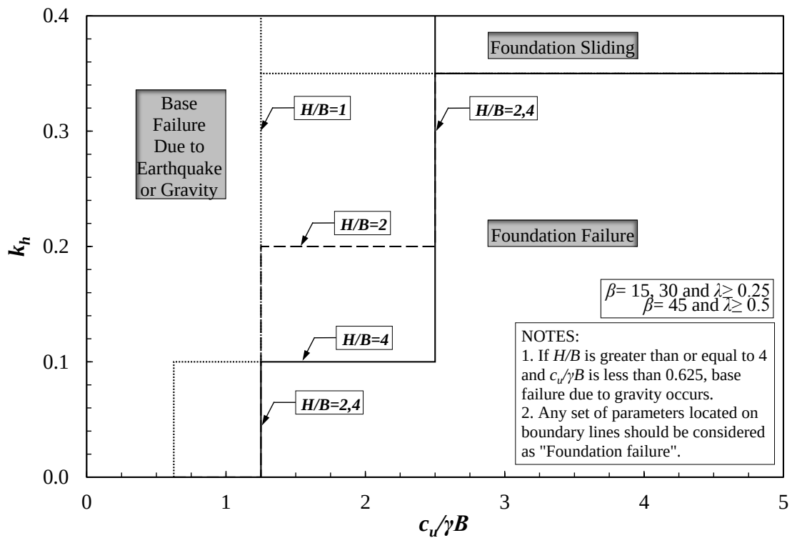
Figure 4.12. Variation of failure modes with influential parameters ( \lambda \geq 0.25 or 0.5 ).
