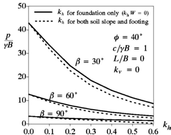
Figure 2.32. Effect of soil inertia k_h on p/\gamma B (Shiau et al. , 2006).
