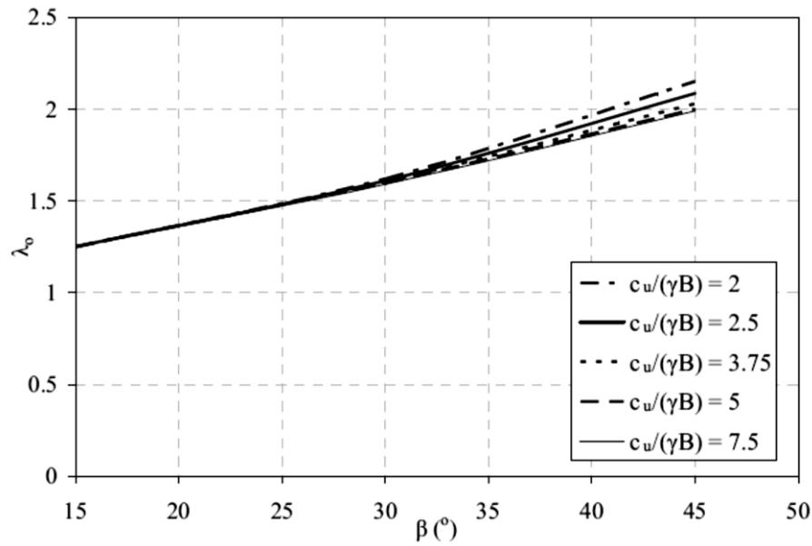
Figure 2.17. Variation of \lambda_o with \beta (Georgiadis, 2010).
