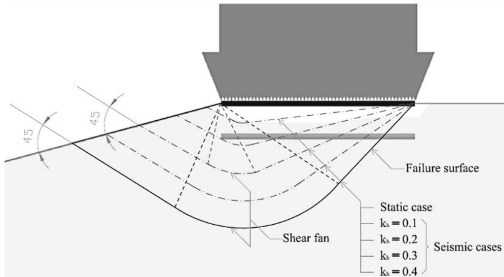
Figure 4.25. Geometry of failure mechanisms obtained at the ultimate state for all k_h values.
