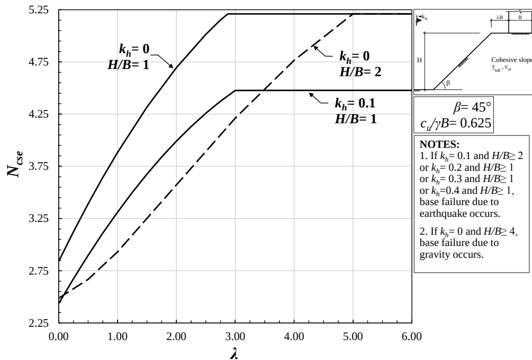
Figure 4.24. Design chart for seismic bearing capacity factor of surficial strip footings near cohesive slopes ( \beta = 45^\circ , c_u/\gamma B = 0.625 , H/B = 1, 2, 4 ).
