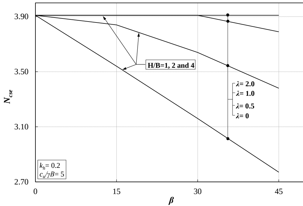
Figure 4.2. Variation of N_{cse} with \beta for all \lambda values ( k_h = 0.2 , c_u/\gamma B = 5 ).
