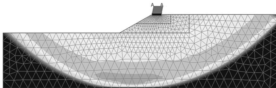
Figure 4.6. Base failure due to earthquake inertia force ( \beta = 30^\circ , H/B = 2 , c_u/\gamma B = 0.625 , k_h = 0.2 ).
