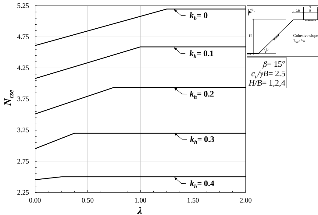
Figure 4.14. Design chart for seismic bearing capacity factor of surficial strip footings near cohesive slopes ( \beta = 15^\circ , c_u/\gamma B = 2.5 , H/B = 1, 2, 4 ).
