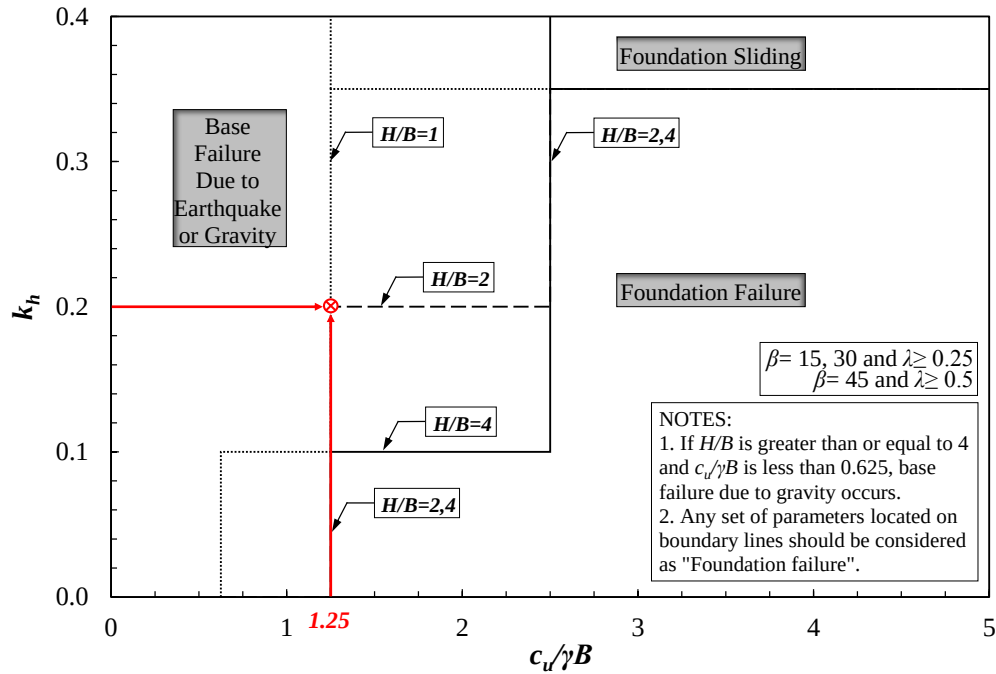
Figure 4.31. Estimation of the failure mode for the design example 2.
