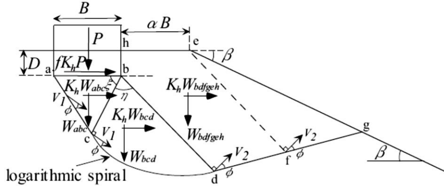
Figure 2.33. Failure mechanism used in the analysis (Yamamoto, 2010).
