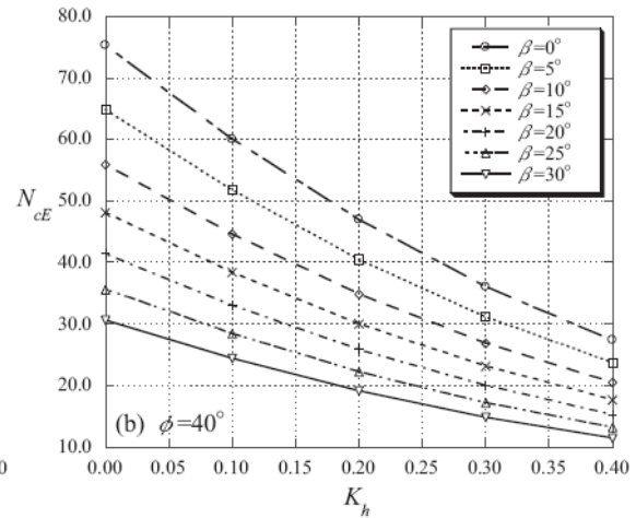
Figure 2.35. Design charts for N_{ce} ( \Phi = 30^\circ, 40^\circ , D/B = 0 , a = 0.0 ) (Yamamoto, 2010).
