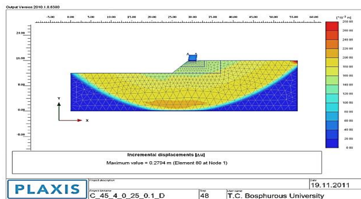
Figure 3.27. Failure mechanism of unstable cohesive slope in seismic condition ( \beta= 45^\circ , H=4.0 m, c_u= 25 kPa, k_h= 0.1 ).
