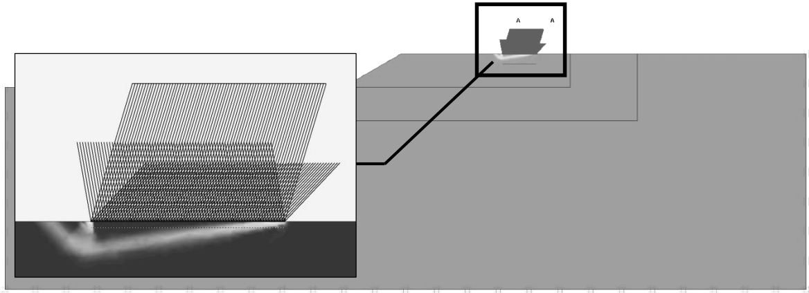
Figure 3.17. Shear surfaces obtained for the finite element model named as C_30_2_3_200_0.3_D and enlarged view of the shear surfaces.
