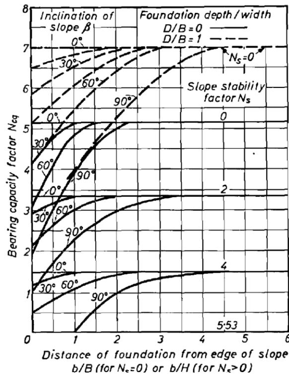
Figure 2.4. Bearing capacity factors for strip foundation on top of purely cohesive slope (Meyerhof, 1957).
