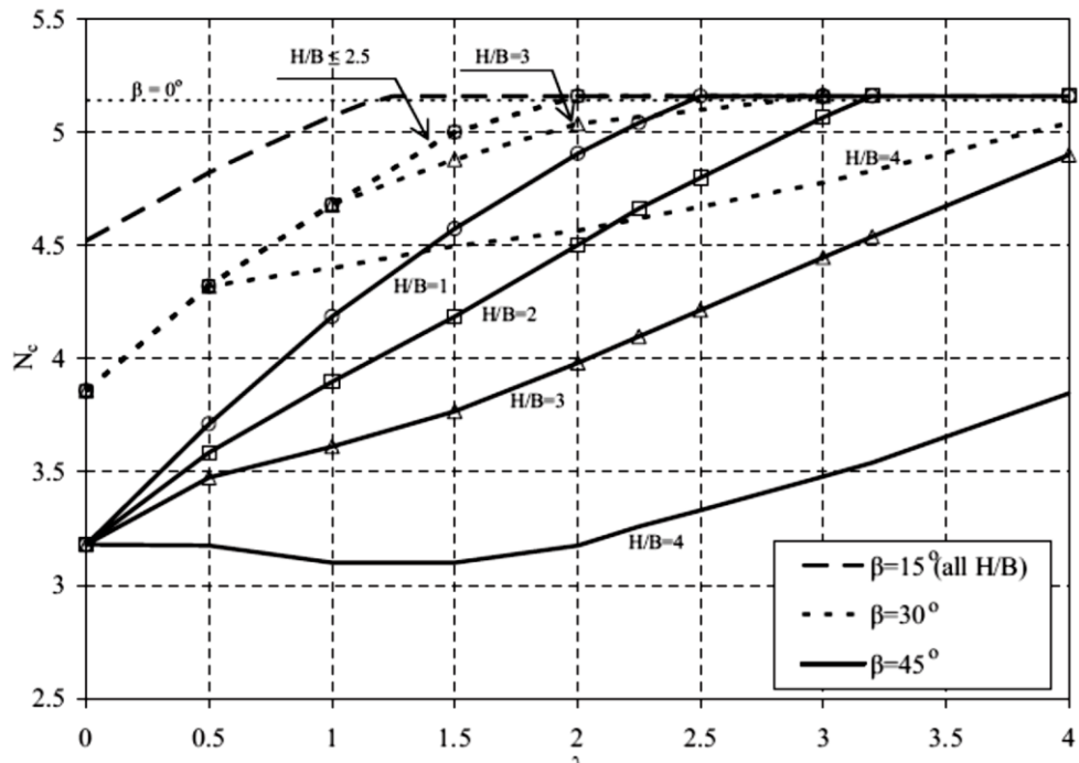
Figure 2.14. Variation of N_c with \lambda for c_u/\gamma B = 1 (Georgiadis, 2010).
