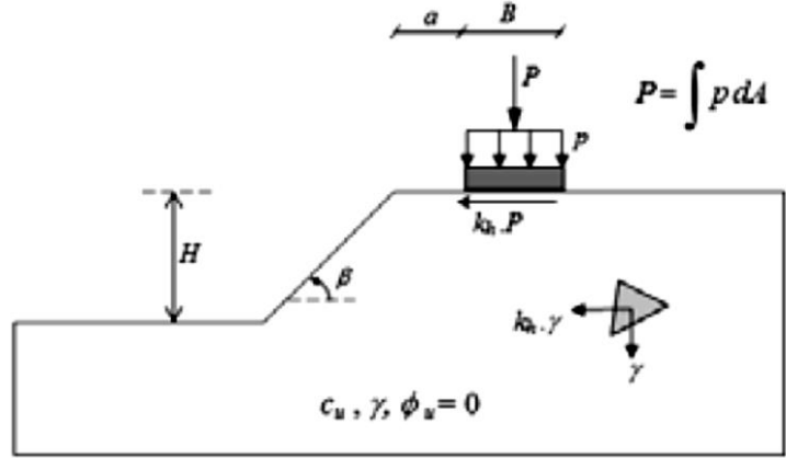
Figure 2.42. Problem parameters (Farzaneh et al. , 2013).
