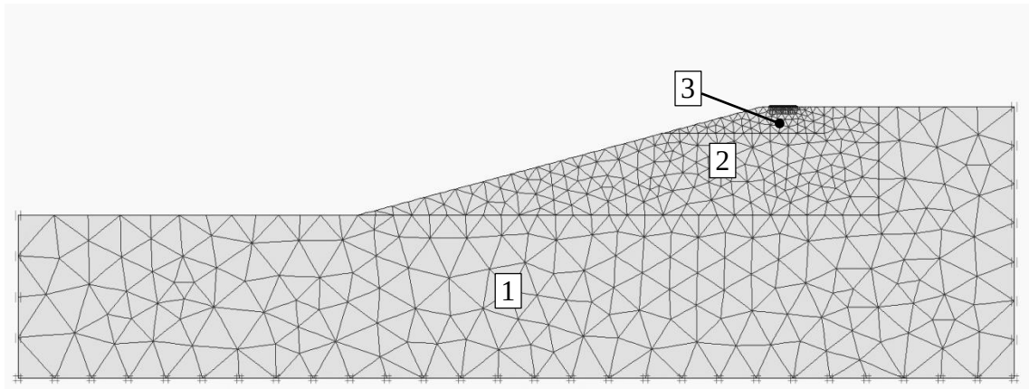
Figure 3.12. Typical connectivity plot obtained applying to developed mesh generation procedure ( \beta= 15^\circ , H= 8.0\text{m} ; \lambda= 0.25 ).
