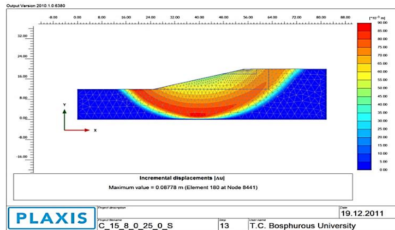
Figure 3.22. Failure mechanism of unstable cohesive slope in static condition ( \beta=15^\circ , H=8.0 m and c_u=25 kPa).
