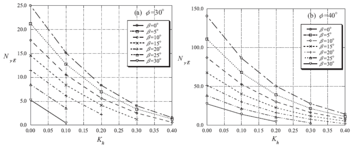
Figure 2.40. Design charts for N_{\gamma E} ( \Phi = 30^\circ, 40^\circ , D/B = 0 , a = 0.5 ) (Yamamoto, 2010).
