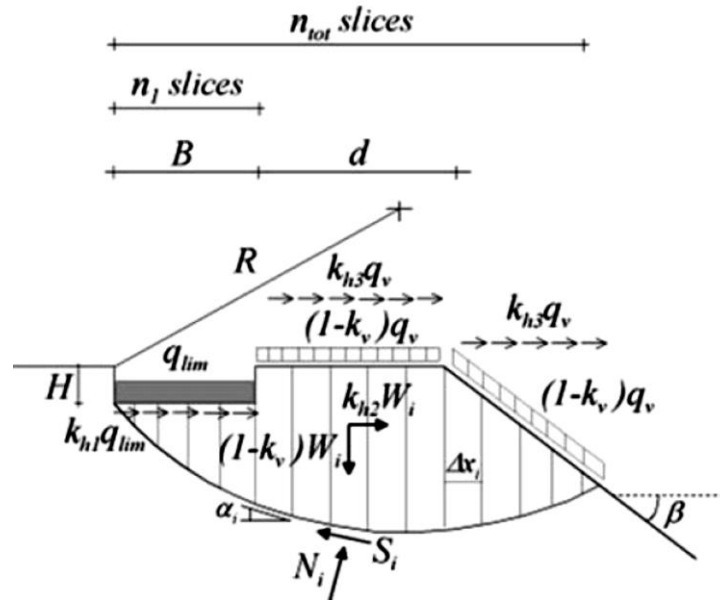
Figure 2.18. Failure mechanism and applied forces adopted in the analysis (Castelli and Motta, 2010).
