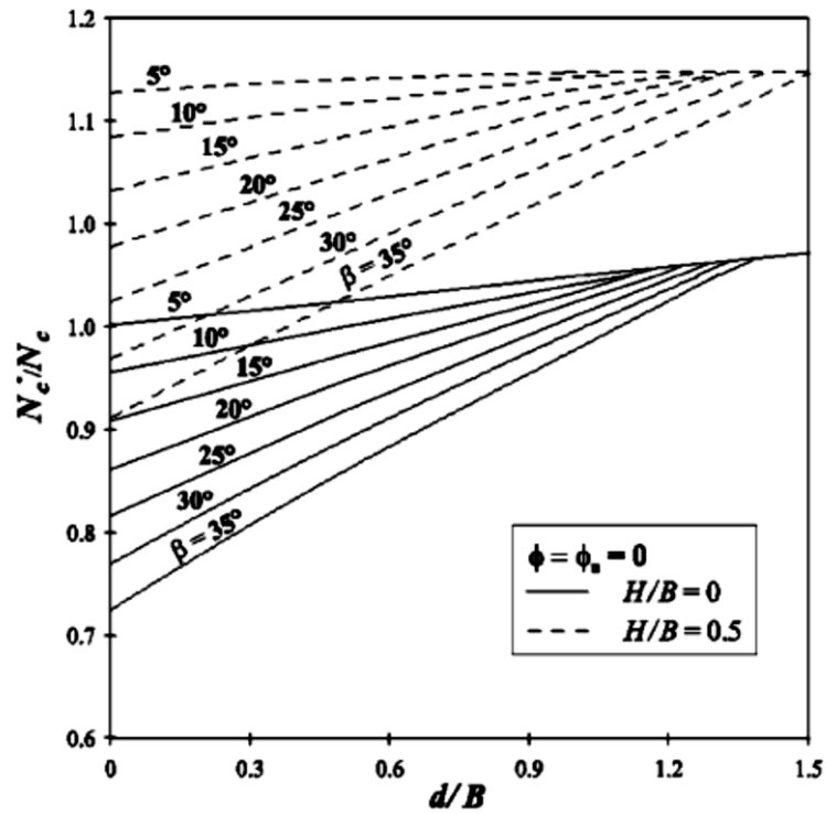
Figure 2.19. Variation of ground factors ( N_c^*/N_c ) in static condition with the footing distance from the edge of the slope (Castelli and Motta, 2010).
