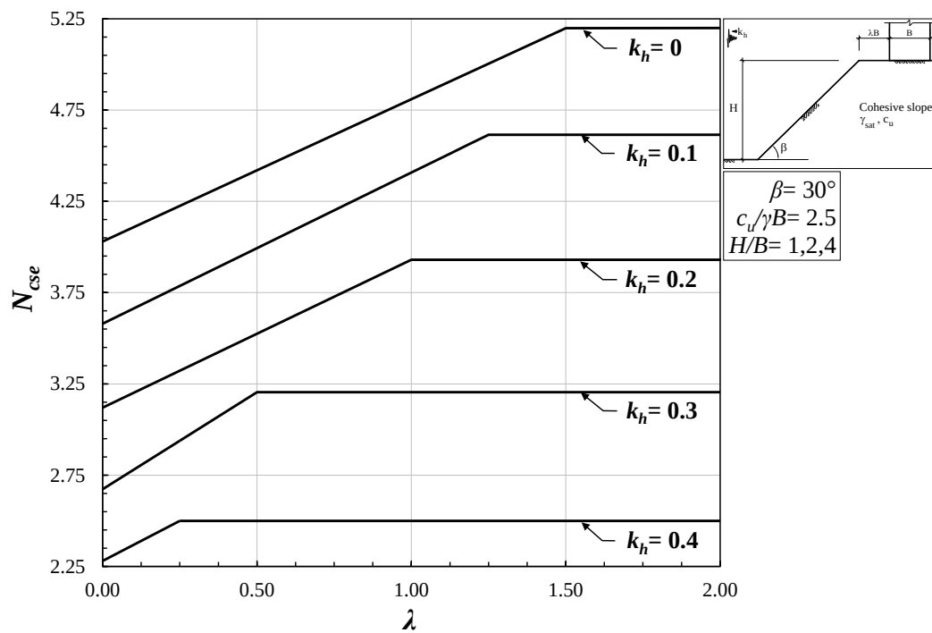
Figure 4.18. Design chart for seismic bearing capacity factor of surficial strip footings near cohesive slopes ( \beta = 30^\circ , c_u/\gamma B = 2.5 , H/B = 1, 2, 4 ).
