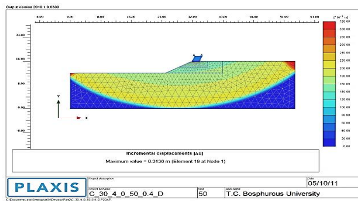
Figure 3.26. Failure mechanism of unstable cohesive slope in seismic condition ( \beta= 30^\circ , H= 4.0 m, c_u= 50 kPa, k_h= 0.4 ).
