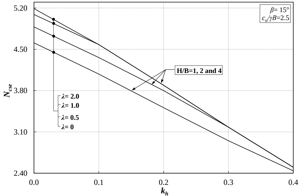
Figure 4.1. Variation of N_{cse} with k_h for all \lambda values ( \beta = 15^\circ , c_u/\gamma B = 2.5 ).
