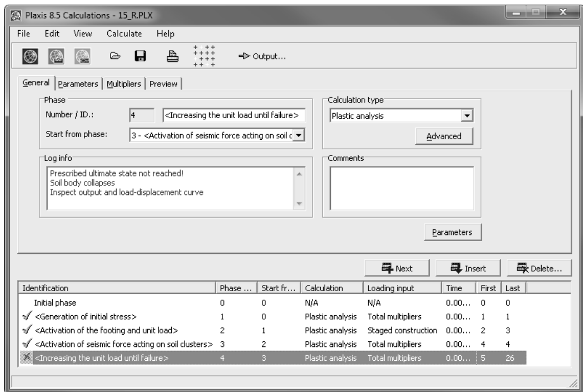
Figure 3.14. Typical view of “Calculations Module” window.
