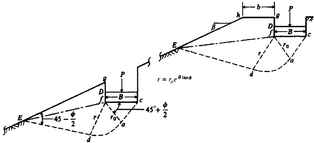
Figure 2.5. Footings on or adjacent to a slope (Bowles, 1997).
