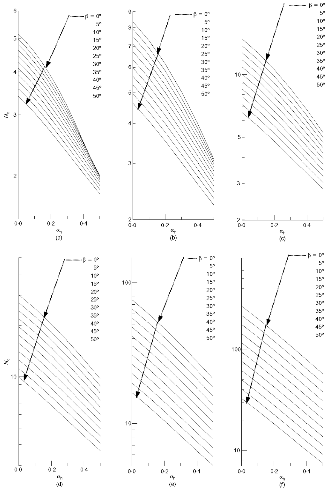
Figure 2.26. Variation of N_c with \alpha_h for different values of \Phi and \beta : (a) \Phi = 0^\circ ; (b) \Phi = 10^\circ ; (c) \Phi = 20^\circ ; (d) \Phi = 30^\circ ; (e) \Phi = 40^\circ ; (f) \Phi = 50^\circ (Kumar and Rao, 2003).
