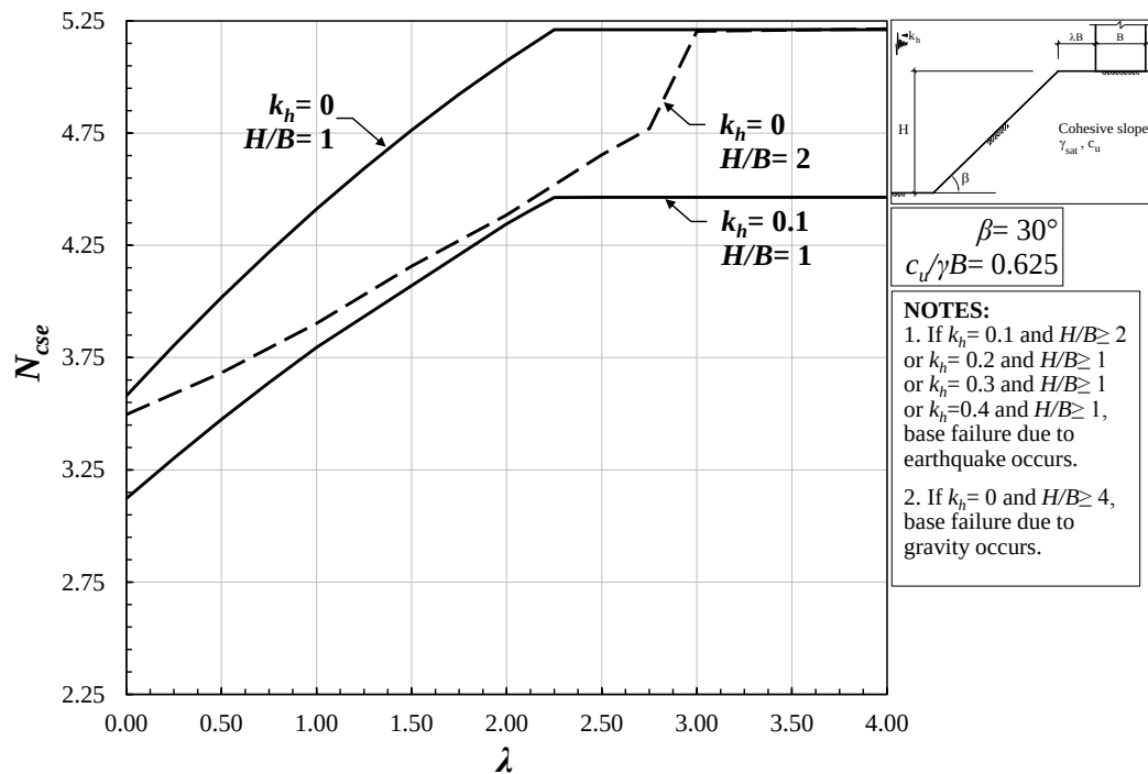
Figure 4.20. Design chart for seismic bearing capacity factor of surficial strip footings near cohesive slopes ( \beta = 30^\circ , c_u/\gamma B = 0.625 , H/B = 1, 2, 4 ).
