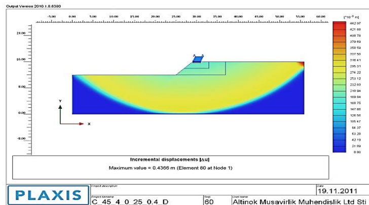
Figure 3.30. Failure mechanism of unstable cohesive slope in seismic condition ( \beta=45^\circ , H=4.0 m, c_u=25 kPa, k_h=0.4 ).
