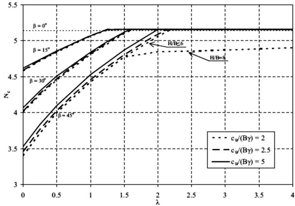
Figure 2.16. Variation of N_c with \lambda for c_u/\gamma B = 2, 2.5 and 5 (Georgiadis, 2010).
