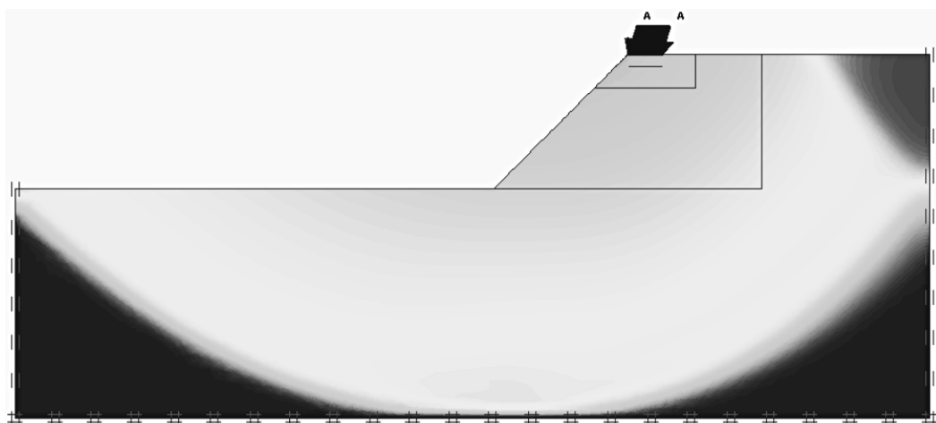
Figure 4.46. Failure mechanism obtained by Plaxis 2D for the design example 5.
