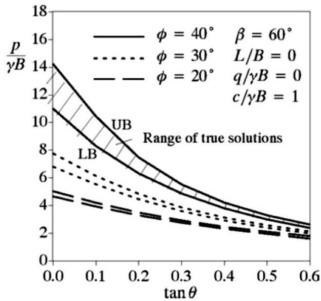
Figure 2.29. Effect of \tan\theta on p/\gamma B for various \Phi (Shiau et al. , 2006).
