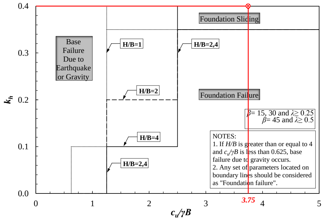
Figure 4.48. Estimation of the failure mode for the design example 6.
