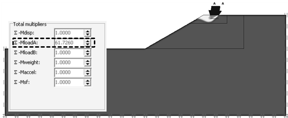
Figure 4.29. Load multiplier ( \Sigma -MloadA) and the failure mechanism obtained by Plaxis 2D for the design example 1.
