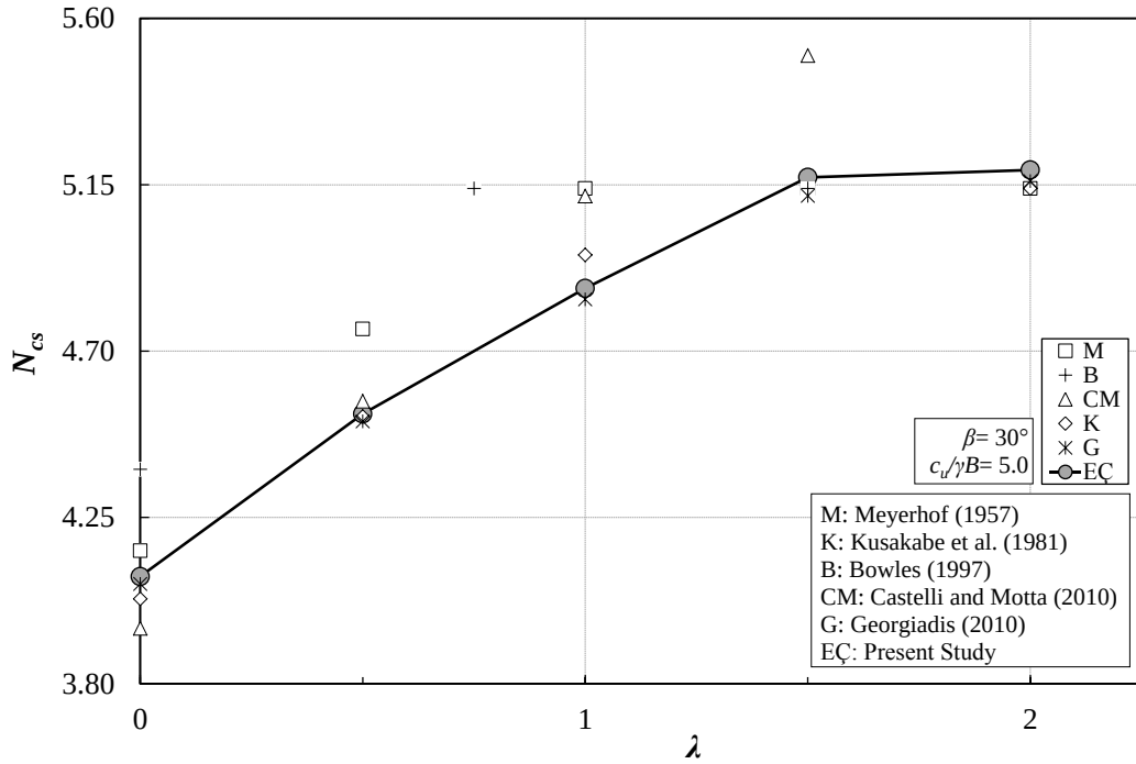
Figure 3.19. Variation of N_{cs} with \lambda (For \beta=30^\circ , c_u/\gamma B=5 ).
