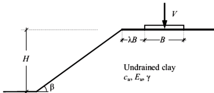
Figure 2.10. Schematic representation of the problem (Georgiadis, 2010).
