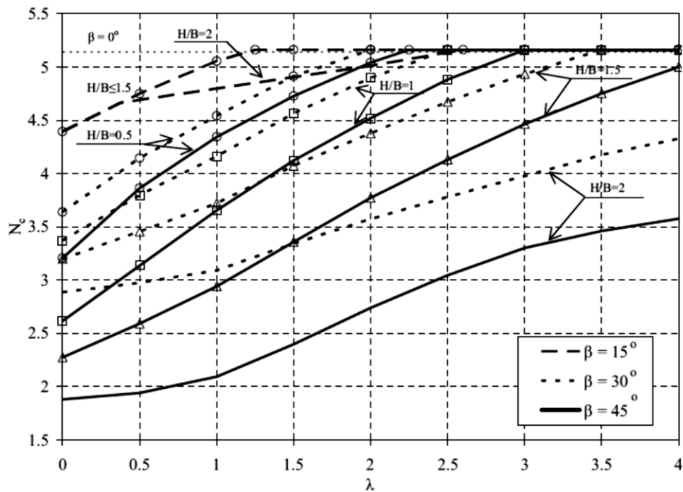
Figure 2.13. Variation of N_c with \lambda for c_u/\gamma B = 0.5 (Georgiadis, 2010).
