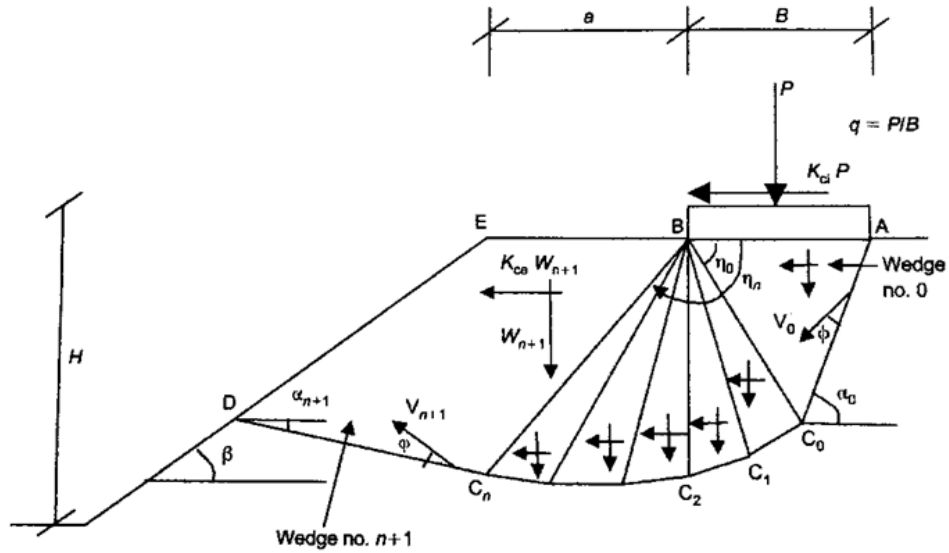
Figure 2.22. Failure mechanism used in the analysis (Askari and Farzaneh, 2003).
