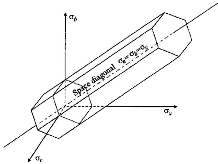
Figure 3.7. Tresca yield surface in principal total stress space (Potts and Zdravkovic, 1999).
