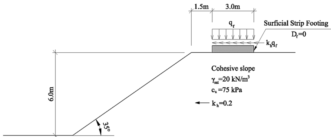
Figure 4.30. Schematic representation of the design example 2.
