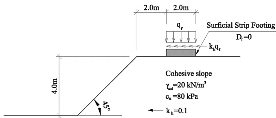
Figure 4.35. Schematic representation of the design example 3.
