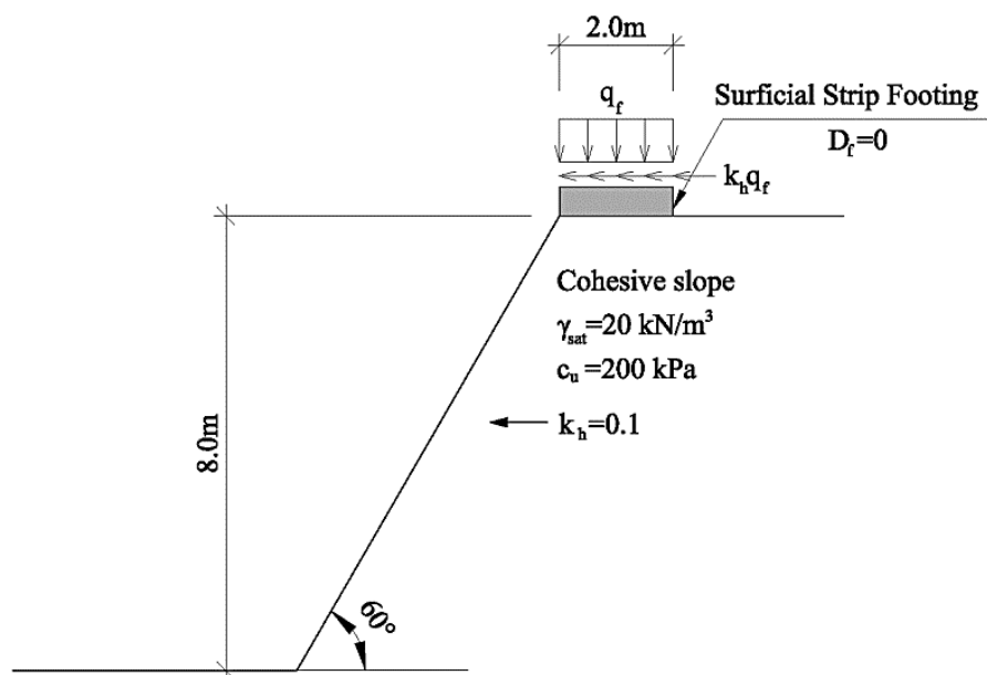
Figure 4.40. Schematic representation of the design example 4.
