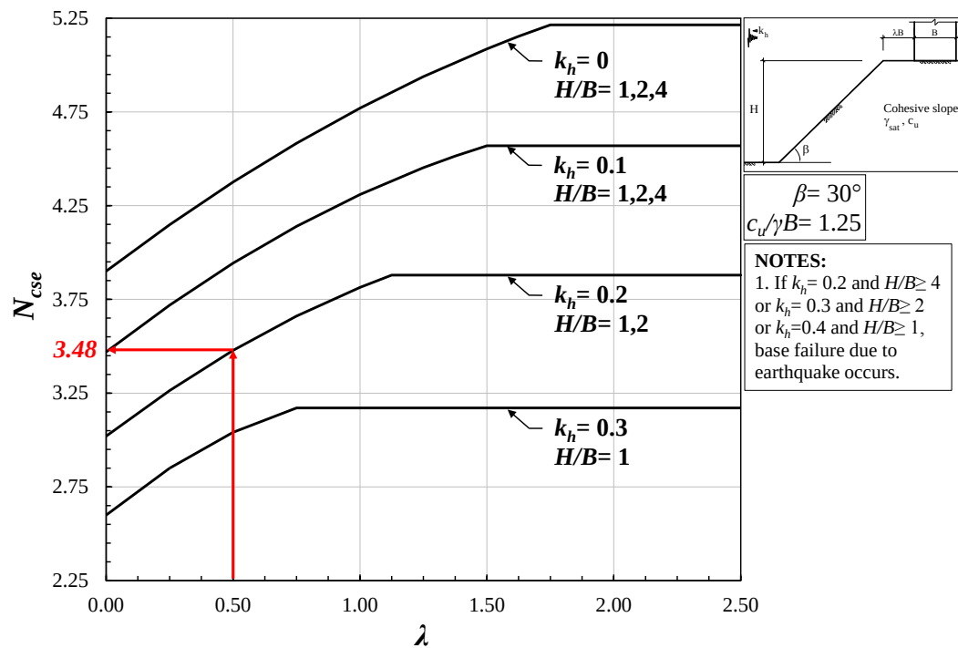
Figure 4.32. The first N_{cse} value to be used in linear interpolation for the design example 2.
