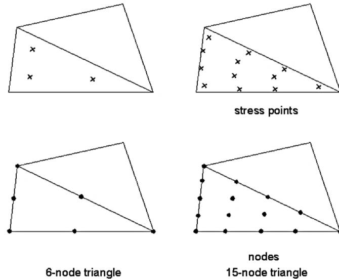
Figure 3.4. Position of nodes and stress points in soil elements (Brinkgreve et al. , 2006).
