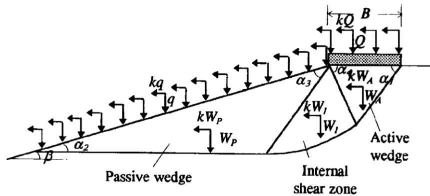
Figure 2.21. Failure mechanism and applied forces of foundation-soil system (Sarma and Chen, 1996).
