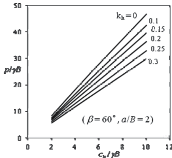
Figure 2.44. Variation of seismic bearing capacity c_u/\gamma B (Farzaneh et al. , 2013).
