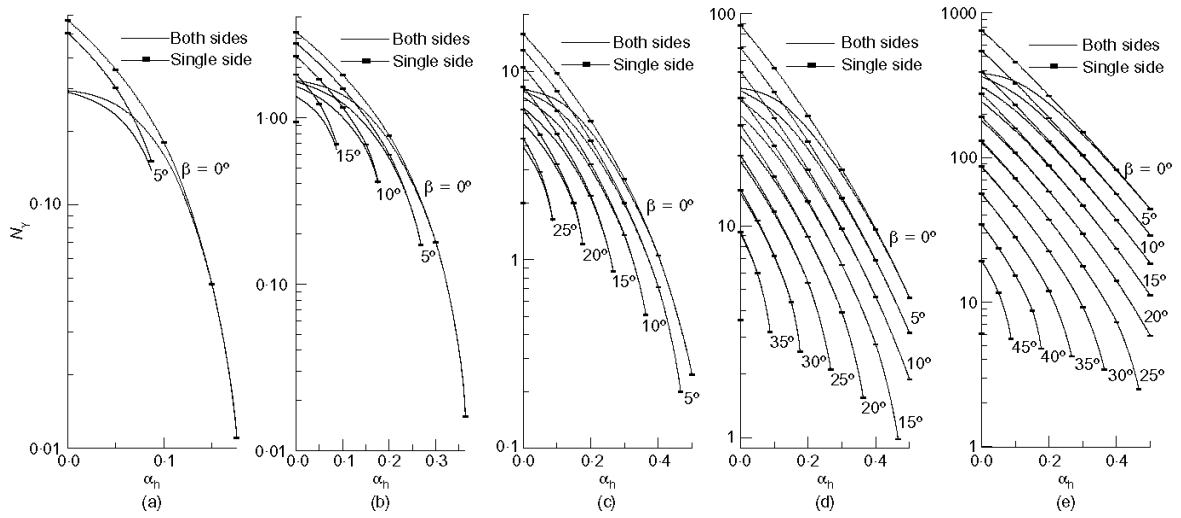
Figure 2.27. Variation of N_\gamma with \alpha_h for different values of \Phi and \beta : (a) \Phi = 10^\circ ; (b) \Phi = 20^\circ ; (c) \Phi = 30^\circ ; (d) \Phi = 40^\circ ; (e) \Phi = 50^\circ (Kumar and Rao, 2003)
