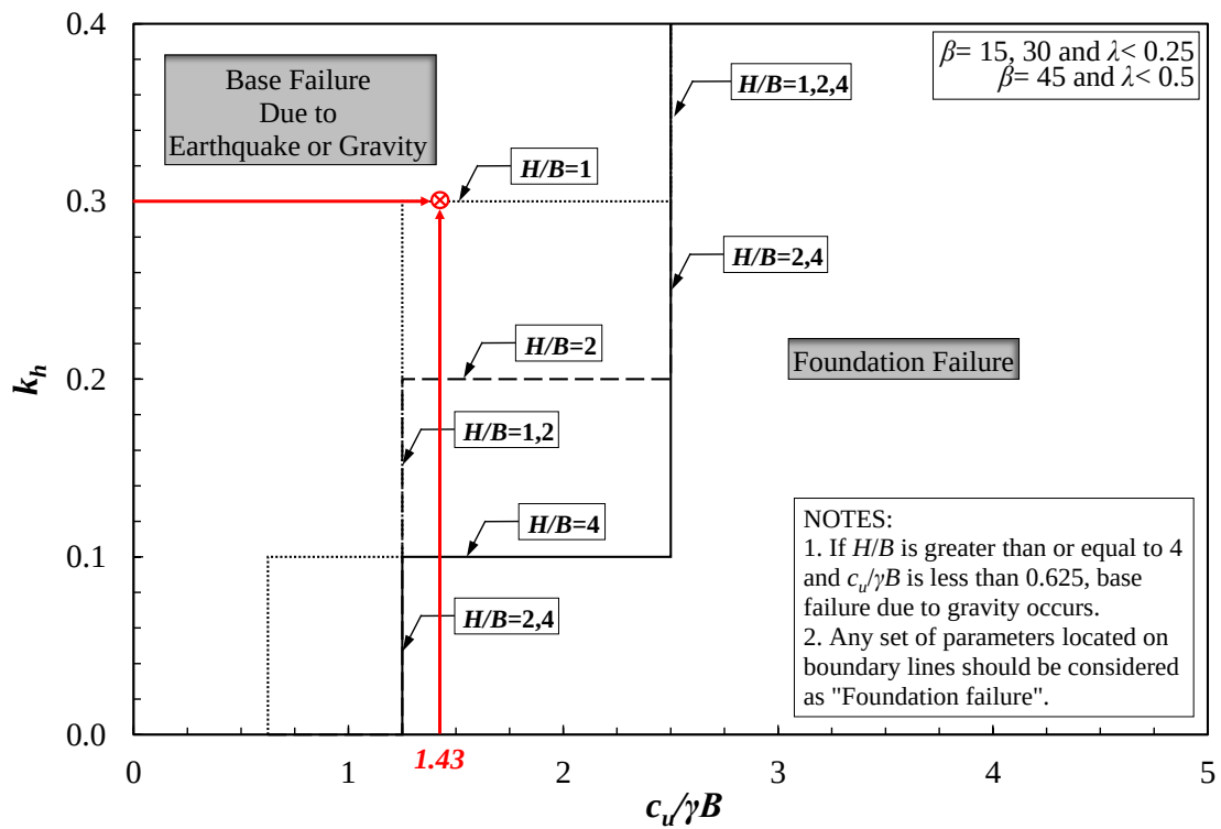
Figure 4.44. Estimation of the failure mode for the design example 5.
