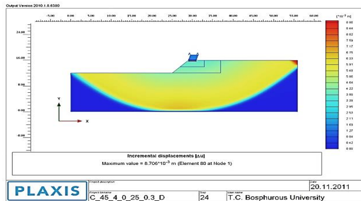
Figure 3.29. Failure mechanism of unstable cohesive slope in seismic condition ( \beta=45^\circ , H=4.0 m, c_u=25 kPa, k_h=0.3 ).
