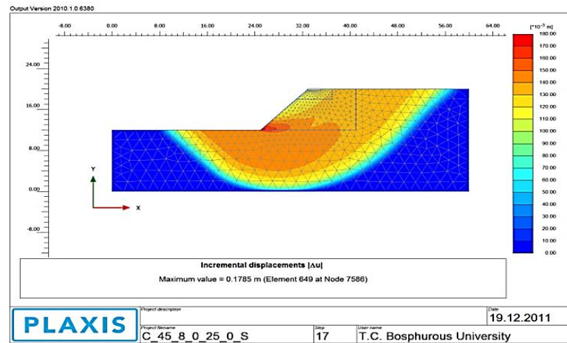
Figure 3.24. Failure mechanism of unstable cohesive slope in static condition ( \beta = 45^\circ , H = 8.0 m and c_u = 25 kPa).
