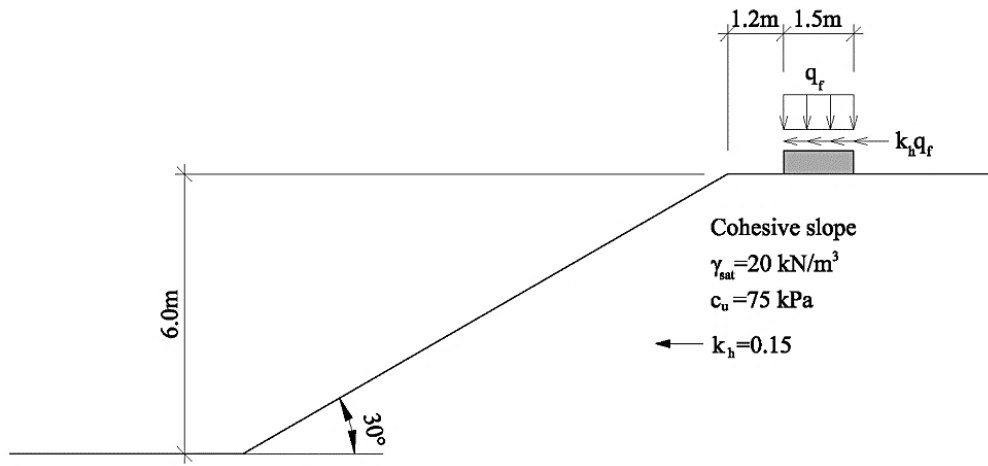
Figure 4.26. Schematic representation of the design example 1.
