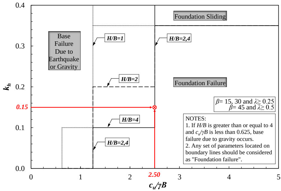
Figure 4.27. Estimation of the failure mode for the design example 1.
