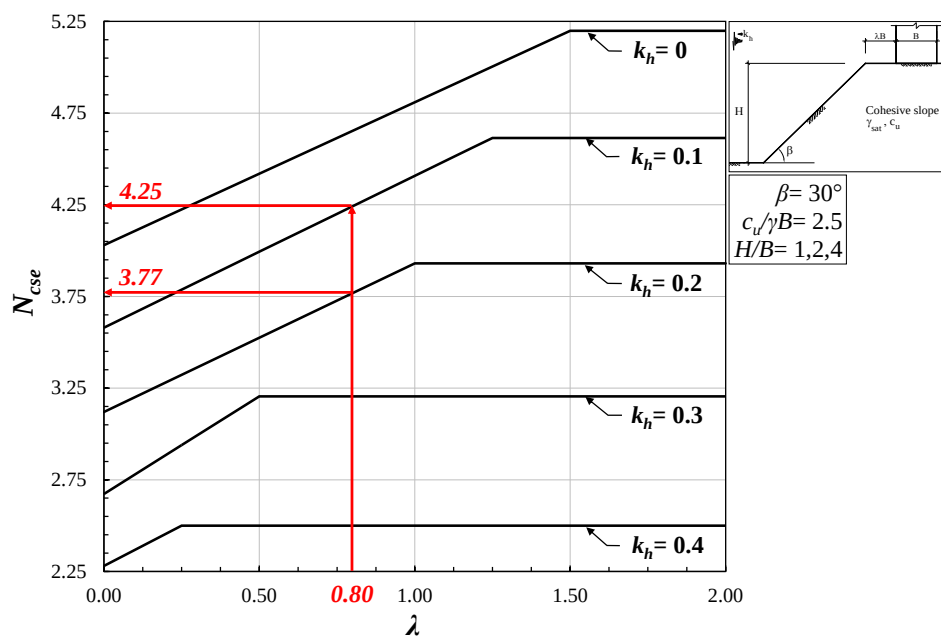
Figure 4.28. N_{cse} values to be used in linear interpolation for the design example 1.
