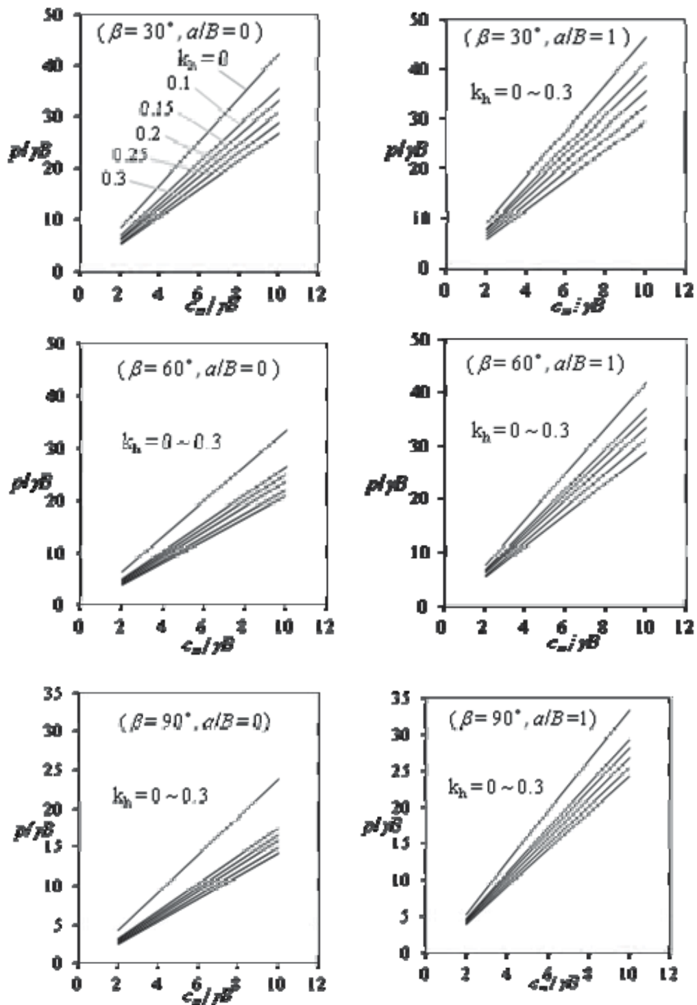
Figure 2.45. Design charts for seismic bearing capacity of strip footings near cohesive slopes (Farzaneh et al. , 2013).
