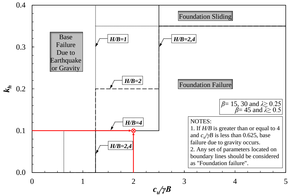
Figure 4.36. Estimation of the failure mode for the design example 3.
