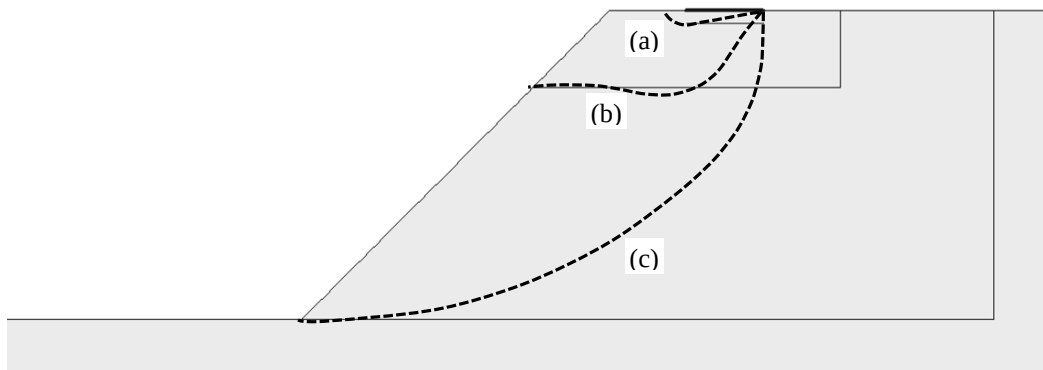
Figure 4.8. Typical "Foundation failure" modes for \lambda > 0 condition (a) \beta = 45^\circ , H/B = 4 , c_u/\gamma B = 2.5 , k_h = 0.3 ; (b) \beta = 45^\circ , H/B = 4 , c_u/\gamma B = 2.5 , k_h = 0.1 ; (c) \beta = 45^\circ , H/B = 4 , c_u/\gamma B = 1.25 , k_h = 0.1 .
