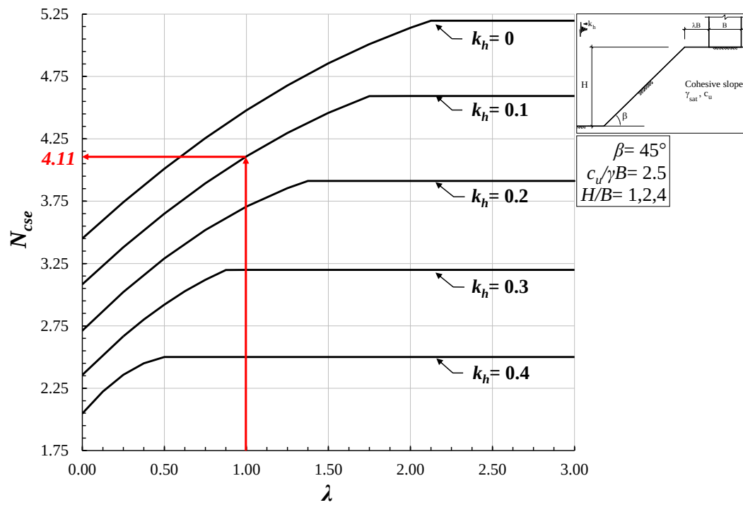
Figure 4.37. The first N_{cse} value to be used in linear interpolation for the design example 3.
