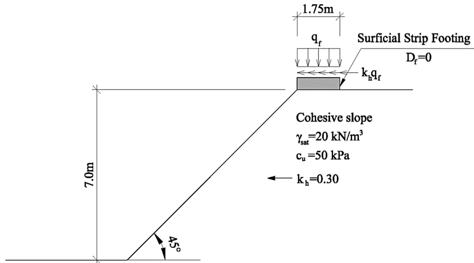
Figure 4.43. Schematic representation of the design example 5.
