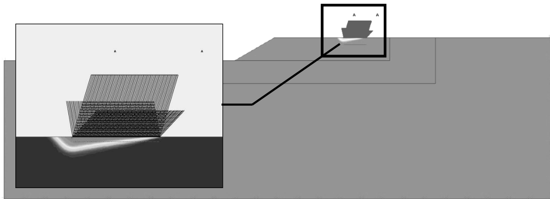
Figure 3.16. Failure mechanism obtained for the finite element model named as C_30_2_3_200_0.3_D and enlarged view of the failure mechanism.
