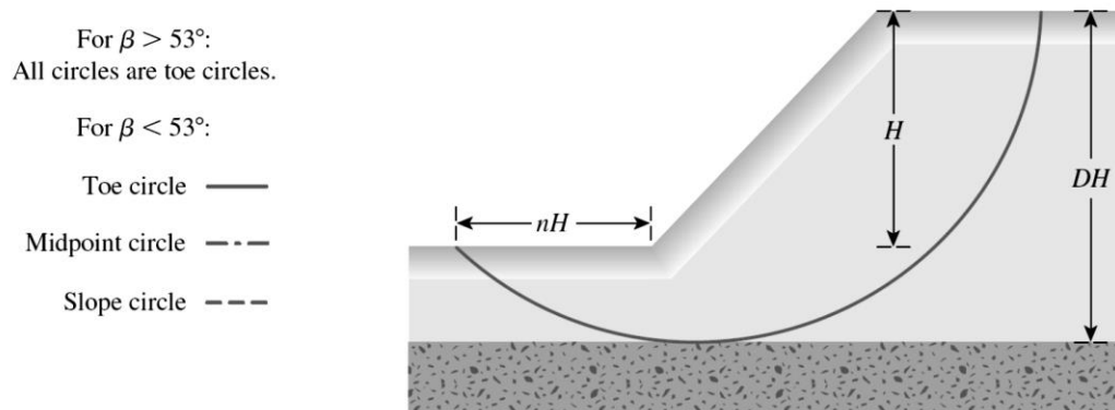
Figure 2.46. Definition of parameters for midpoint circle type of failure (Taylor, 1937) (Adapted from Das, 2009).
