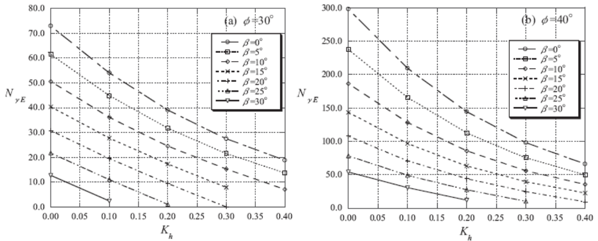
Figure 2.39. Design charts for N_{\gamma E} ( \Phi = 30^\circ, 40^\circ , D/B = 1 , a = 0.0 ) (Yamamoto, 2010).
