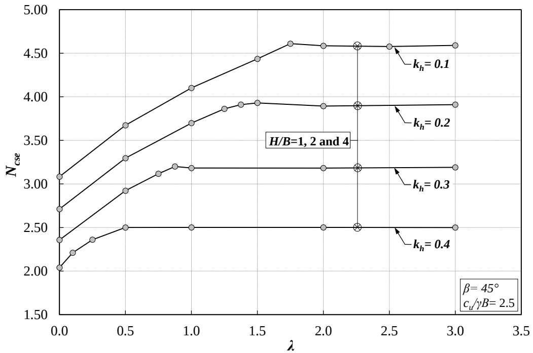
Figure 4.3. Variation of N_{cse} with \lambda for all k_h values ( \beta = 45^\circ , c_u/\gamma B = 2.5 ).
