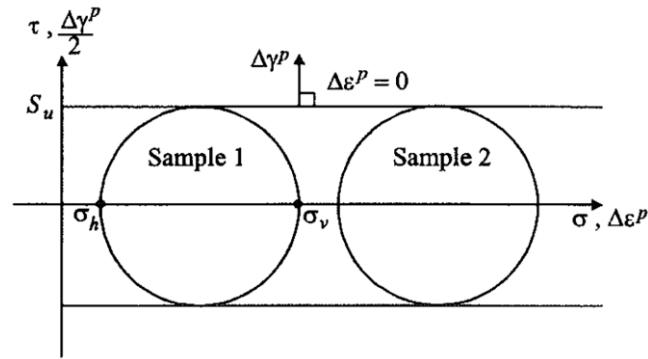
Figure 3.8. Mohr's circles of total stress (Potts and Zdravkovic, 1999).
