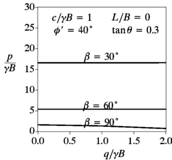
Figure 2.31. Effect of q/\gamma B on p/\gamma B for various \beta (Shiau et al. , 2006).
