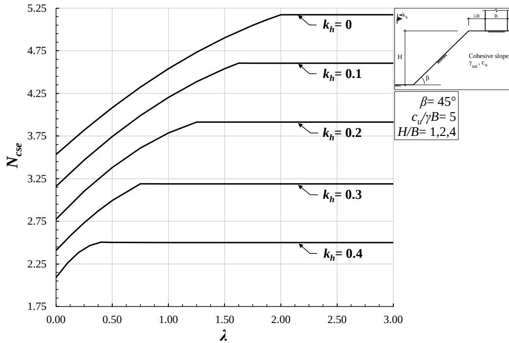
Figure 4.21. Design chart for seismic bearing capacity factor of surficial strip footings near cohesive slopes ( \beta = 45^\circ , c_u/\gamma B = 5 , H/B = 1, 2, 4 ).
