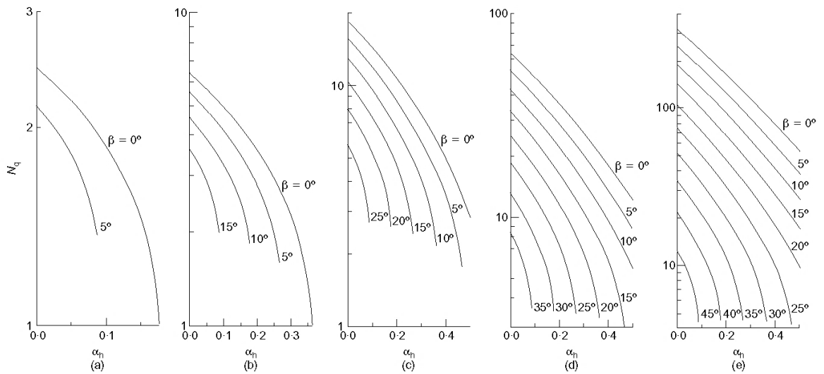
Figure 2.25. Variation of N_q with \alpha_h for different values of \Phi and \beta : (a) \Phi = 10^\circ ; (b) \Phi = 20^\circ ; (c) \Phi = 30^\circ ; (d) \Phi = 40^\circ ; (e) \Phi = 50^\circ (Kumar and Rao, 2003).
