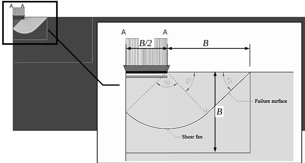
Figure 3.10. Failure mechanism determined by Plaxis 2D at the ultimate state and its enlarged view.
