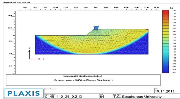
Figure 3.28. Failure mechanism of unstable cohesive slope in seismic condition ( \beta=45^\circ , H=4.0 m, c_u=25 kPa, k_h=0.2 ).
