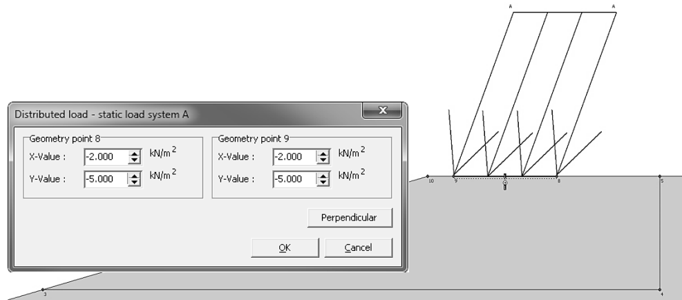
Figure 3.6. Inclined load acting on the rigid footing and unit load definition (For k_h = 0.4 )
