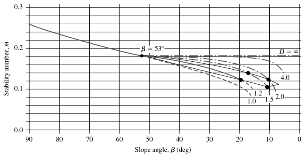
Figure 2.47. Plot of stability number ( m ) against slope angle ( \beta ) (Taylor, 1937) (Adapted from Das, 2009).
