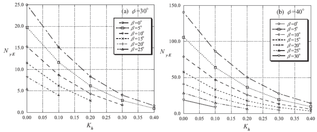
Figure 2.38. Design charts for N_{ye} ( \Phi = 30^\circ, 40^\circ, D/B = 0, a = 0.0 ) (Yamamoto, 2010).
