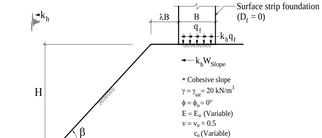
Figure 3.1. Graphical representation of the problem.
