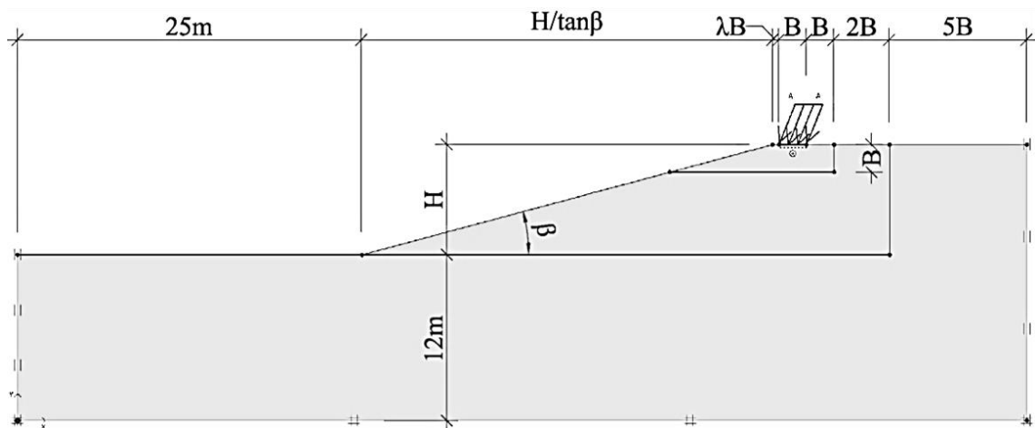
Figure 3.5. Schematic representation of created finite elements model.
