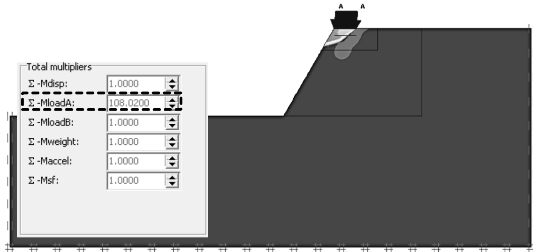
Figure 4.42. Load multiplier ( \Sigma\text{-MloadA} ) and the failure mechanism obtained by Plaxis 2D for the design example 4.
