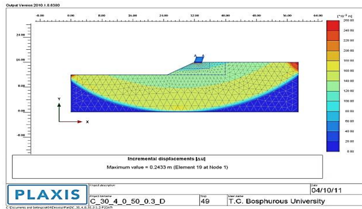
Figure 3.25. Failure mechanism of unstable cohesive slope in seismic condition ( \beta= 30^\circ , H= 4.0 m, c_u= 50 kPa, k_h= 0.3 ).
