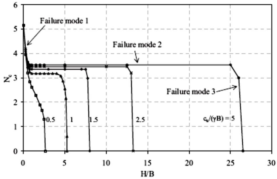
Figure 2.12. Variation of failure mode and N_c with H/B for \lambda = 0 and \beta = 45^\circ (Georgiadis, 2010).
