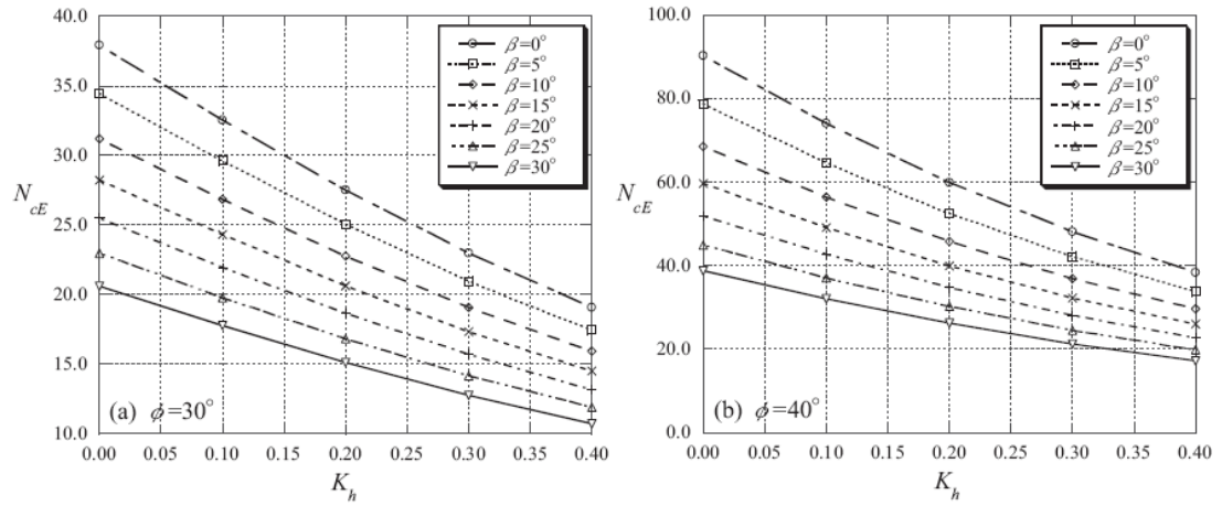
Figure 2.36. Design charts for N_{ce} ( \Phi = 30^\circ, 40^\circ, D/B = 1, a = 0.0 ) (Yamamoto, 2010).
