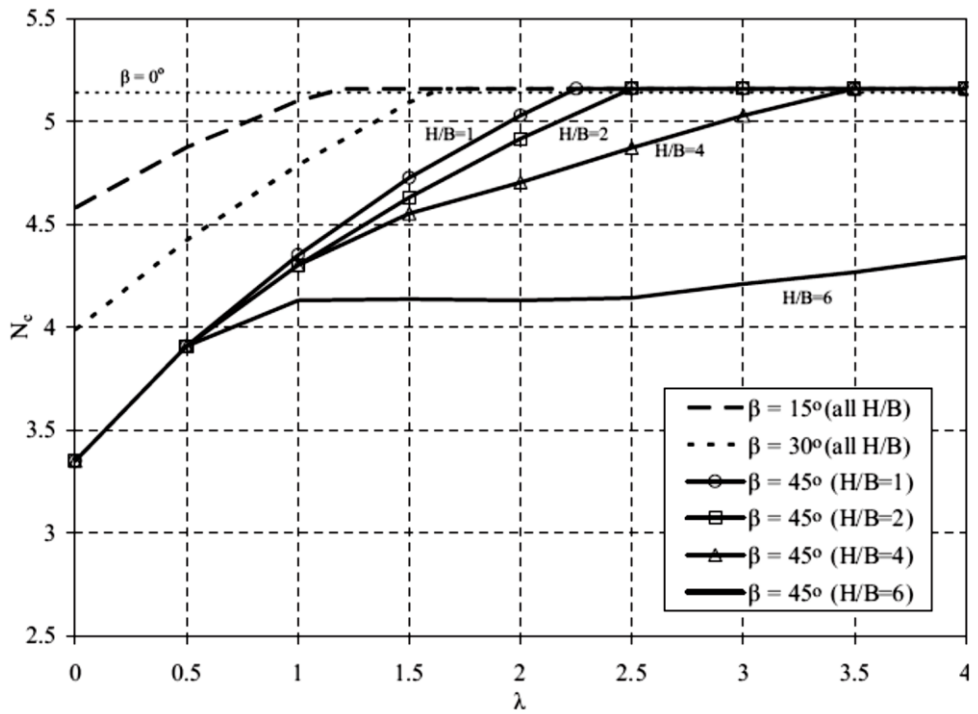
Figure 2.15. Variation of N_c with \lambda for c_u/\gamma B = 1.5 (Georgiadis, 2010).
