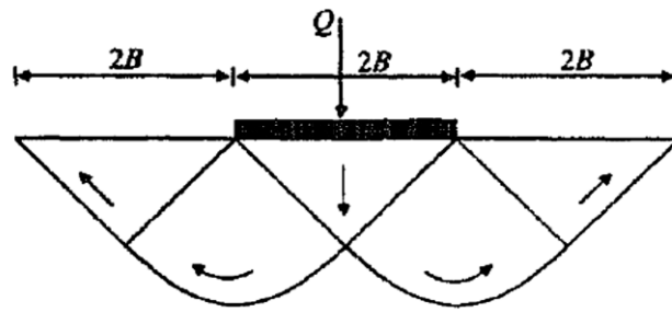
Figure 3.9. Prandtl type failure mechanism (Prandtl, 1920) (Adapted from Potts and Zdravkovic, 2001).
