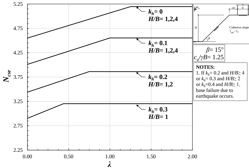
Figure 4.15. Design chart for seismic bearing capacity factor of surficial strip footings near cohesive slopes ( \beta = 15^\circ , c_u/\gamma B = 1.25 , H/B = 1, 2, 4 ).
