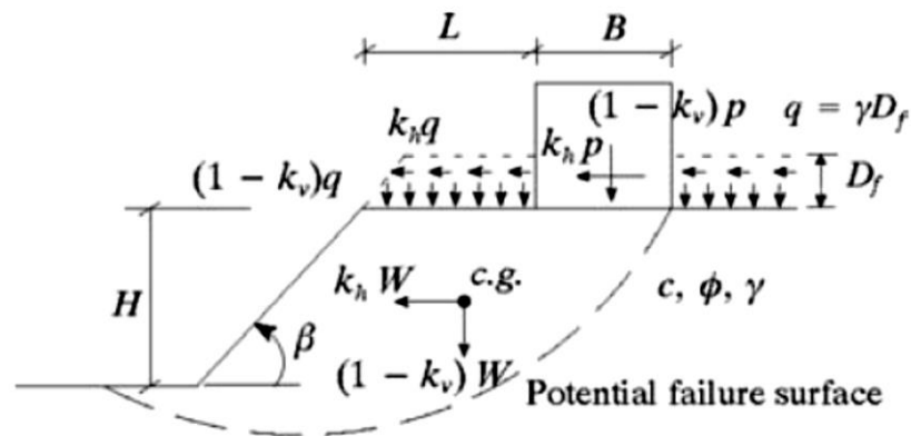
Figure 2.28. Graphical representation of the problem (Shiau et al. , 2006).
