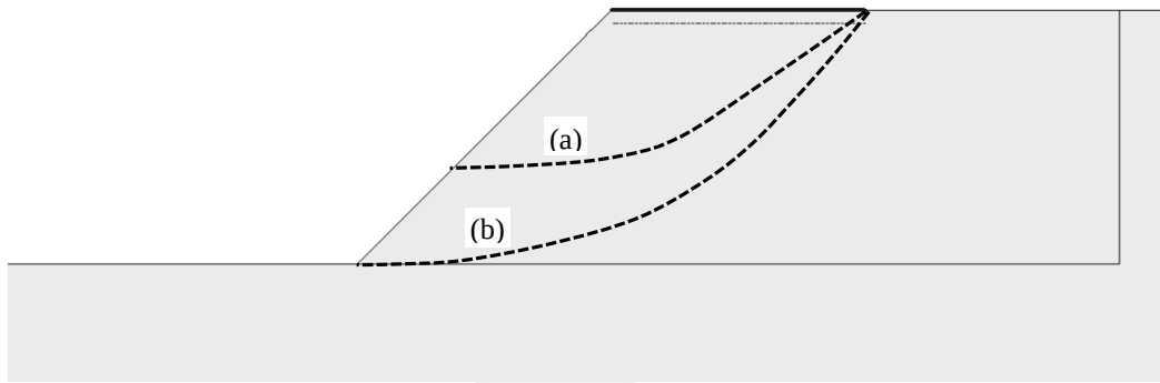
Figure 4.7. Typical "Foundation failure" modes for \lambda = 0 condition (a) \beta = 45^\circ , H/B = 1 , c_u/\gamma B = 1.25 , k_h = 0.2 ; (b) \beta = 45^\circ , H/B = 1 , c_u/\gamma B = 0.625 , k_h = 0.1 .
