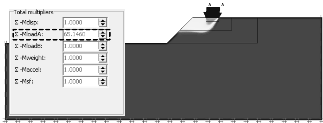
Figure 4.39. Load multiplier ( \Sigma -MloadA) and the failure mechanism obtained by Plaxis 2D for the design example 3.
