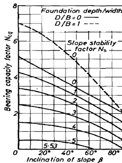
Figure 2.2. Bearing capacity factors for strip foundation on face of a purely cohesive slope (Meyerhof, 1957).
