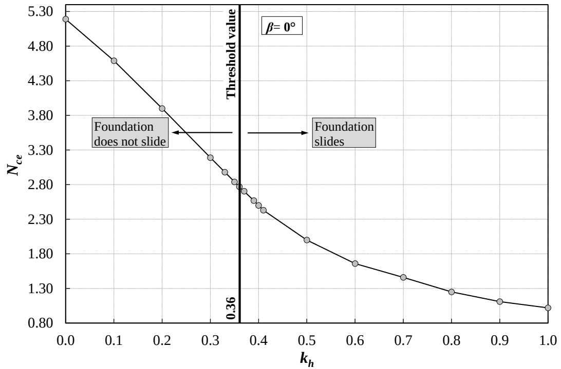
Figure 4.10. Variation of N_{ce} with k_h ( \beta = 0^\circ ).
