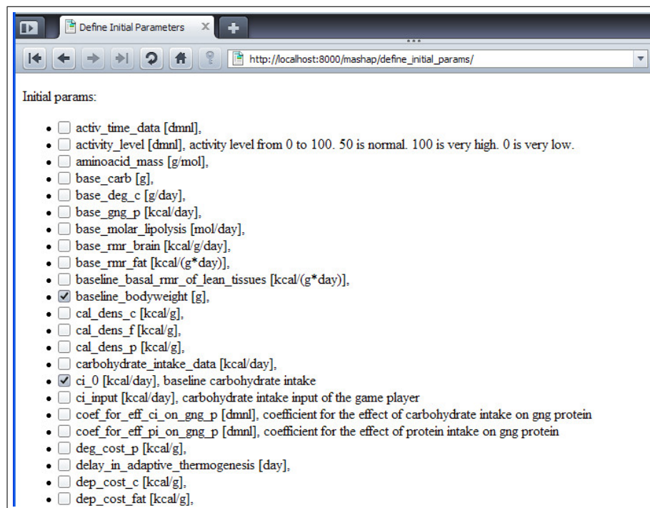
Figure 7.3. Initial Parameters Definition Screen
