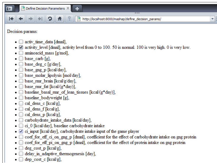
Figure 7.5. Decision Variables Definition Screen
