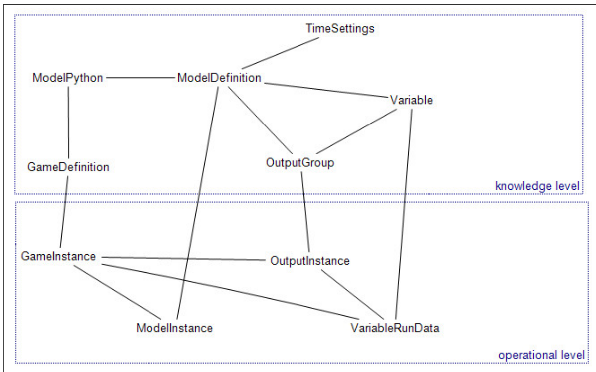
Figure 5.1. Domain model of the Mashap software
