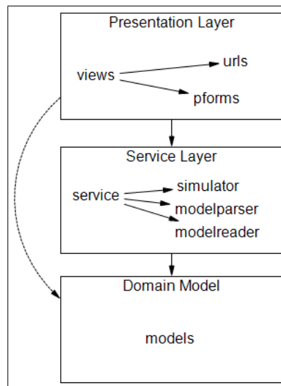
Figure 5.2. Layers of the system architecture of Mashap
