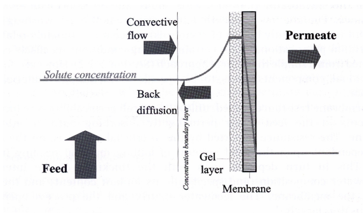
Figure 2.7. Concentration polarization (Judd and Jefferson, 2003).
