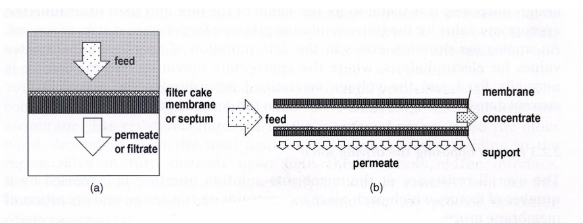
Figure 2.5. (a) Dead-end filtration and (b) cross-flow filtration (Judd and Jefferson, 2003).
