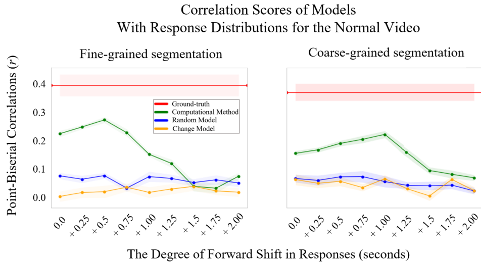
Figure 9 Time-dependent correlations of computational models
