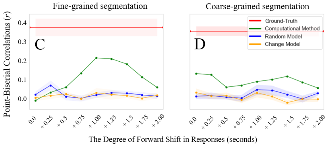
Figure 12 The performance of the model in noisy video segmentation
