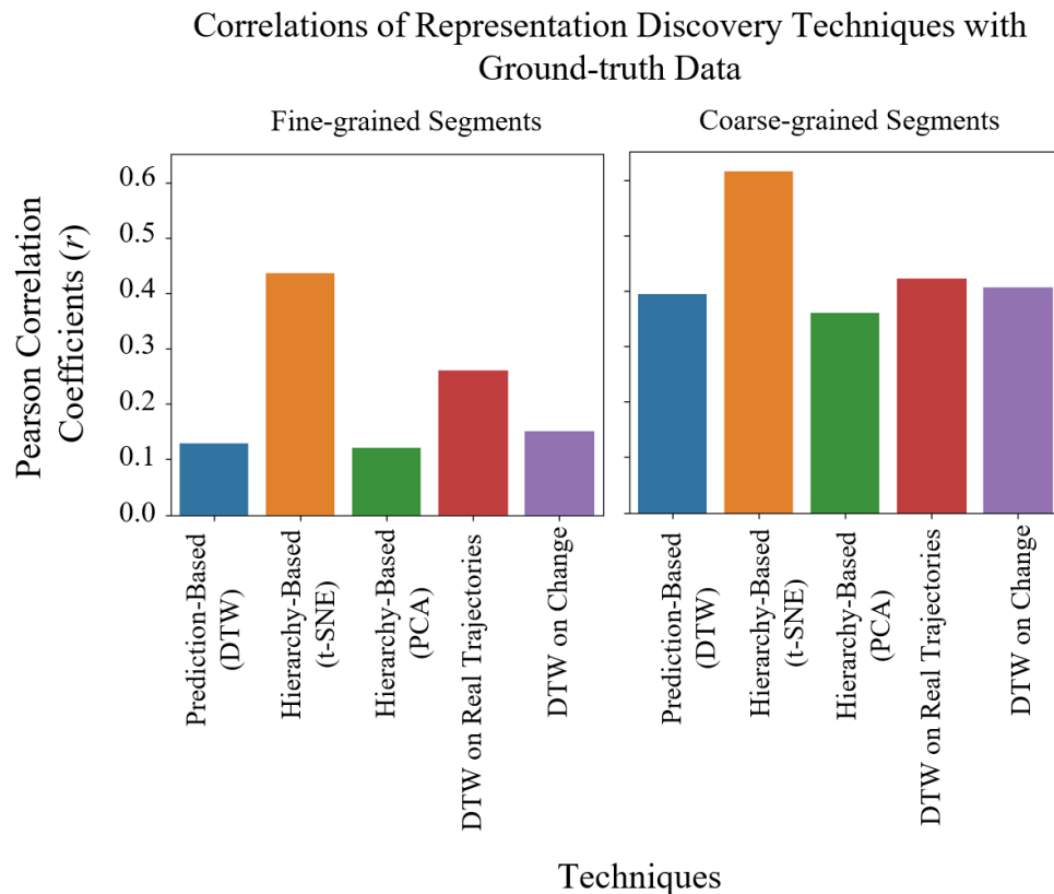
Figure 16 Correlations of representation discovery techniques and baselines
