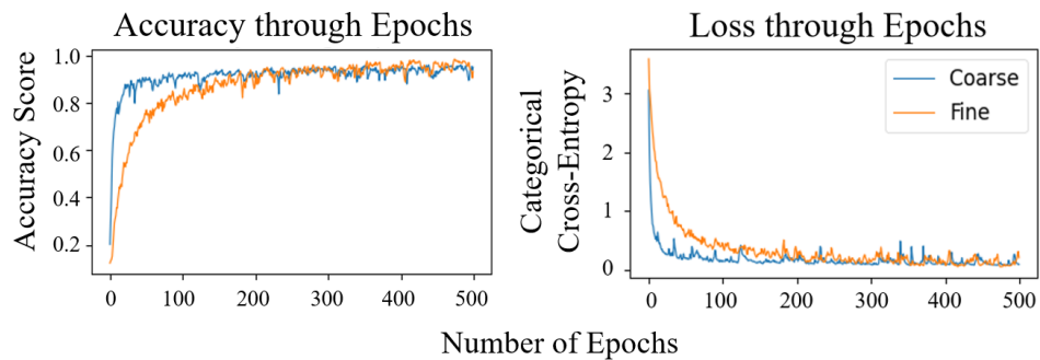
Figure 13 Accuracy scores and losses of hierarchical models
