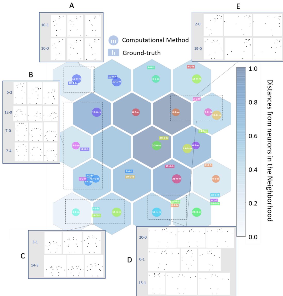
Figure 17 SOM results for fine-grained event representations
