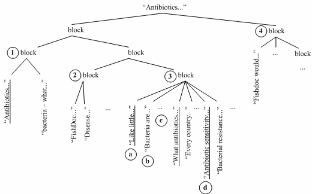
Figure 4.3. The document tree obtained after DOM tree processing
