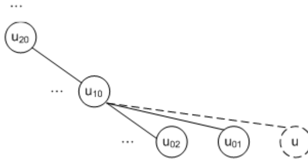
Figure 5.6. Contextual information in document sectional hierarchy
