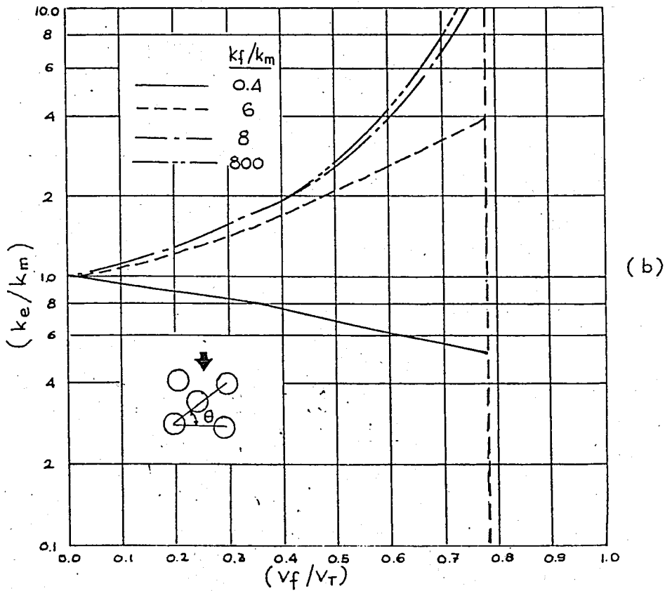
FIGURE 2.18 - Effective conductivities for staggered array fiber composite ( \theta = 45 deg.) a) Homogeneous Method b) Flux Method
