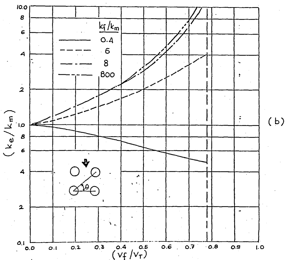
FIGURE 2.9 - Effective conductivities for rectangular array fiber composite ( \theta = 45 deg.)
