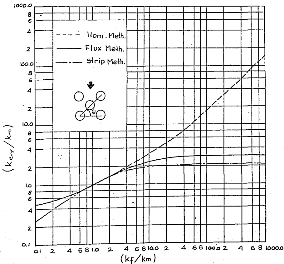
FIGURE 2.12 - Effective conductivities for staggered array fiber composite ( v_f/v_T = 0.5 , \theta = 35 deg.)
