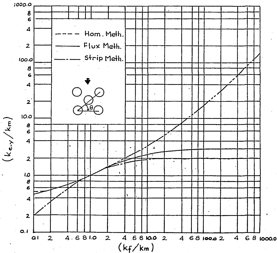
FIGURE 2.13 - Effective conductivities for staggered array fiber composite ( v_f/v_T = 0.5 , \theta = 40^\circ .)
