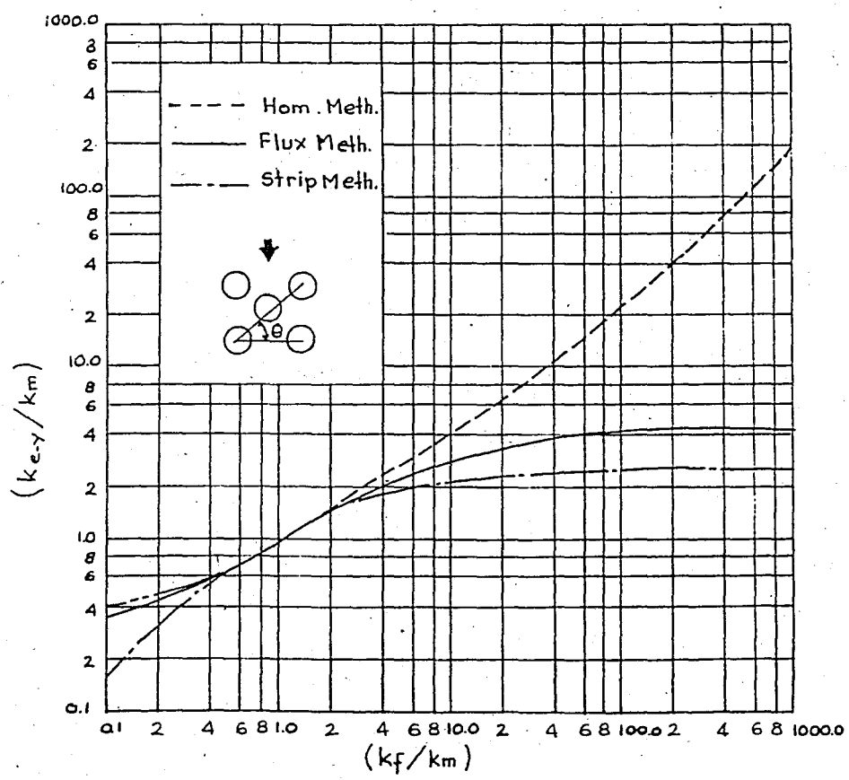
FIGURE 2.14 - Effective conductivities for staggered array fiber composite ( v_f/v_T = 0.6 , \theta = 40^\circ ).
