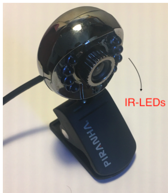
Figure 2.13 Webcam with IR-LEDs that is used to capture eye blinks.
