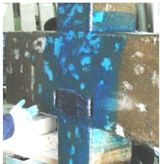
Figure 3.11. Application of belts
