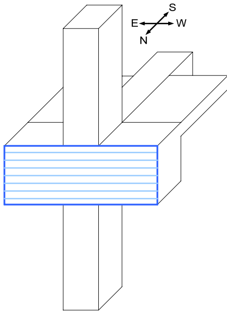
Figure 3.13. Application of CFRP on backside of the specimen
