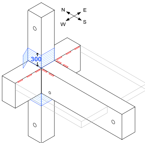
Figure 3.14. Application of column wraps
