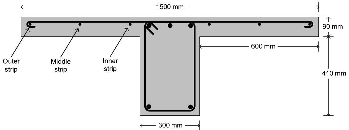
Figure 4.53. Distribution of slab reinforcement and their labels
