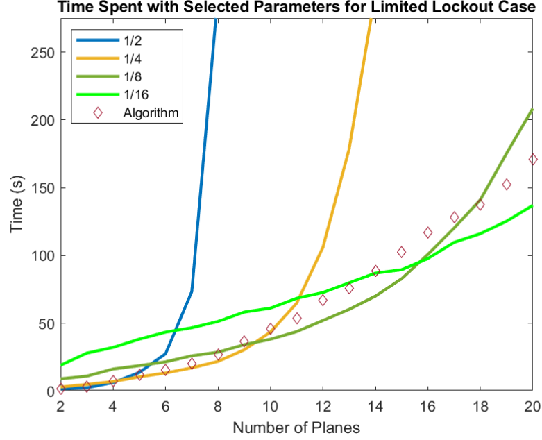
Figure 3.7. The performance of the algorithm and static methods for limited lockout case with PRF: 150\text{ Hz} , BW: 2.4^\circ , and RPM: 6\text{ min}^{-1} .
