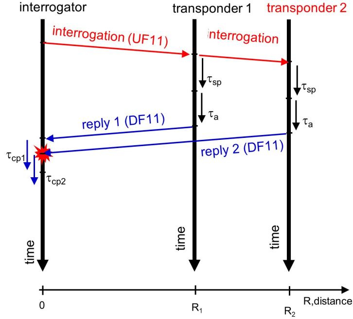
Figure 2.6. Time-flow chart for two transponders flying close to each other in succession.
