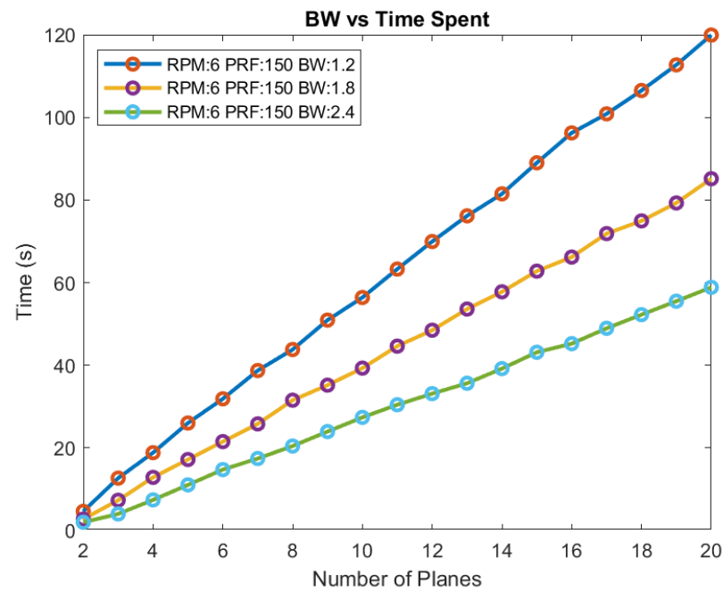
Figure 3.3. Effect of beam-width on the performance of the Adaptive Algorithm.
