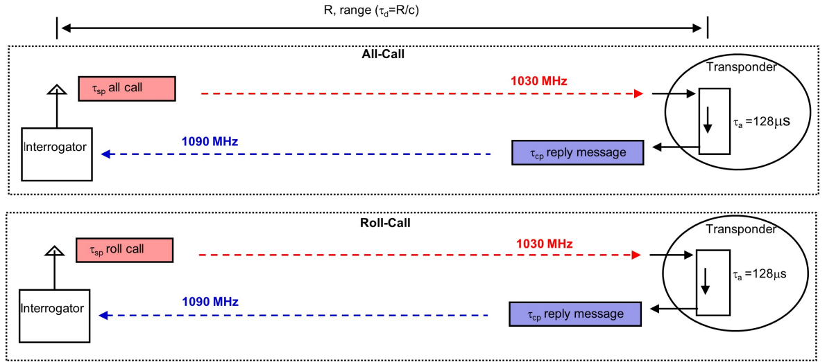
Figure 2.4. All-call and roll-call interrogation illustration.
