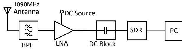
Figure 2.13. Connection scheme.
