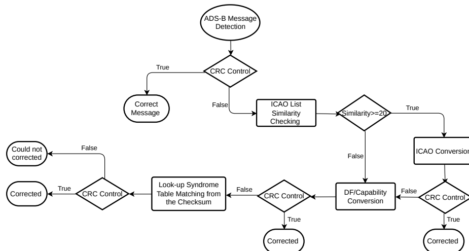
Figure 2.17. The flow diagram of the second method for error correction.
