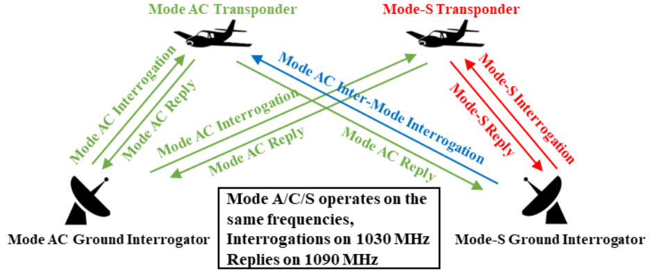
Figure 1.1. Mode-S and Mode A/C interrogations and replies [4].
