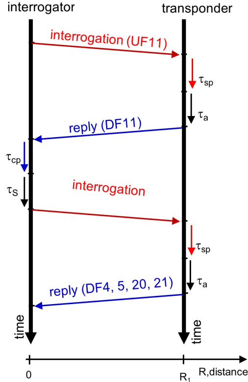
Figure 2.5. Time-flow chart for a single transponder case.
