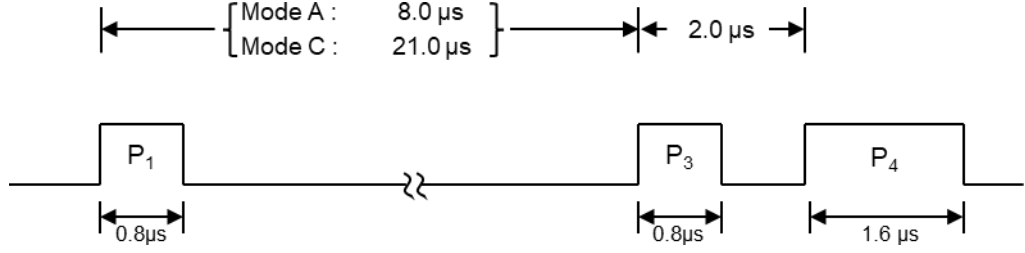
Figure 1.3. Mode A/C/S all-call interrogation format [27].
