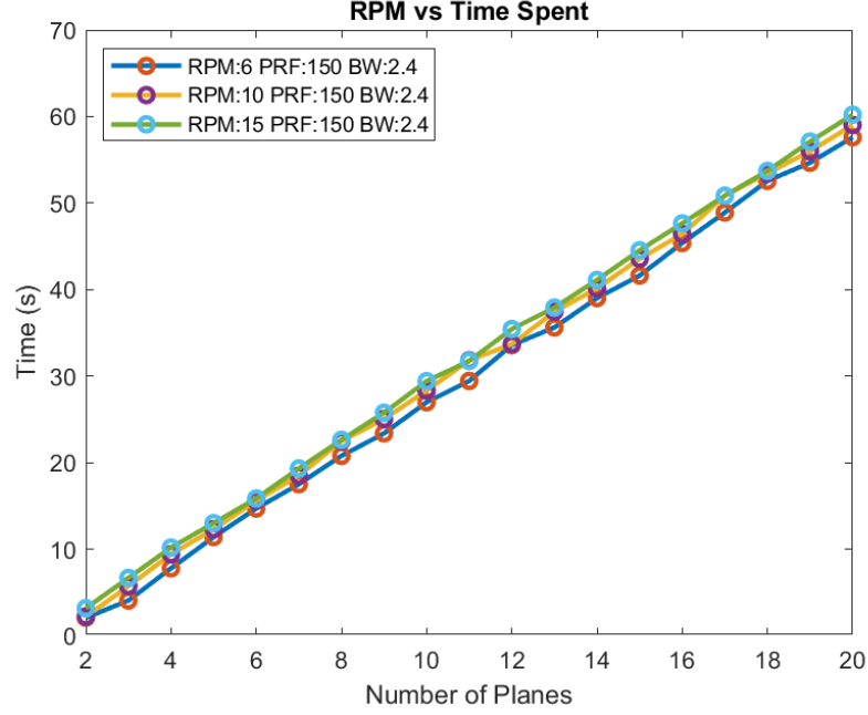
Figure 3.5. Effect of RPM on the performance of the Adaptive Algorithm.
