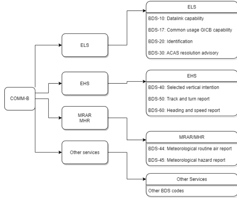
Figure 1.4. Comm-B message types [7].
