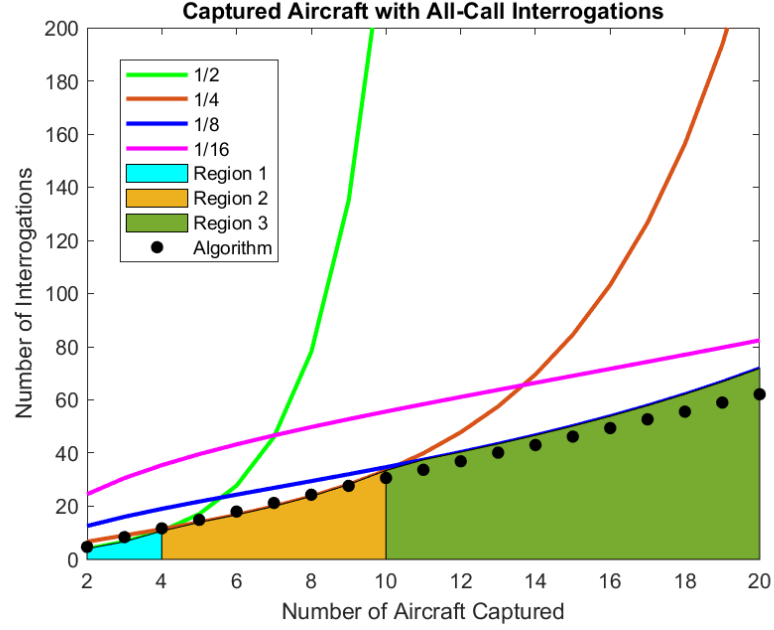
Figure 3.2. Overall performance of adaptive algorithm vs static interrogations.
