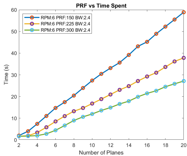
Figure 3.4. Effect of PRF on the performance of the Adaptive Algorithm.
