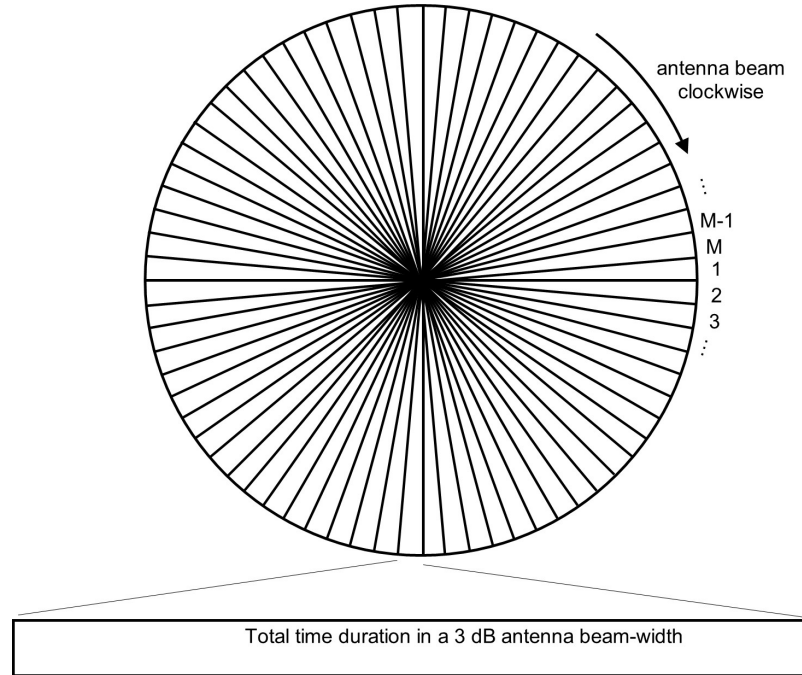
Figure 2.2. Azimuth space divided by antenna into M slices.
