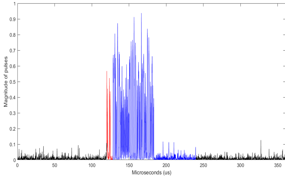
Figure 2.15. Real-time collection of 56-bit short data.
