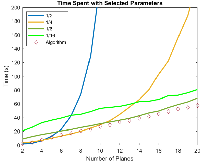
Figure 3.6. The performance of the algorithm and static methods with selected parameters, i.e., PRF: 150\text{ Hz} , BW: 2.4^\circ , and RPM: 6\text{ min}^{-1} .
