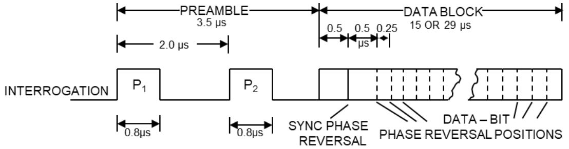
Figure 1.2. Mode-S uplink pulse sequence [27].
