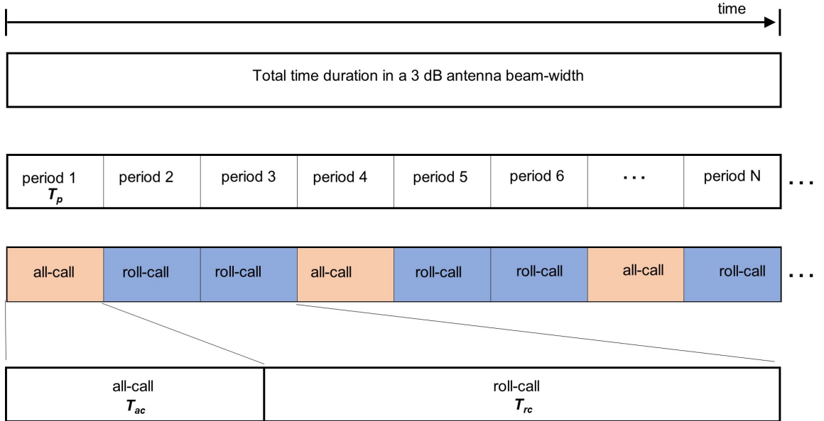
Figure 2.3. Dividing time into periods in an antenna 3-dB beam-width duration.
