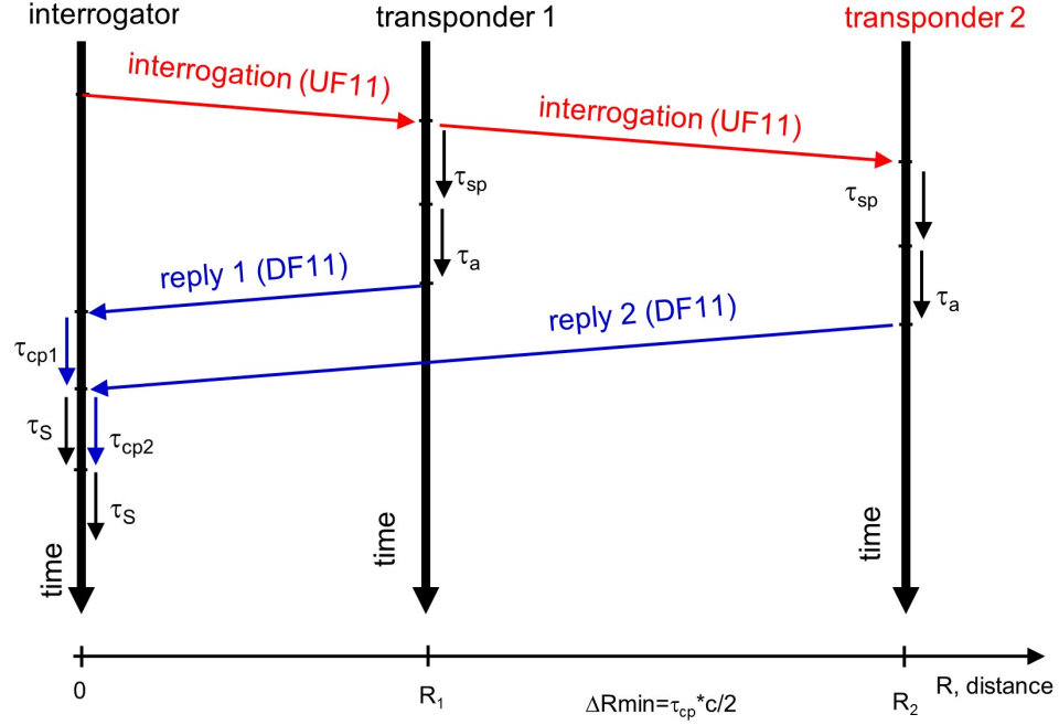
Figure 2.7. Time-flow chart for two transponders flying distant to each other in succession.
