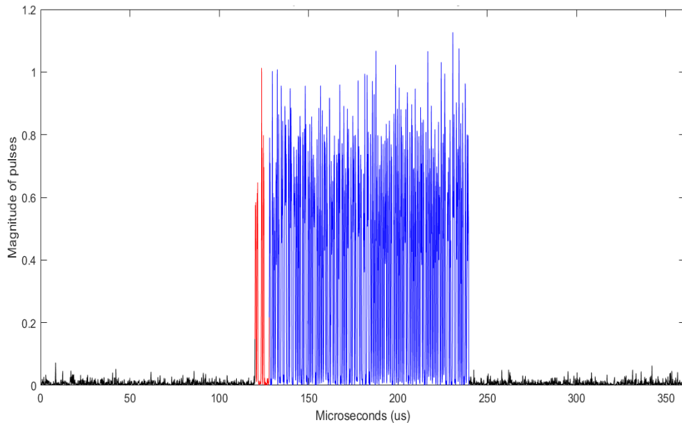
Figure 2.16. Real-time collection of 112-bit long data.
