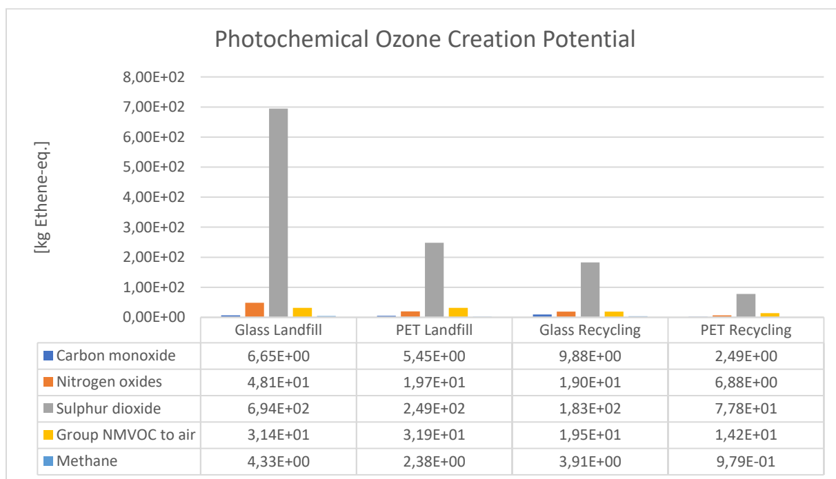
Figure 4.13. Photochemical ozone creation potential comparison of PET and glass bottle scenarios
