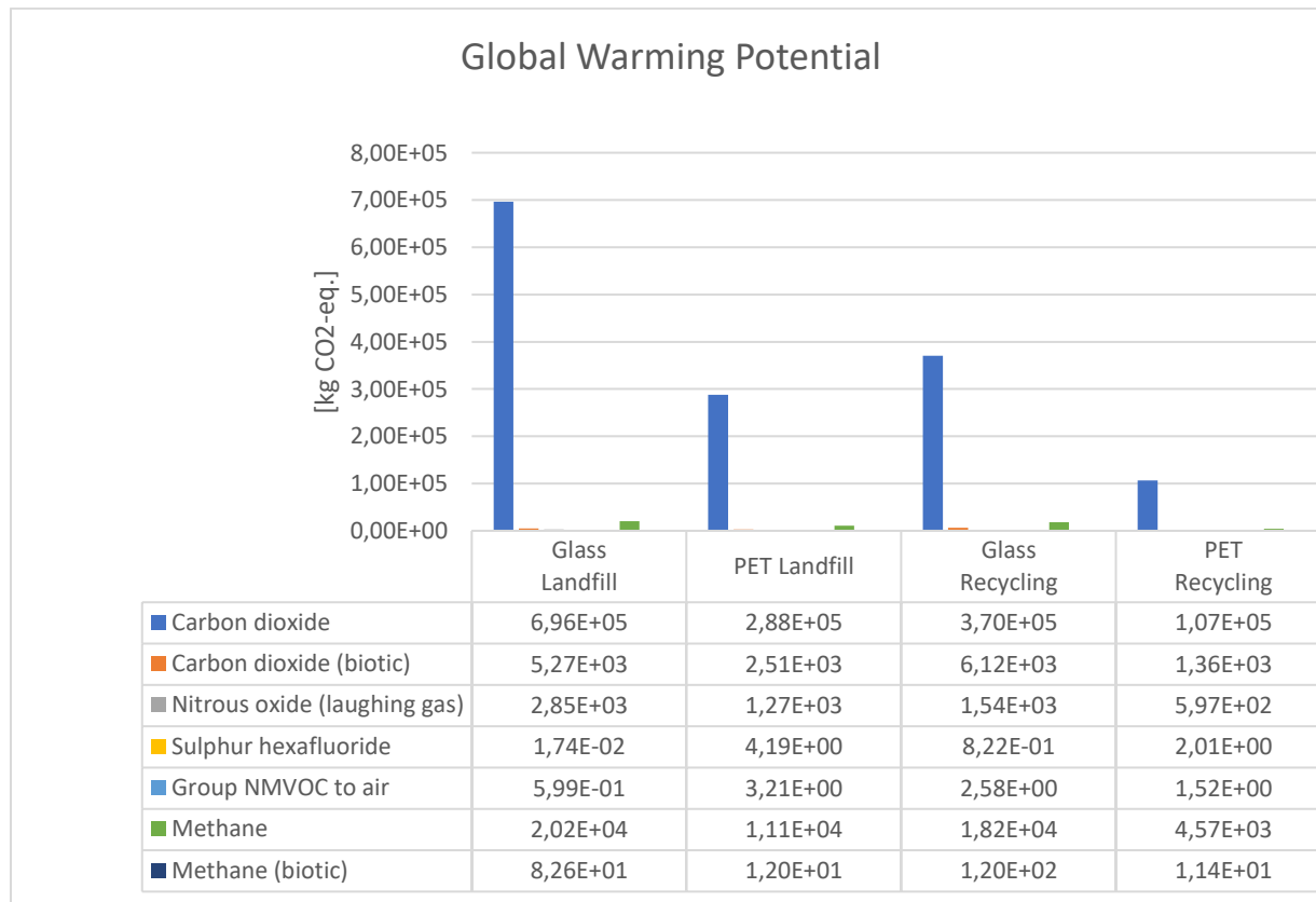
Figure 4.11. Global warming potential comparison of PET and glass bottle scenarios
