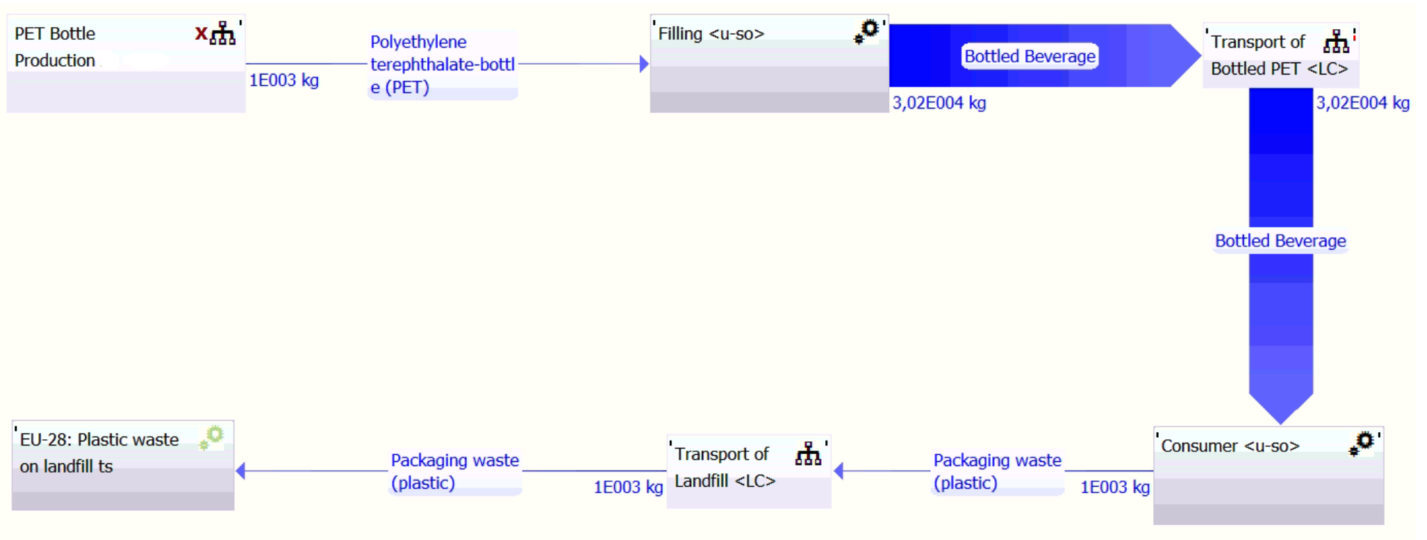
Figure 3.7. Landfill scenario of 1-ton PET bottle
