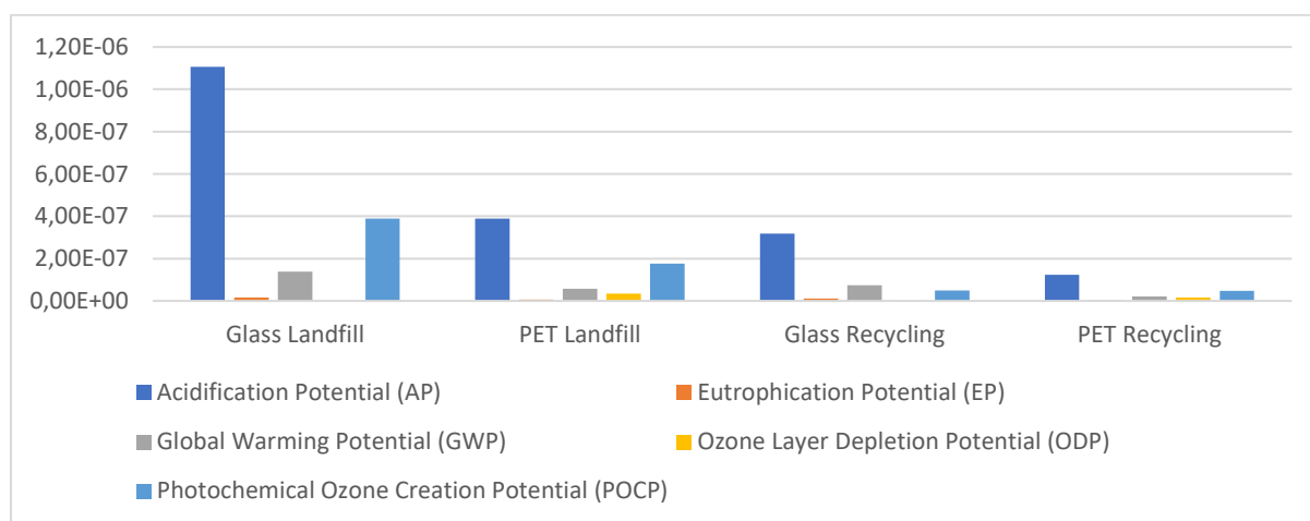
Figure 4.14. Comparison of normalization results of PET and glass bottle scenarios
