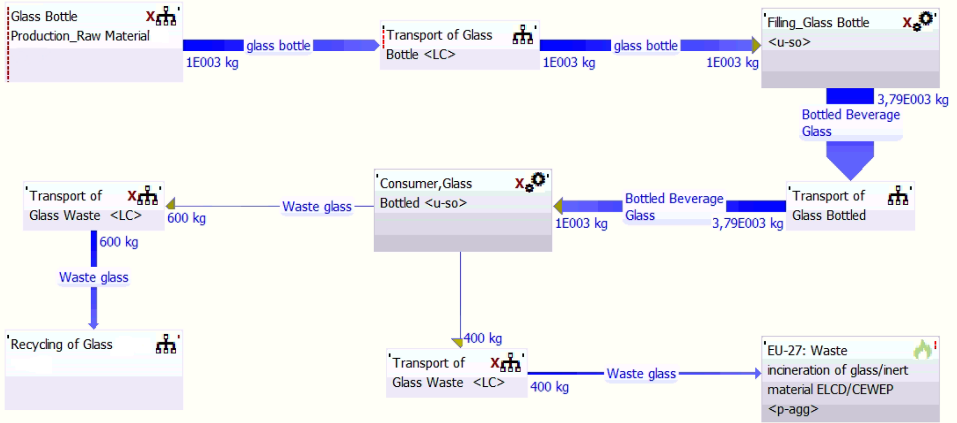
Figure 3.11. Incineration scenario for 1-ton glass bottle
