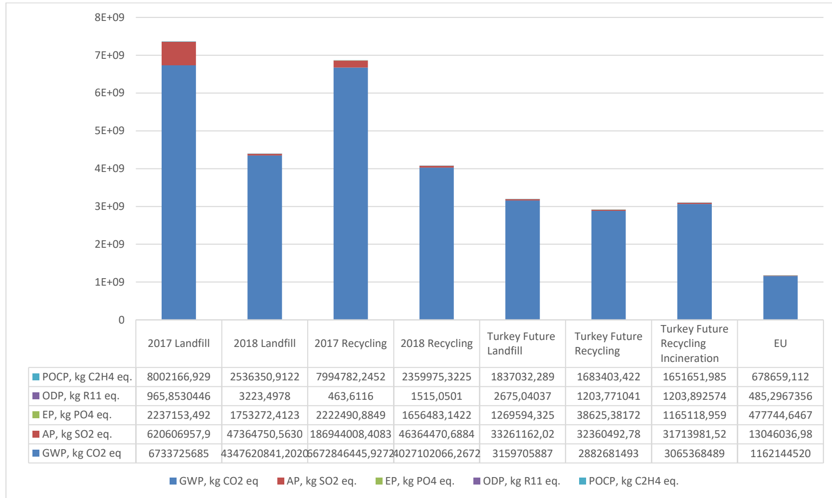
Figure 4.2. Annual impacts of PET bottle life cycle for all scenarios
