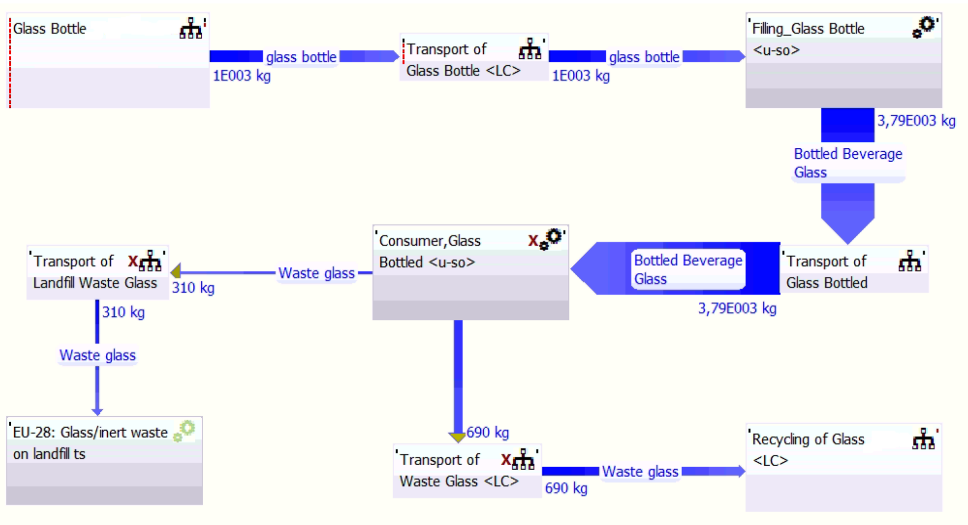
Figure 3.10. Recycling scenario for 1-ton glass bottle
