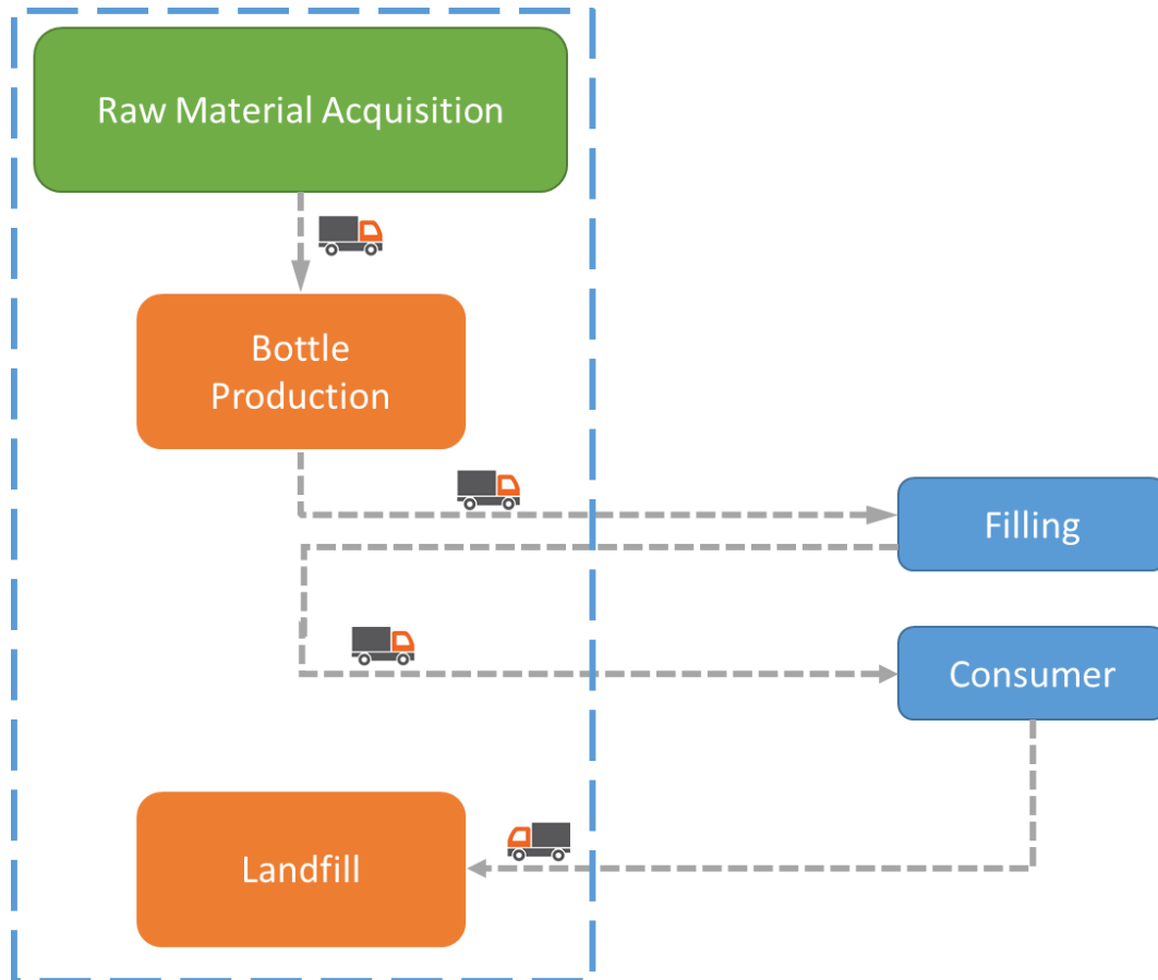
Figure 3.6. System boundaries of both PET and glass bottles
