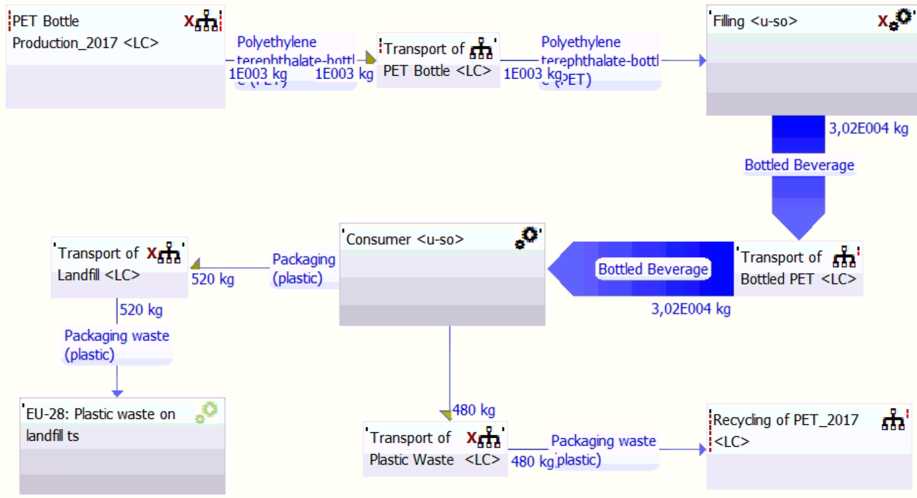
Figure 3.8. Recycling scenario of 1-ton PET bottle
