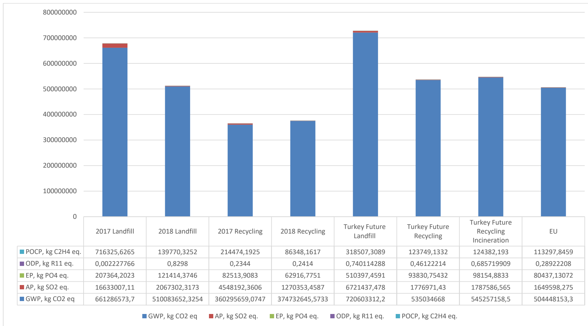
Figure 4.6. Annual impacts of glass bottle life cycle for all scenarios
