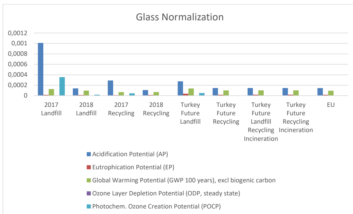
Figure 4.7. Normalization results of Glass Bottle Production for different scenarios
