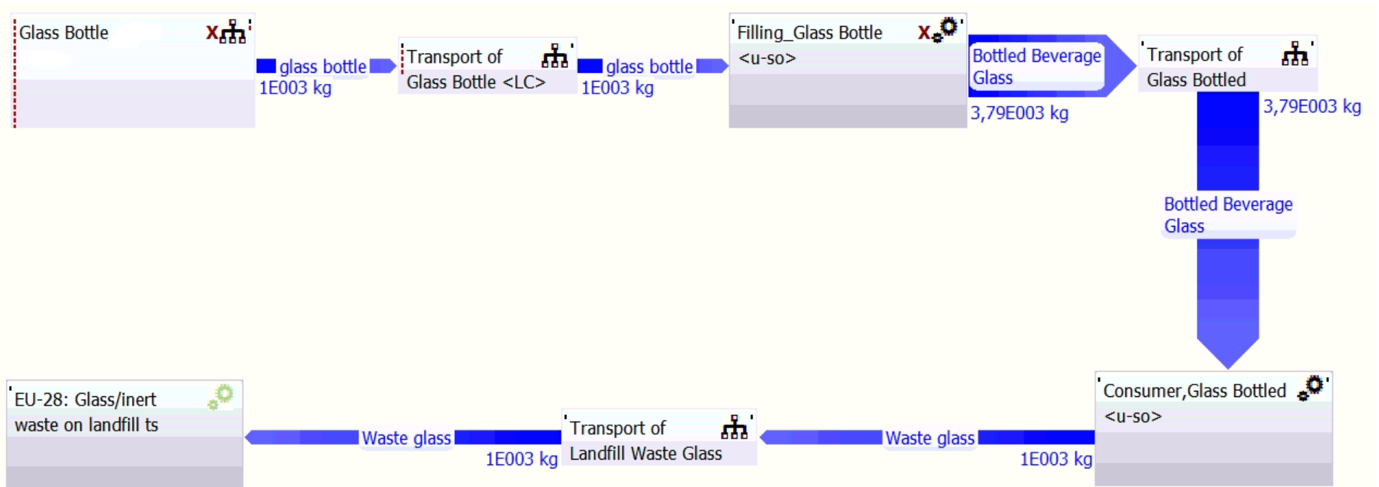
Figure 3.9. Landfill scenario for 1-ton glass bottle
