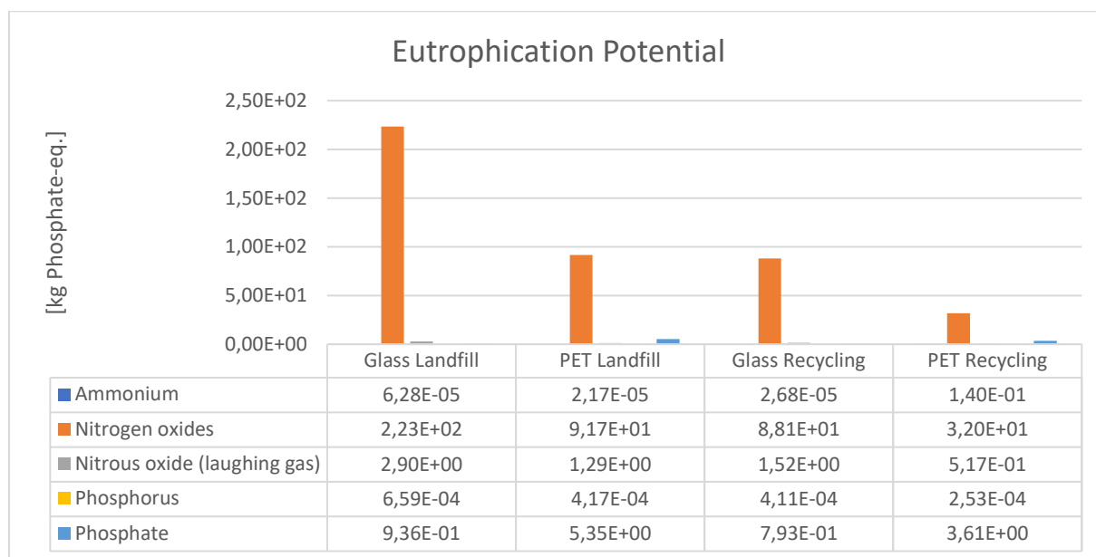
Figure 4.10. Eutrophication potential comparison of PET and glass bottle scenarios
