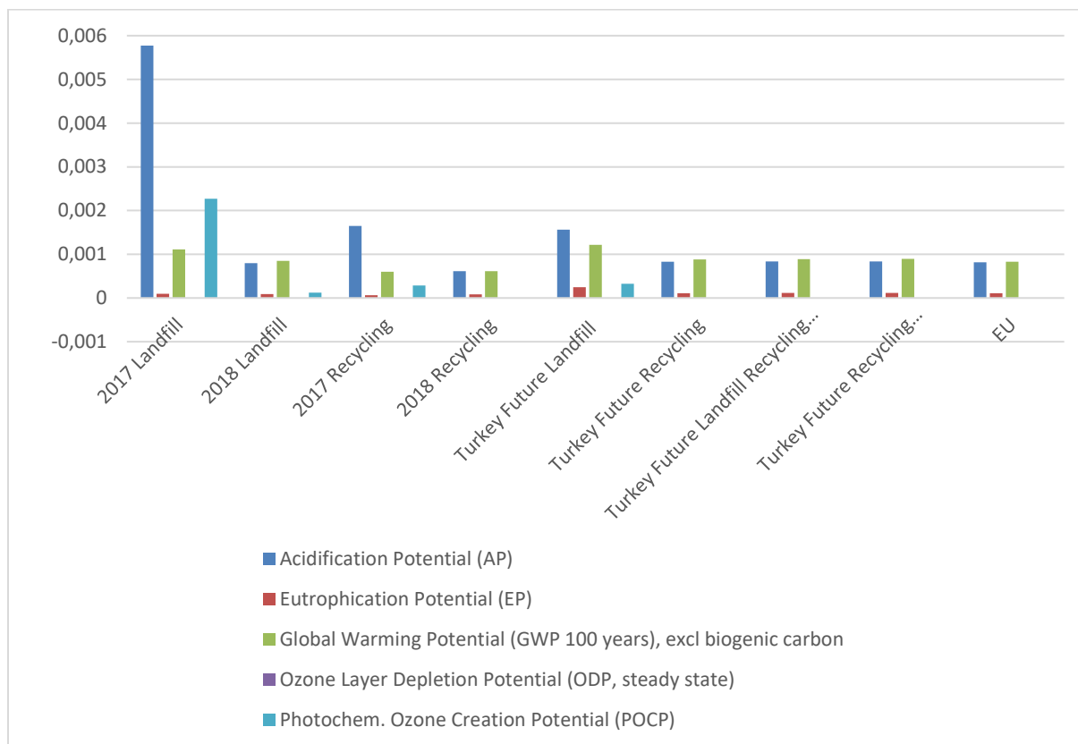
Figure 4.8. Weighting results of Glass Bottle Production for different scenarios.
