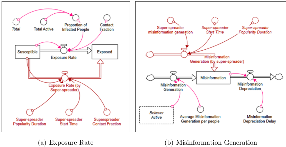
Figure 8.2. Modified Stock-Flow diagrams after incorporating super-spreader: (a) Exposure Rate, (b) Misinformation Generation.
