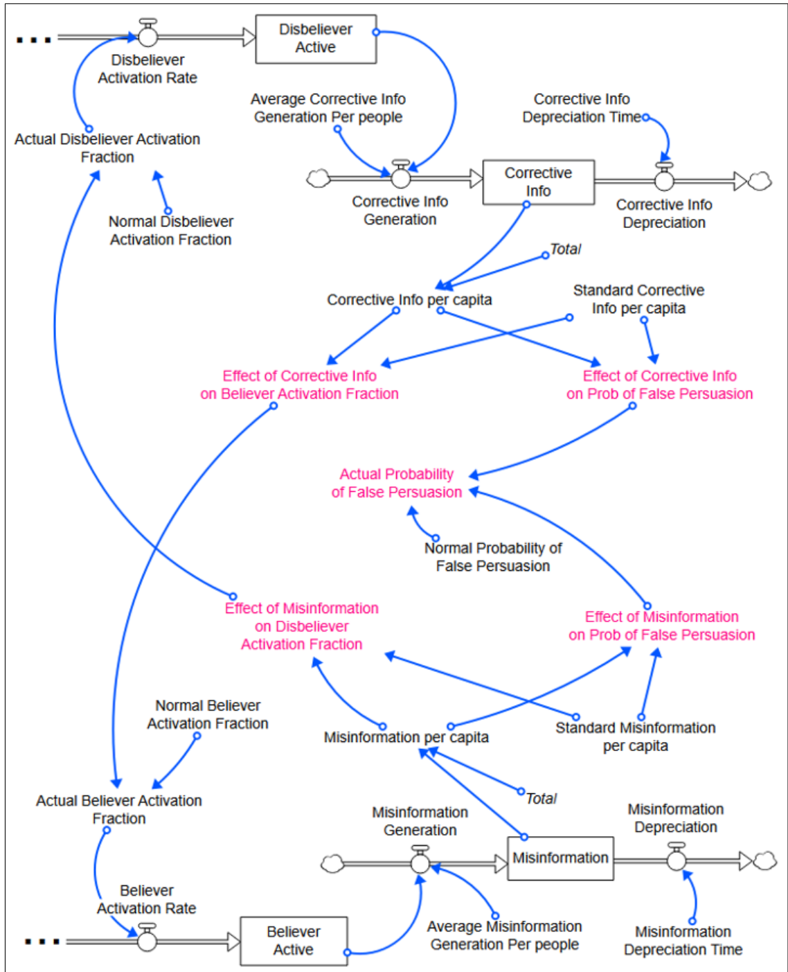
Figure 5.2. Information stocks and effect functions.
