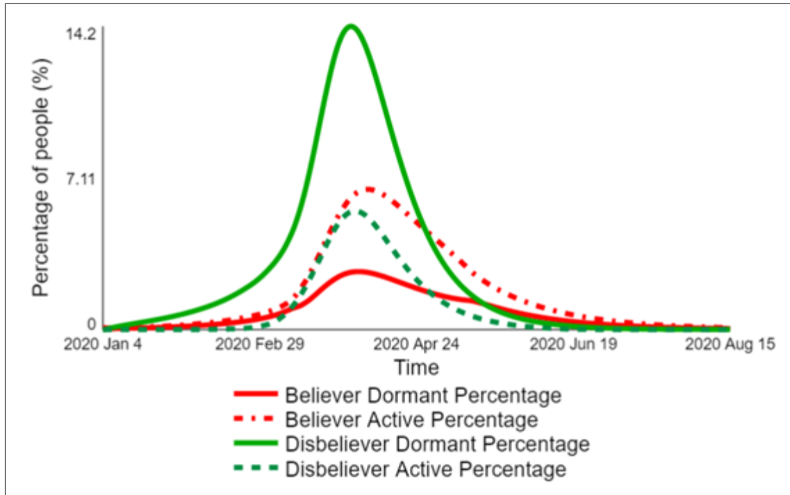
Figure 6.2. Dormant & Active Stocks after calibration.
