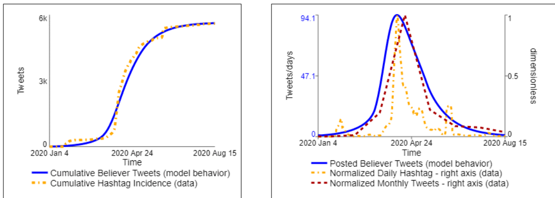
(a) Cumulative Hashtag Incidence (data from [20])
