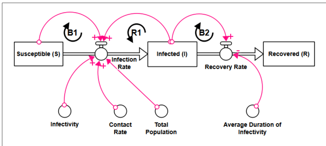
Figure 3.1. Stock-flow Diagram for the simple SIR model with causal loops.
