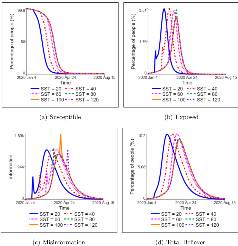
Figure 8.3. Comparative plots of stocks for different start times of super-spreader: (a) Susceptible, (b) Exposed, (c) Misinformation, and (d) Total Believer.
