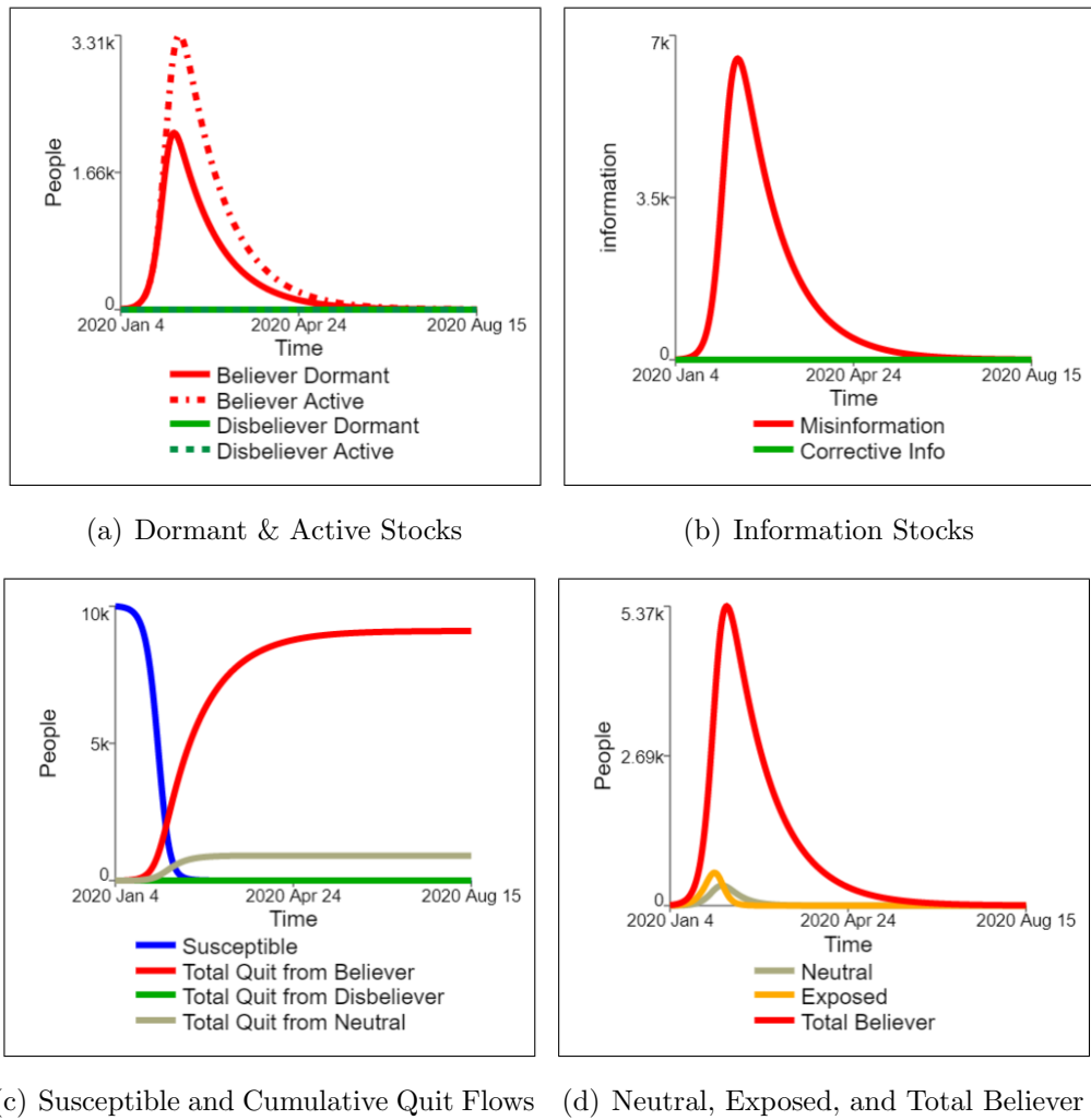
Figure B.3. Extreme condition test results of having Normal Probability of False Persuasion = 0.999: (a) Dormant & Active Stocks, (b) Information Stocks, (c) Susceptible and Cumulative Quit Flows, and (d) Neutral, Exposed, and Total Believer.
