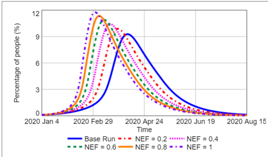
Figure 8.1. The comparative plot of Total Believer Percentage for different values of Neutral Engagement Fraction.
