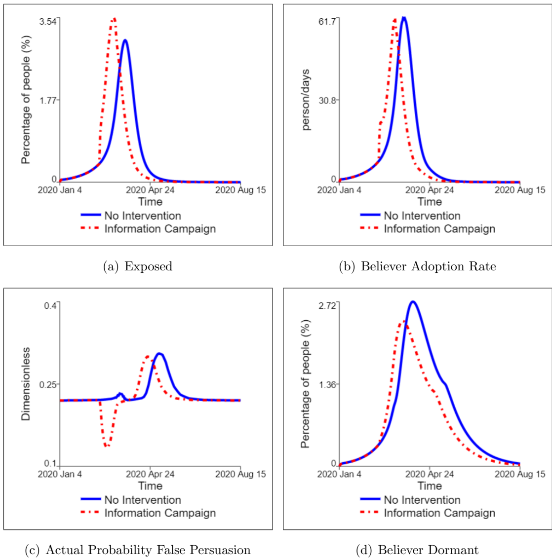
Figure 9.5. Comparative plots for the Information Campaign and no intervention cases: (a) Exposed, (b) Believer Adoption Rate, (c) Actual Probability of False Persuasion, and (d) Believer Dormant.
