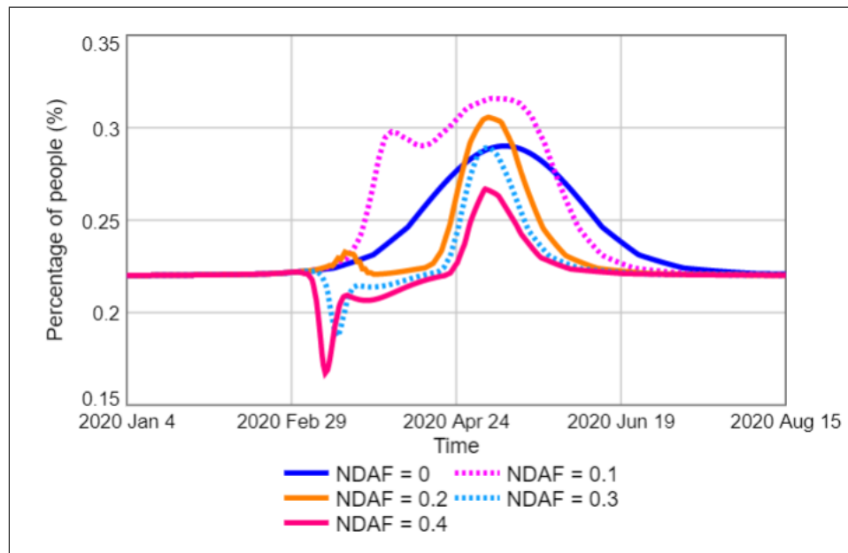
Figure 9.3. The comparative plot of Total Believer Percentage for different values of Normal Disbeliever Activation Fraction (NDAF).
