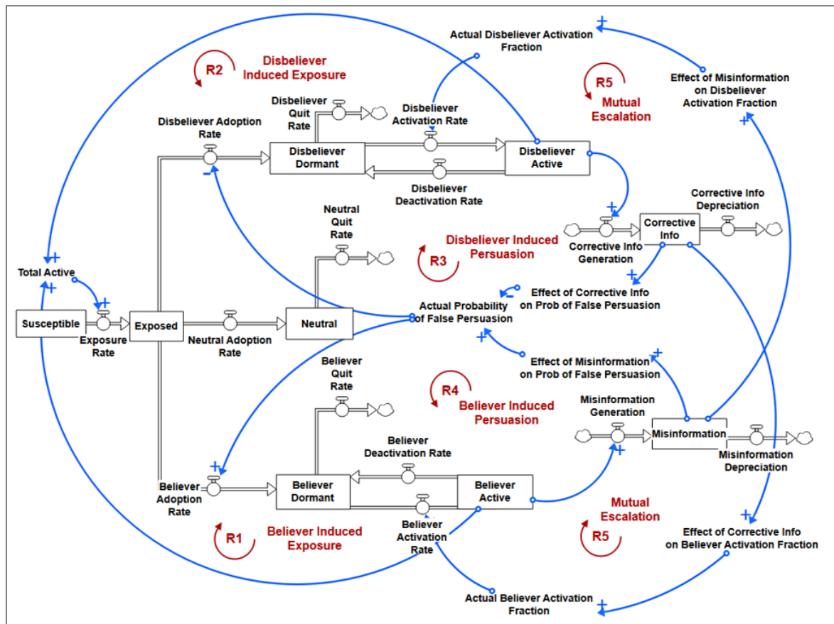
Figure 4.1. The simplified structure of the model and causal loops.
