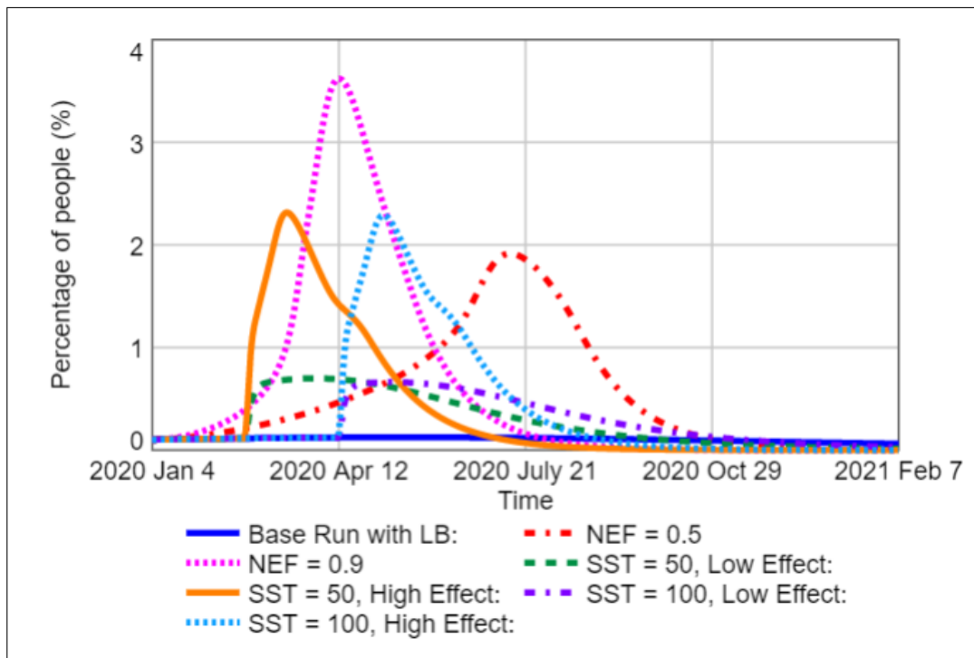
Figure 8.4. The comparative plot of Total Believer Percentage for low believability with neutral sharing and super-spreader scenarios.
