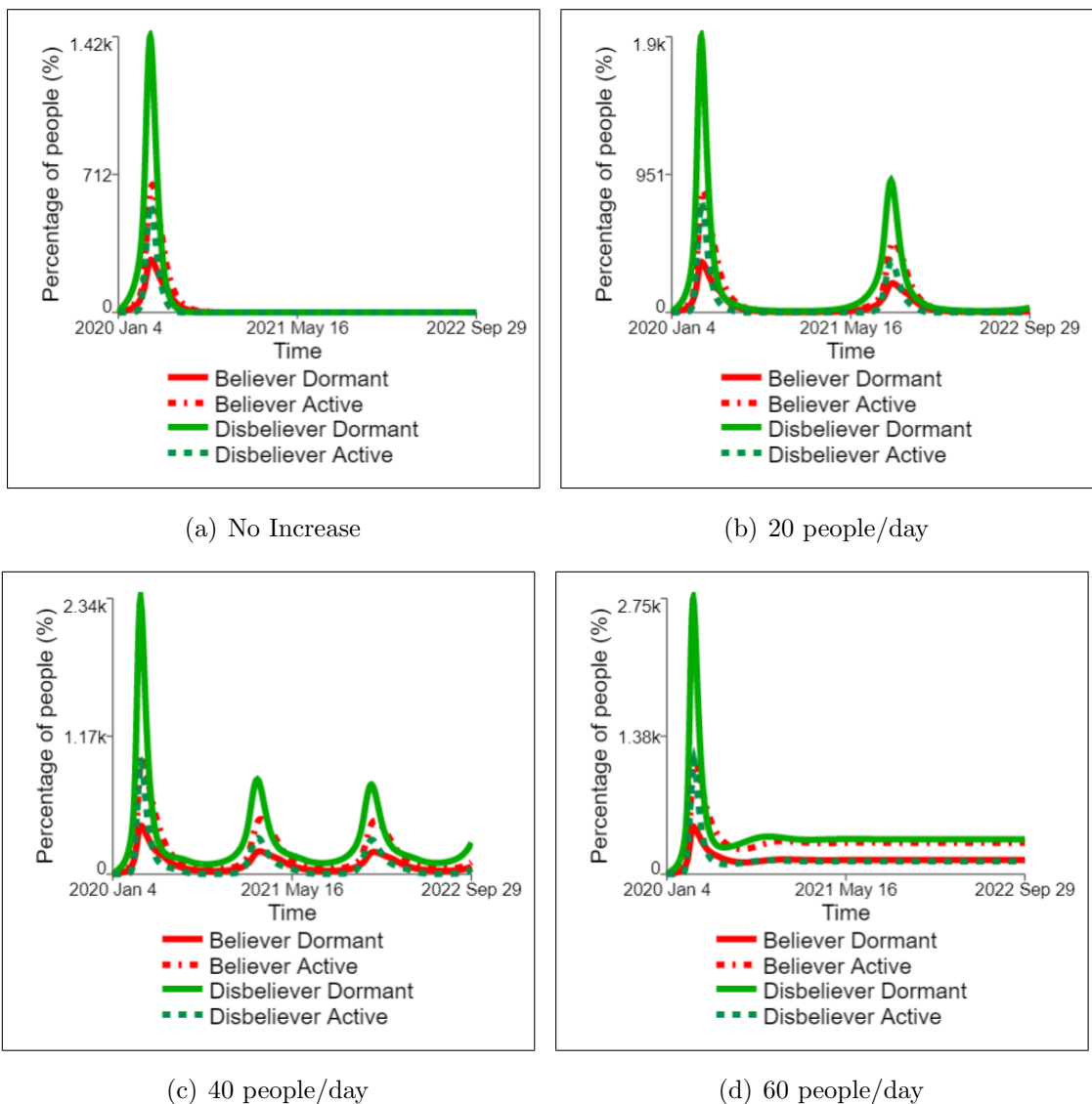
Figure 8.5. Comparative plots of Dormant and Active stock dynamics for different levels of constant inflow to the Susceptible: (a) No Increase, (b) 20 people/day, (c) 40 people/day, and (d) 60 people/day.
