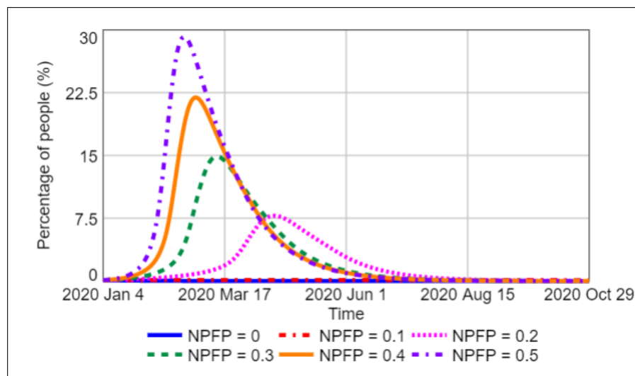
Figure 7.2. Sensitivity of Total Believer to Normal Probability of False Persuasion (NPFP).
