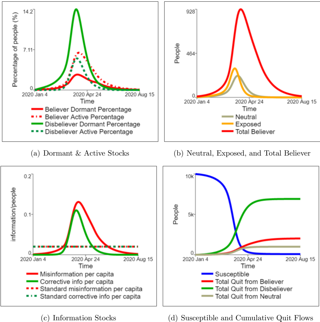
Figure 7.1. Resulting stock dynamics for the Base Run: (a) Dormant & Active Stocks, (b) Neutral, Exposed, and Total Believer, (c) Information Stocks, and (d) Susceptible and Cumulative Quit Flows.
