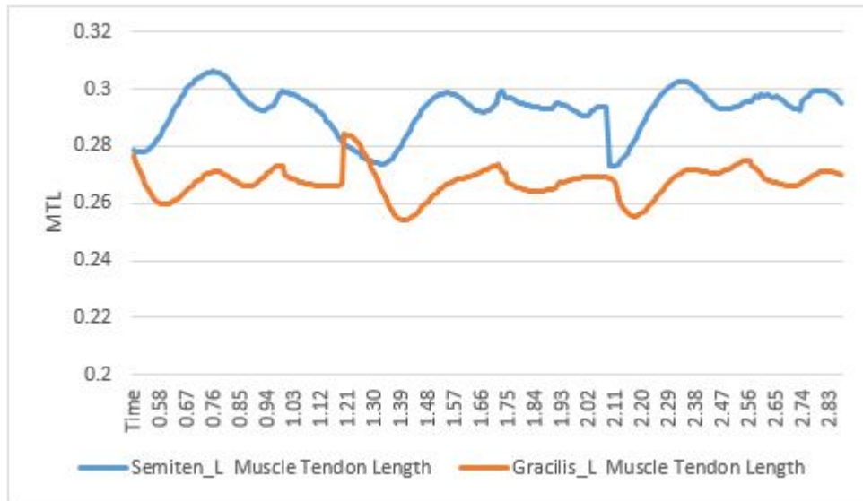
Figure 3.29 Limb 10 GRA and ST muscle-tendon complex length changes during the gait cycle.
