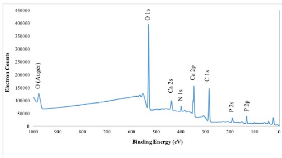
Figure 4.17 Survey Scan of HA modified CH/GO nanocomposite membranes (AlK Alpha Source Gun, Pass Energy 150.0 eV, 300 \mu\text{m} spot size).
