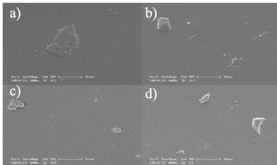
Figure 4.13 SEM images (5000x) of CH/GO nanocomposite membrane were analyzed 3 observe surface defects after UV/Ozone treatment a) CH/GO nanocomposite membrane without treatment b) 1 minute c) 2 minutes d) 5 minutes .
