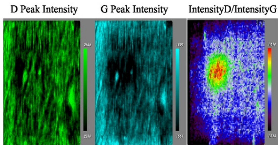
Figure 4.20 D and G peak intensity and ratio.
