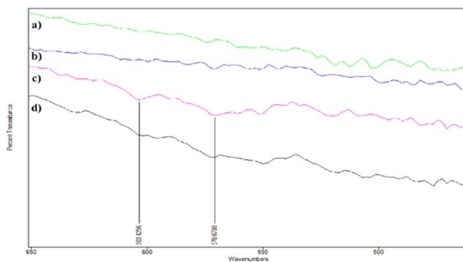
Figure 4.11 FT-IR spectra of a) CH b) CH/HA 1min UV/Ozone treatment c) CH/HA 2 min UV/Ozone treatment d) CH/HA 5 min UV/Ozone treatment 650\text{ cm}^{-1} and 400\text{ cm}^{-1} .
