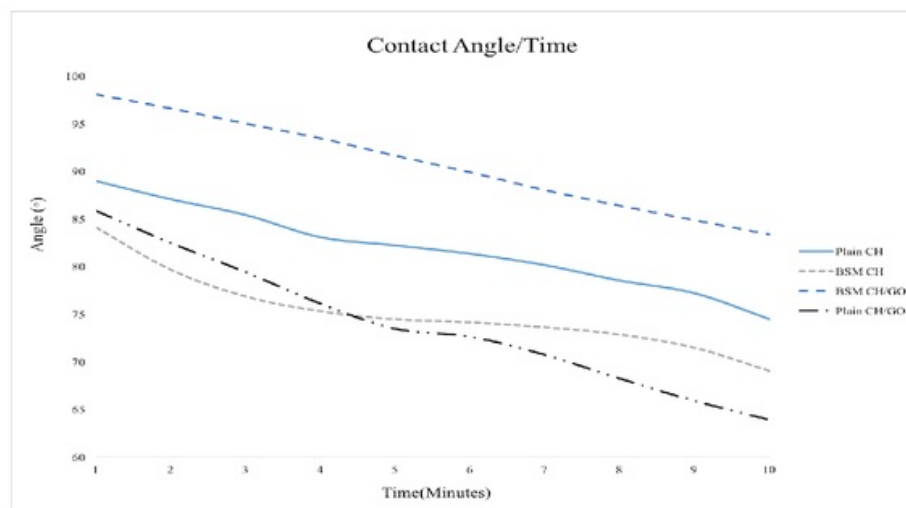
1 Figure 4.7 Measurement of water contact angle of plain CH, BSM CH, plain CH/GO and BSM CH/GO membranes with using PBS over 10 minutes.
