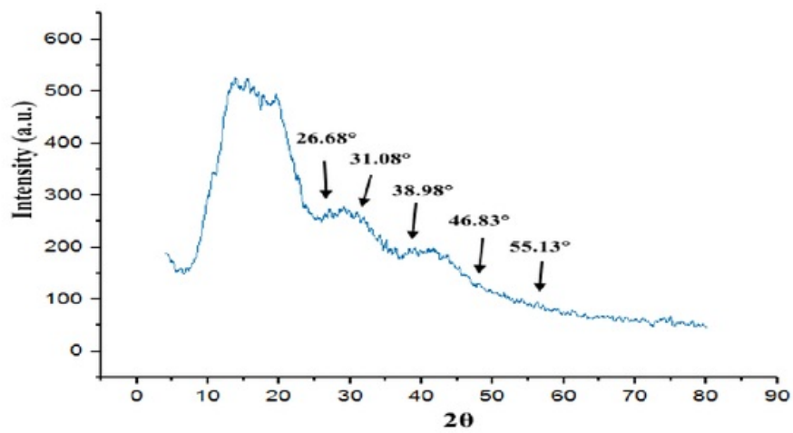
Figure 4.22 XRD spectrum of HA modified CH membrane.
