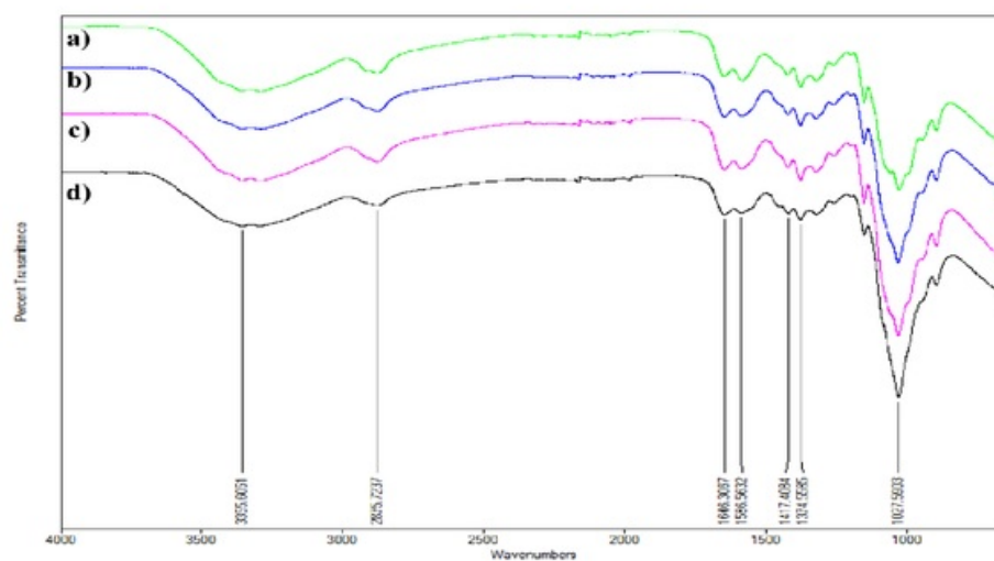
Figure 4.10 FT-IR spectra of a) CH b) CH/HA 1min UV/Ozone treatment c) CH/HA 2 min UV/Ozone treatment d) CH/HA 5 min UV/Ozone treatment 4000\text{ cm}^{-1} and 650\text{ cm}^{-1} .
