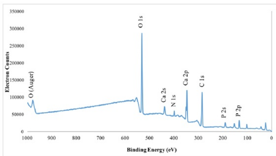
Figure 4.16 Survey scan of HA modified CH membrane (AlK Alpha Source Gun, Pass Energy 150.0 eV, 300 \mu\text{m} spot size).
