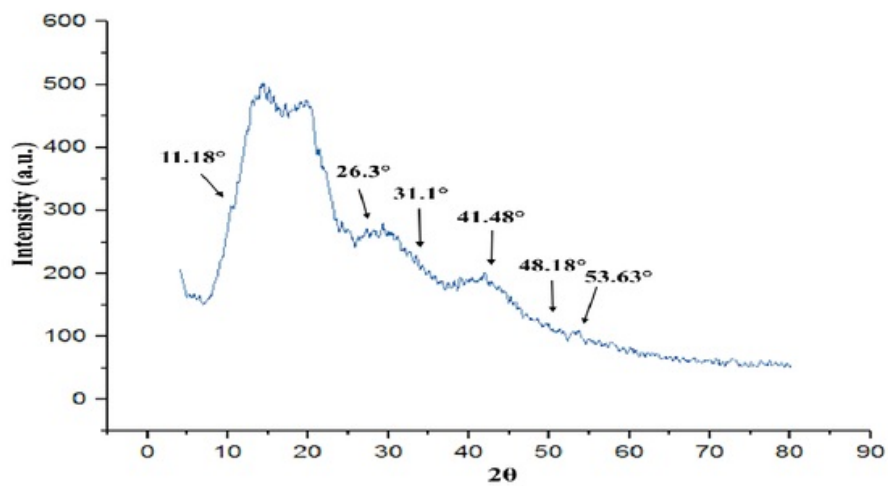
Figure 4.24 XRD spectrum of HA modified CH/GO membrane.
