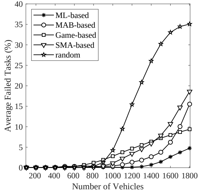
Figure 6.11. Percentage of failed tasks based on all application types.
