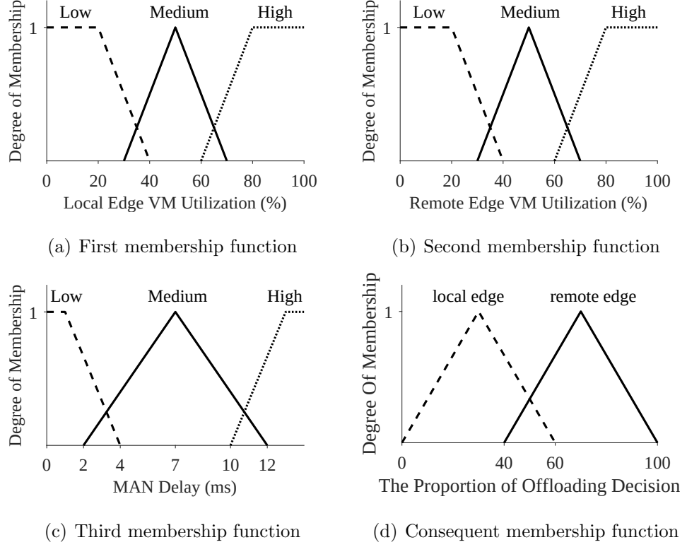
Figure 5.8. Membership functions used in the first stage.
