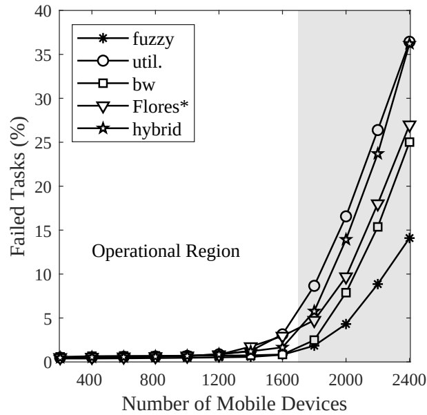
Figure 5.11. Average failed task based on all application types.
