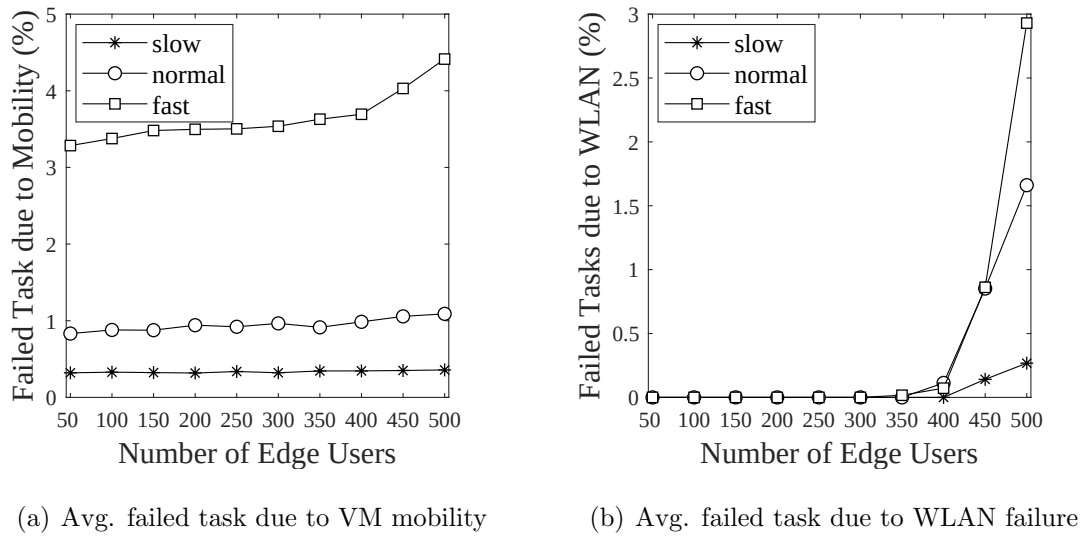
Figure 4.14. Performance evaluation of the system for different dwell time values.
