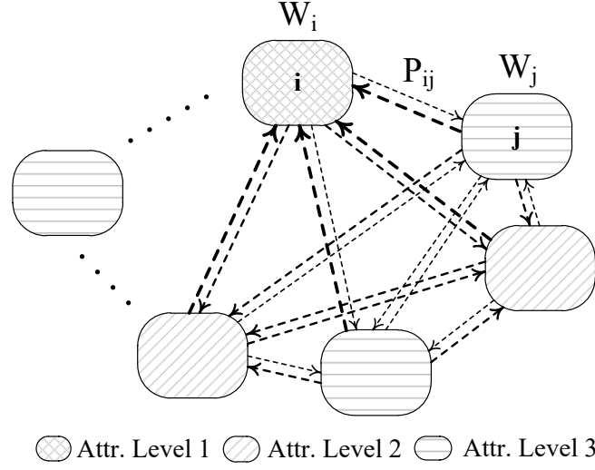
Figure 4.8. Mobility model used in the simulations.
