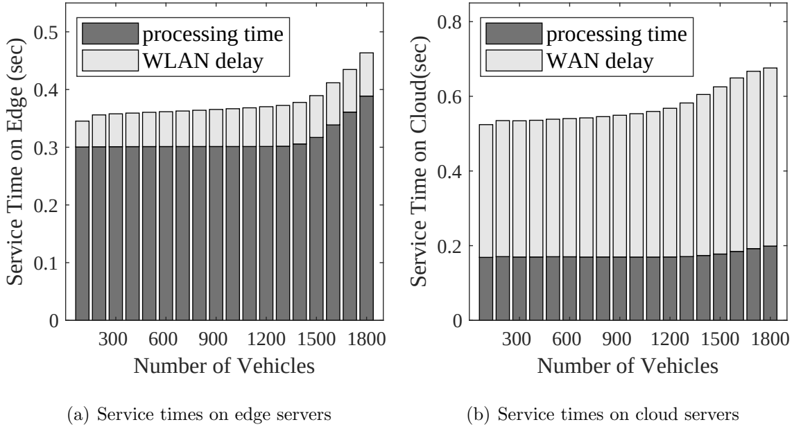
Figure 6.15. Service time ratio of the edge and cloud servers.
