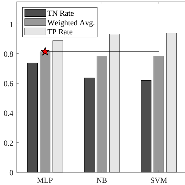
Figure 6.5. Performance comparison of the classifiers used for the edge scenario.
