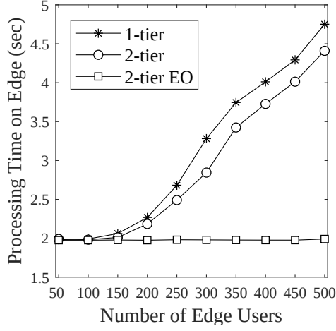
(a) Average processing time for augmented reality application
