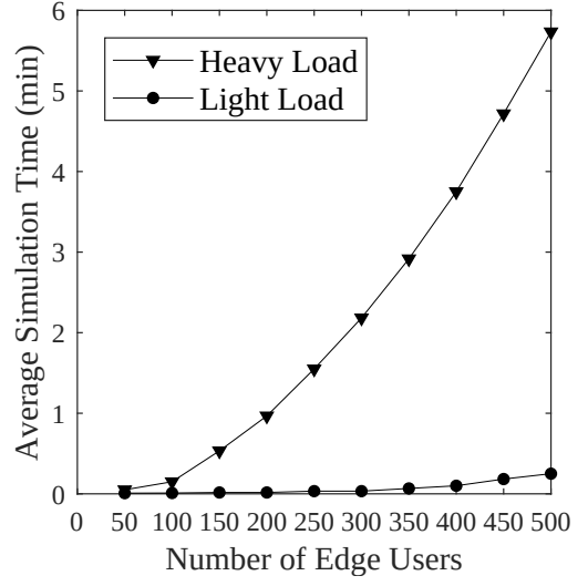
(b) Average simulation time
