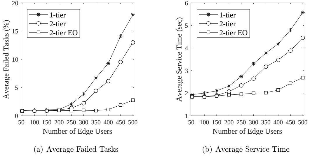
Figure 4.10. Comparative evaluation of the different edge computing architectures based on all application types.
