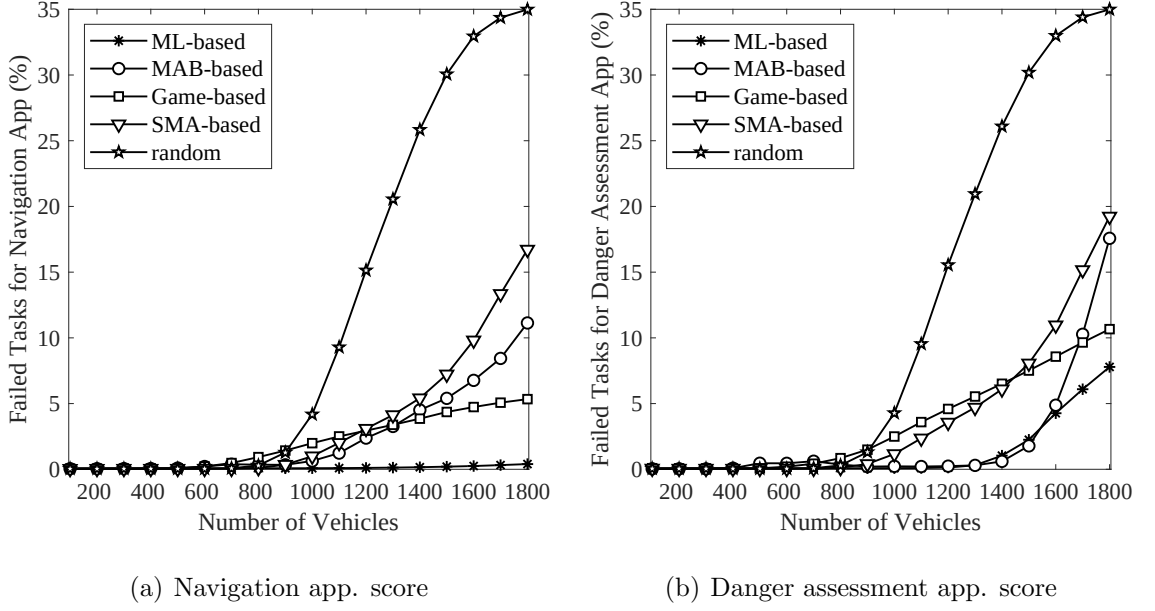
Figure 6.12. Average failed tasks for different application types.
