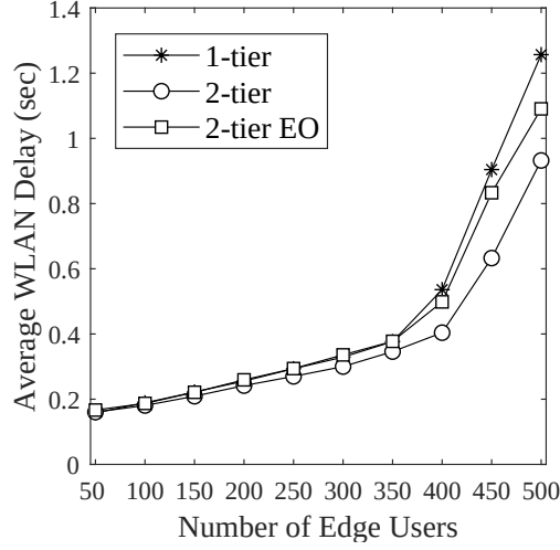
Figure 4.11. Average WLAN Delay based on all application types.
