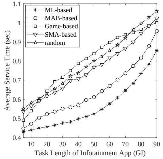
(b) Average service time (sec)
