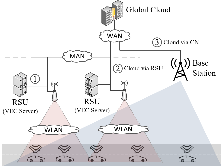
Figure 6.2. Multi-tier multi-access VEC architecture and task offloading options.
