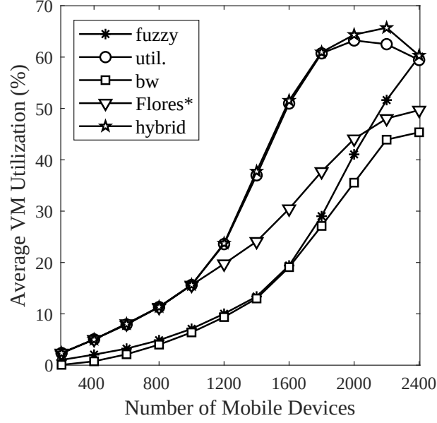
Figure 5.13. Average VM utilization based on all application types.
