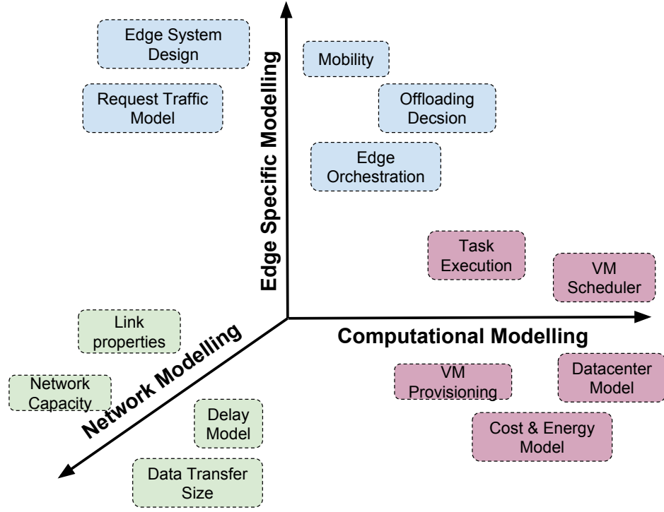
Figure 4.1. Aspects of edge computing simulation modeling.
