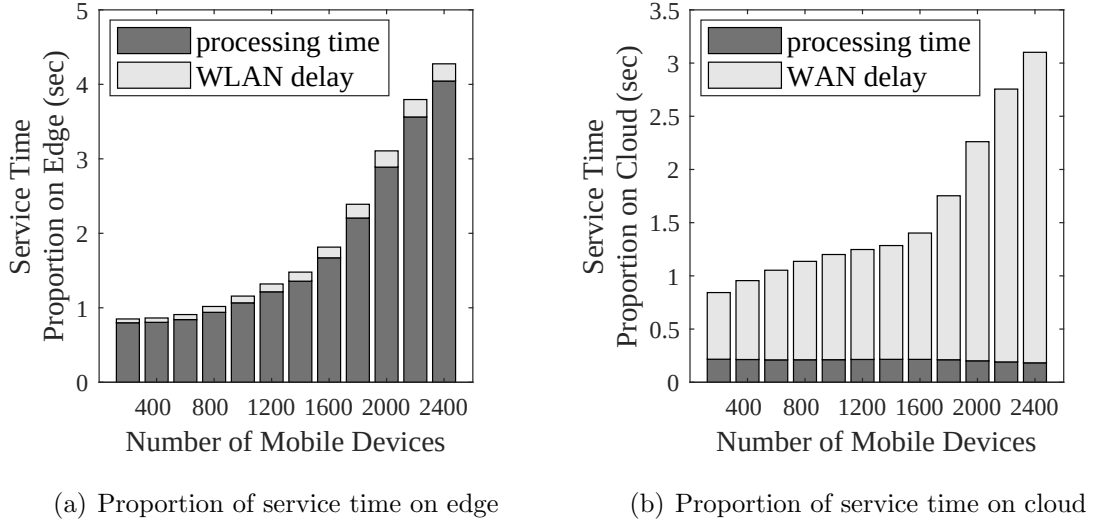
Figure 5.15. Average service time values for fuzzy based workload orchestrator.
