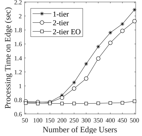
(b) Average processing time for infotainment application
