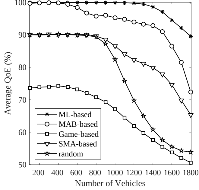
Figure 6.13. Average Quality of Experience based on all application types.
