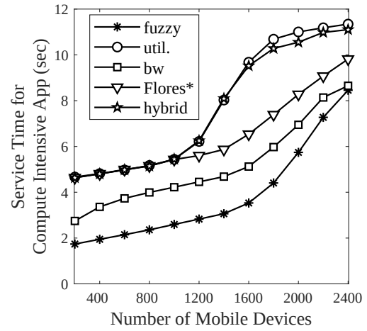
(b) Compute intensive app. score
