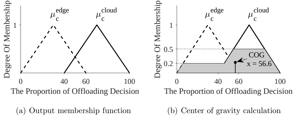
Figure 5.7. Membership function of the consequence classes.
