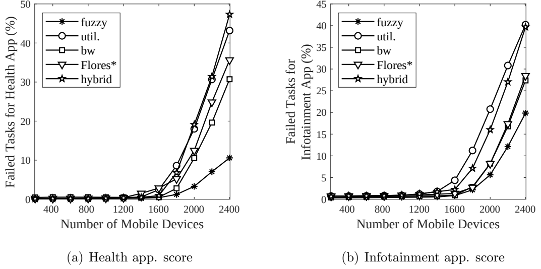
Figure 5.16. Average failed task for different application types.
