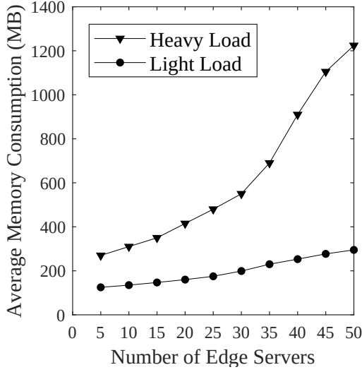
(c) Average memory consumption
