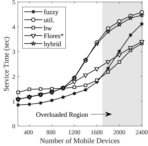
Figure 5.12. Average service time based on all application types.
