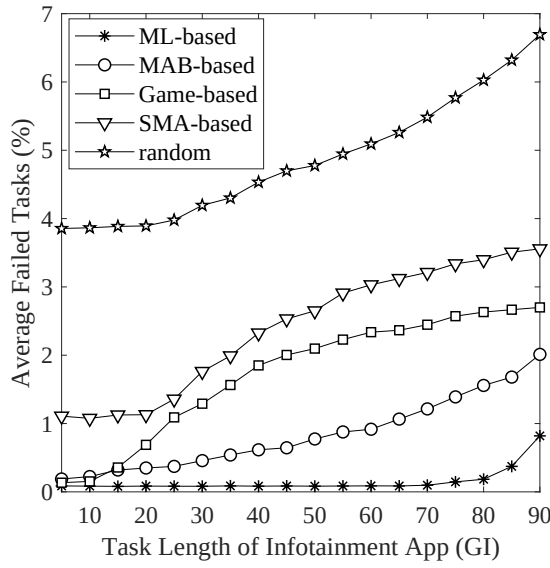
(a) Average failed tasks (%)
