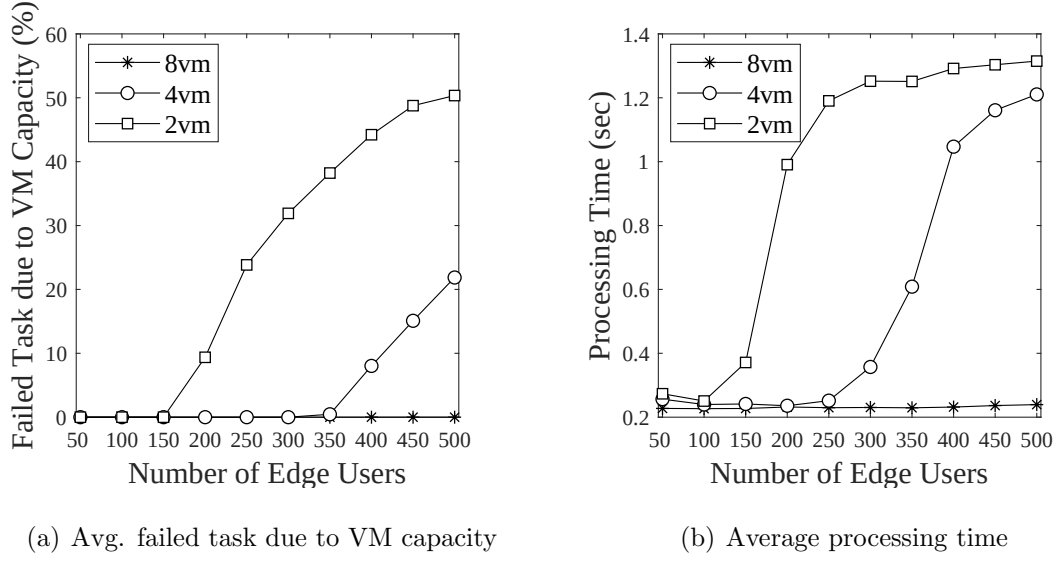
Figure 4.13. Performance evaluation of the system for different VM sizes.
