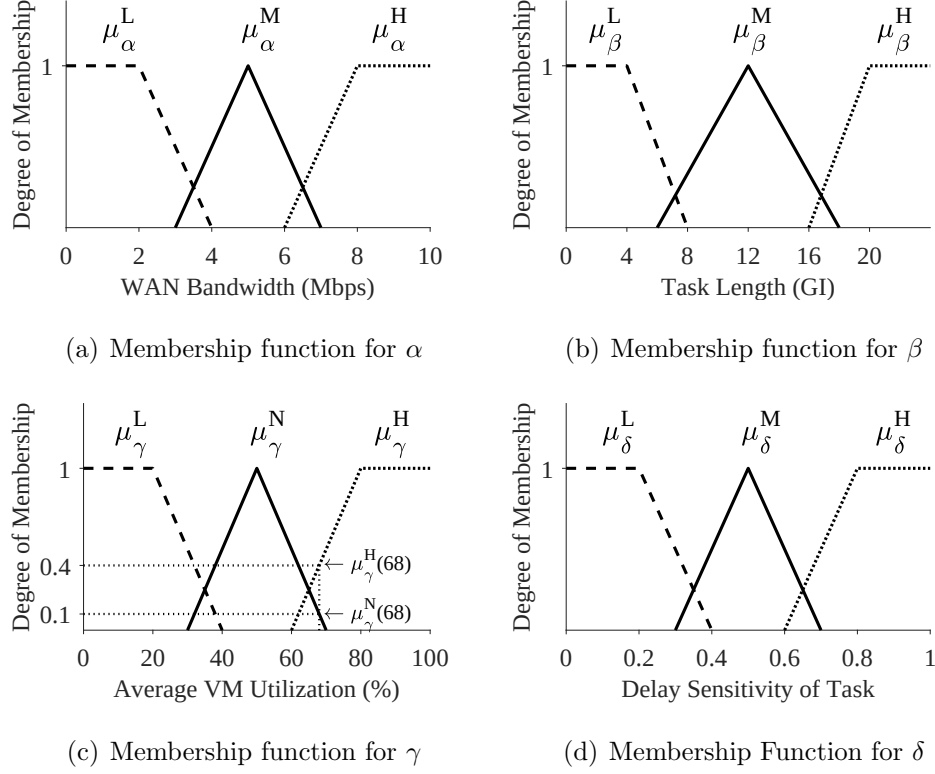
Figure 5.6. Membership functions for the fuzzy variables representing both network and computational resources.
