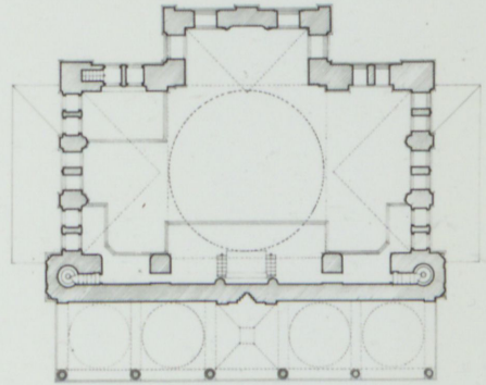
MAHFEL PLANI
