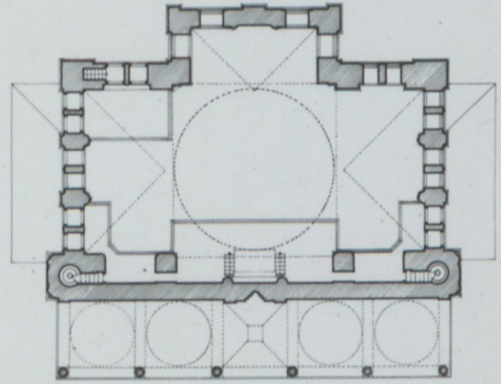
MAHFEL PLANI
