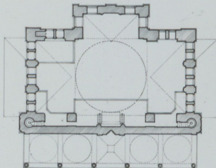
MAHFEL PLANI
