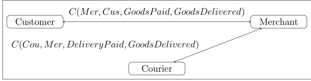
Figure 2.1. Commitment protocol to regulate the e-commerce scenario.
