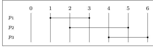
Figure 5.4. Time intervals of the properties in the CSP Example.
