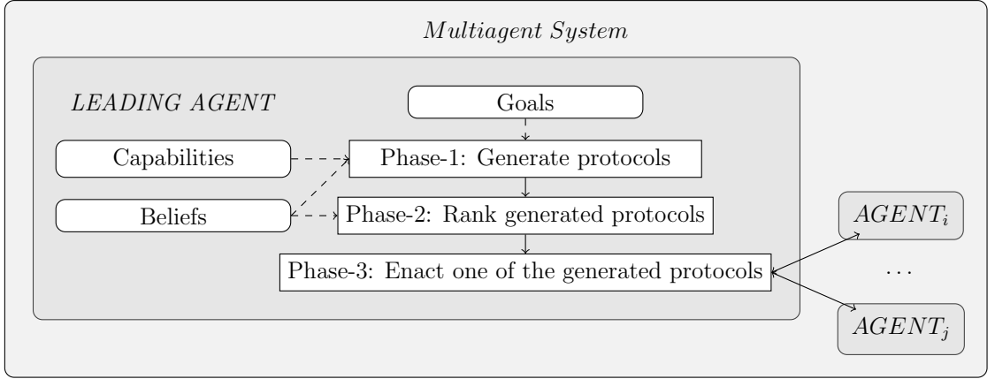
Figure 1.1. The tree-phase process that is executed by the leading agent to come up with a commitment protocol to regulate its interaction while pursuing its goals.
