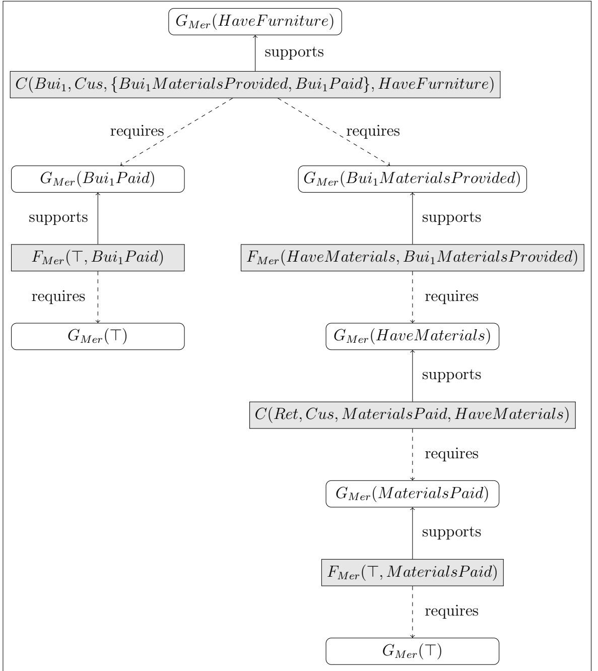
Figure 3.1. Support graph of the protocol \pi that supports G_{Cus}(\text{HaveFurniture}) .
