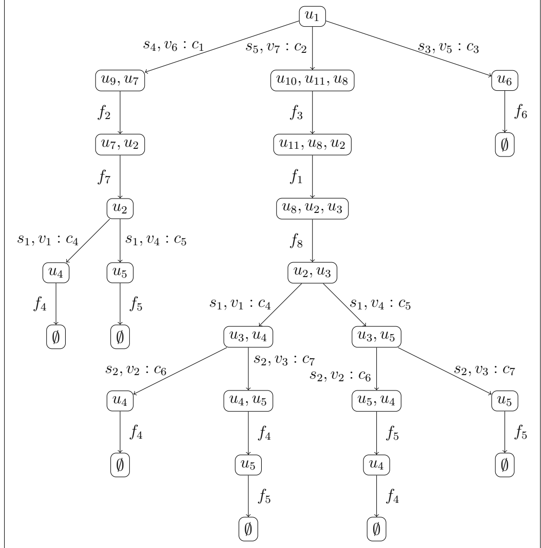
Figure 3.4. Execution trace of PROTOCOLBASED algorithm on the running example.
