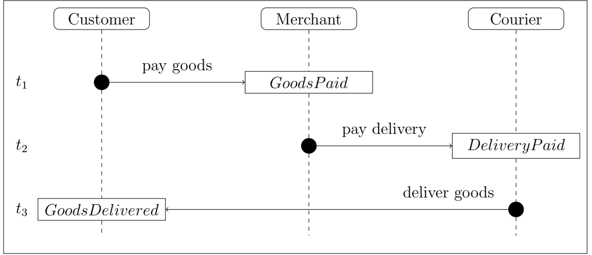
Figure 2.2. A possible execution of the commitment protocol of the e-commerce scenario.
