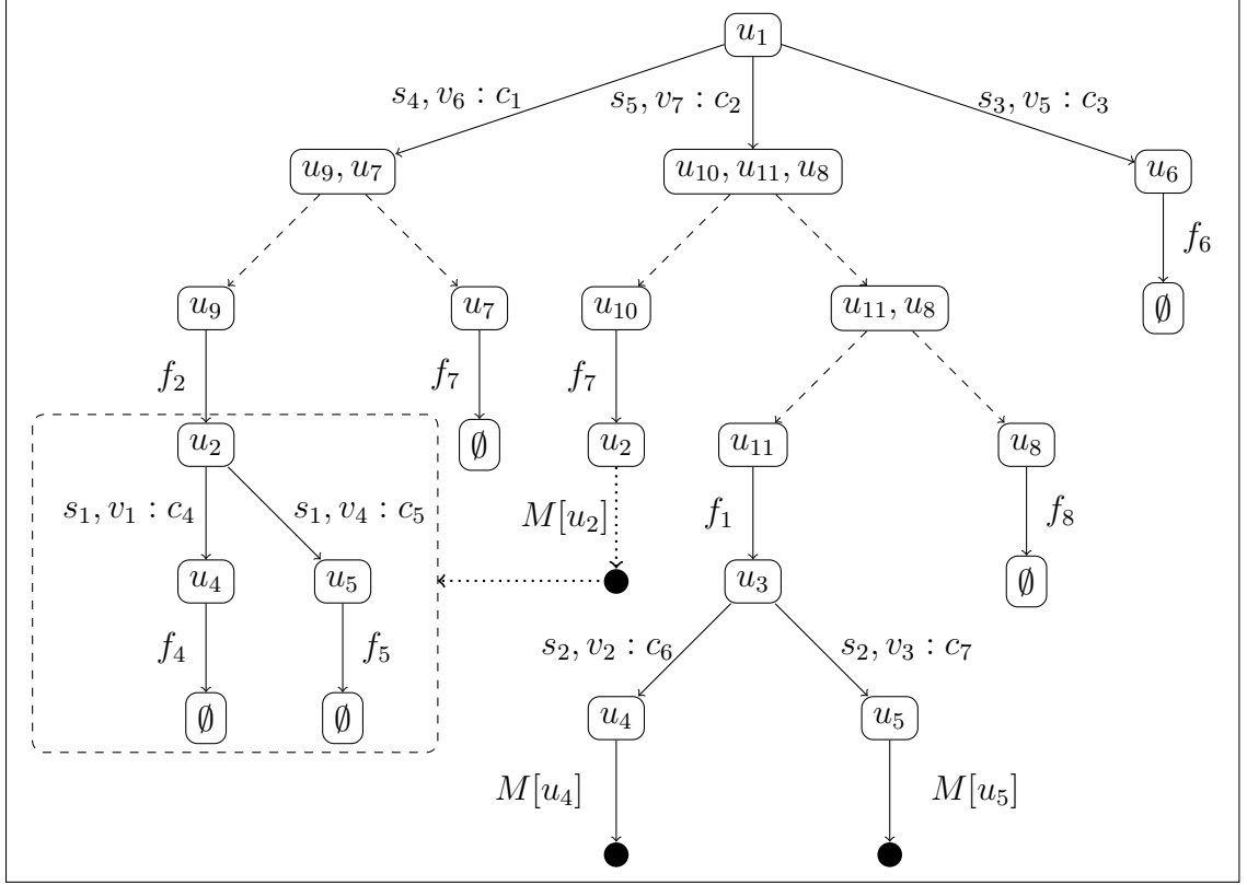
Figure 3.5. Execution trace of GOALBASED algorithm on the running example.
