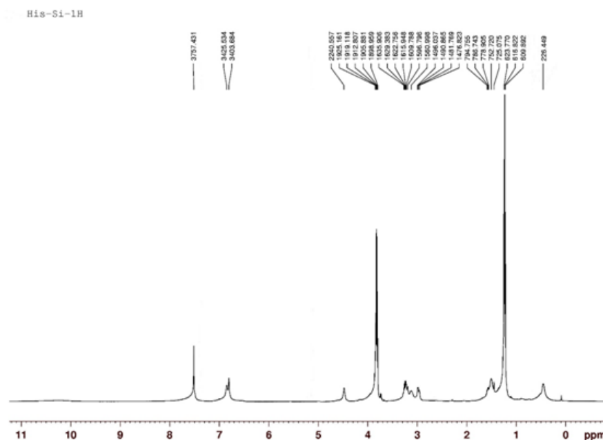
Figure 4.1 ^1\text{H-NMR} spectrum of Histidine conjugated self assembled molecule.
