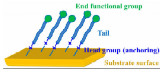
Figure 2.5 General structure of Self Assembled Monolayers [5].
