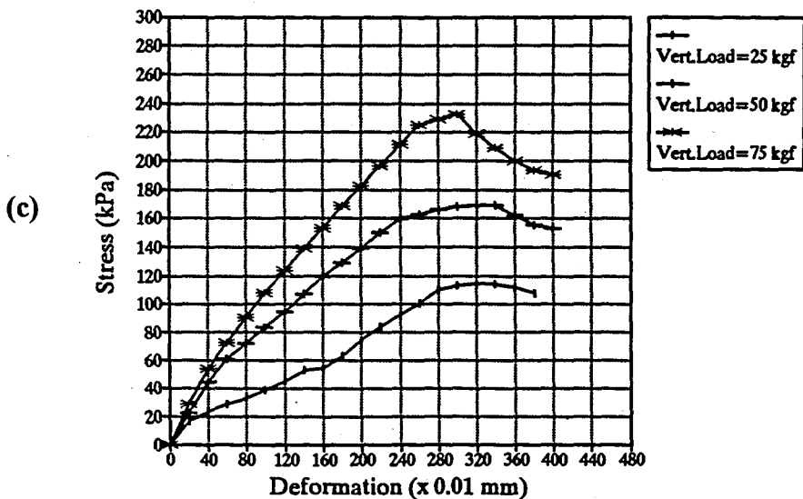
FIGURE A.14. Shear Strength vs deformation behavior of layered samples (soil sections: 30% sand and 70% bent.) a)with no lime, b)with 3% lime, c)with 7% lime
