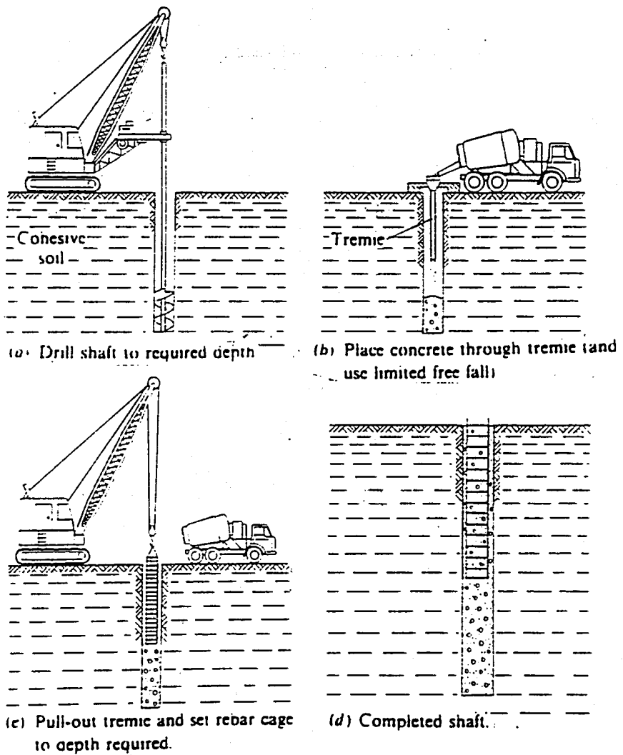
FIGURE 2.11. Dry method of drilled pier construction [30]
