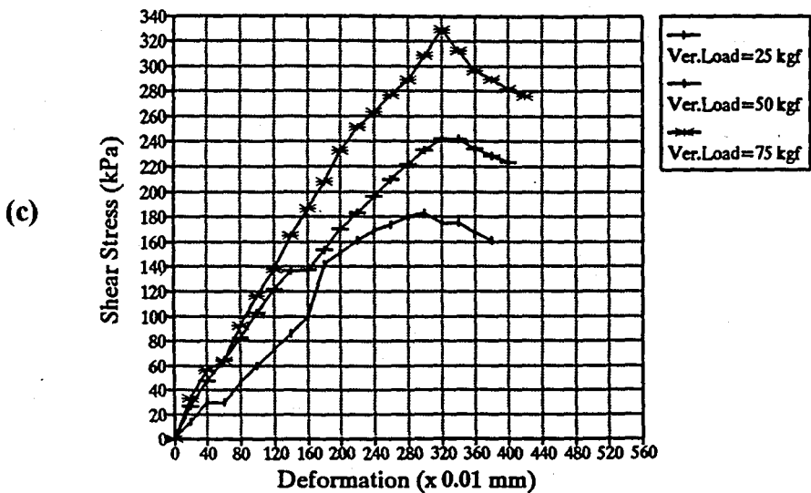
FIGURE A.4. Shear Strength vs deformation behavior of soil samples which is composed of 50% sand and 50% bent. a) with no lime, b) with 3% lime, c) with 7% lime
