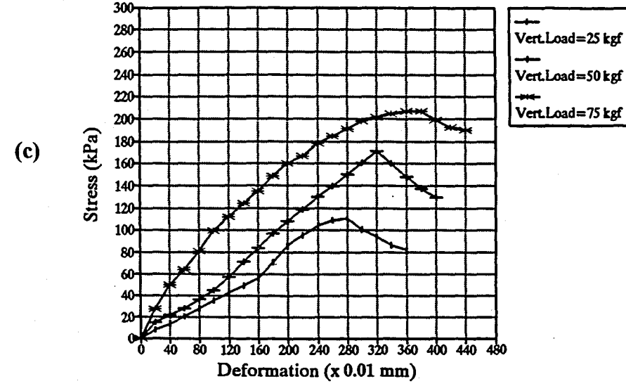
FIGURE A.13. Shear Strength vs deformation behavior of layered samples (soil sections: 30% sand and 70% bent.) a)with no lime, b)with 3% lime, c)with 7% lime
