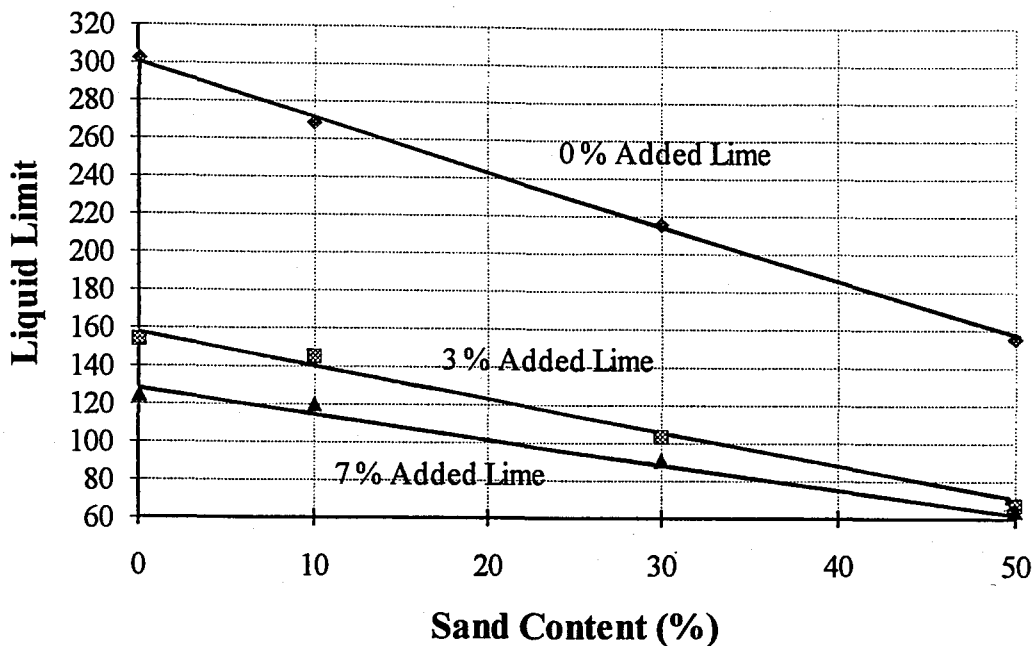
FIGURE 3.3. Liquid limit versus the sand amount in bentonite-sand mixture
