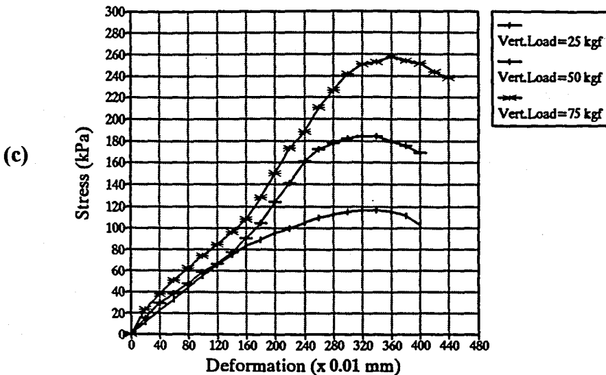
FIGURE A.16. Shear Strength vs deformation behavior of layered samples (soil sections: 50% sand and 50% bent.) a)with no lime, b)with 3% lime, c)with 7% lime
