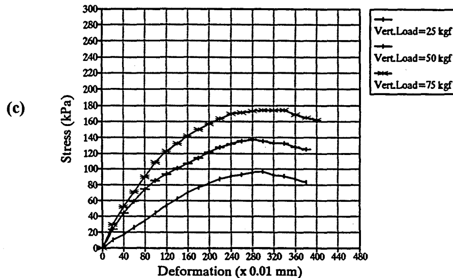
FIGURE A.9. Shear Strength vs deformation behavior of layered samples (soil sections: 100% bentonite) a) with no lime, b) with 3% lime, c) with 7% lime
