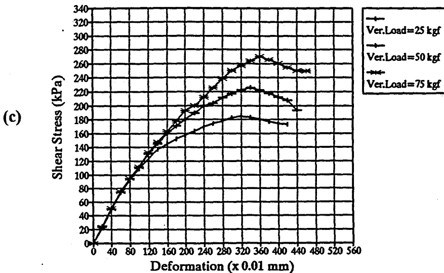
FIGURE A.2. Shear Strength vs deformation behavior of soil samples which is composed of 10% sand and 90% bentonite. a) with no lime, b) with 3% lime, c) with 7% lime
