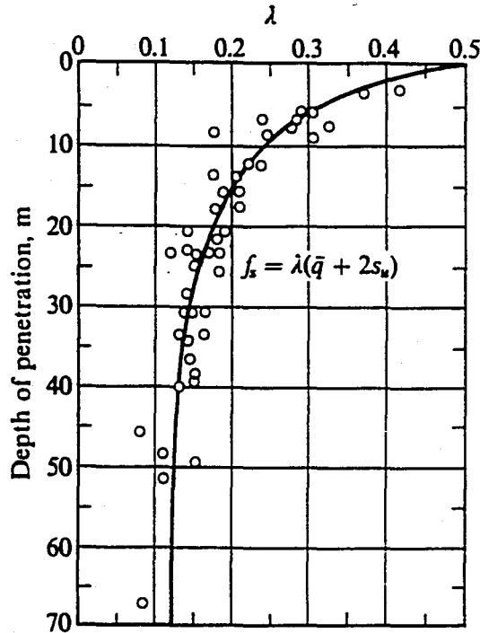
FIGURE 2.10. \lambda coefficients depending on pile penetration [35]
