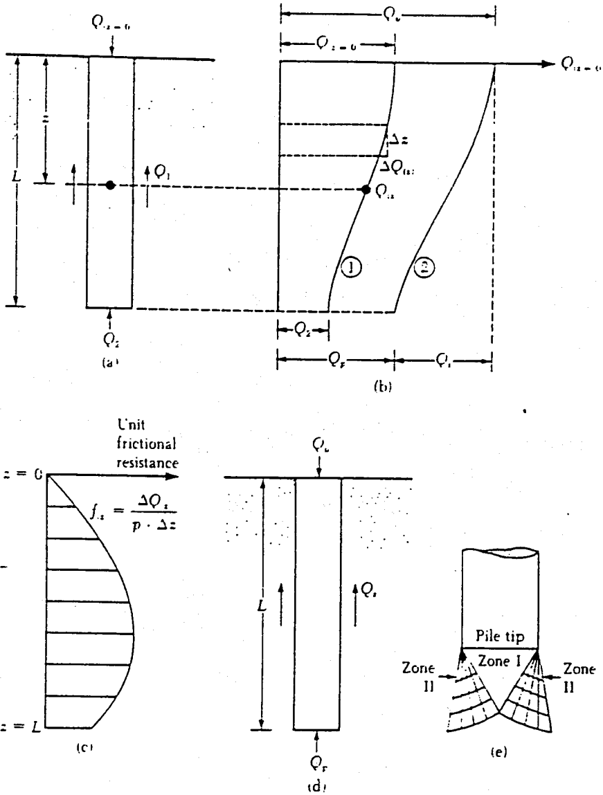
FIGURE 2.8. Load transfer Mechanism for Piles [33]
