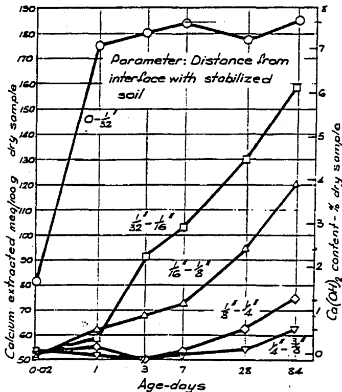
FIGURE 2.7. Diffusion of calcium into cores of lime stabilized (15 per cent) clayey lumps [28]
