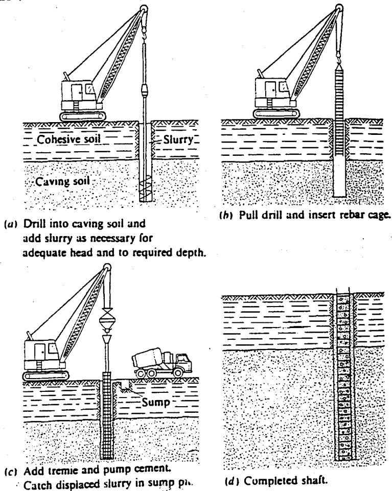
FIGURE 2.13. Slurry method of drilled pier construction [30]
