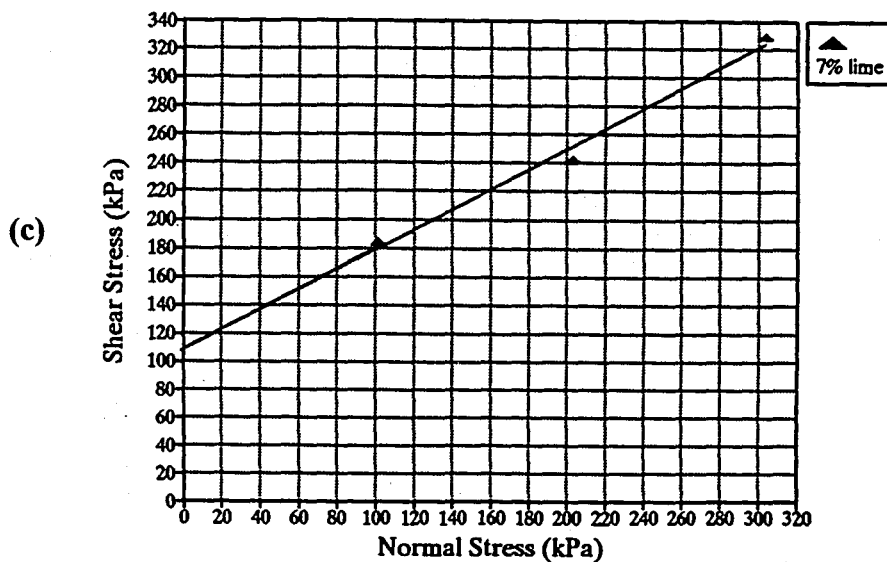
FIGURE A.5. Failure envelopes of soil samples which is composed of 100% bentonite a) with no lime, b) with 3% lime, c) with 7% lime
