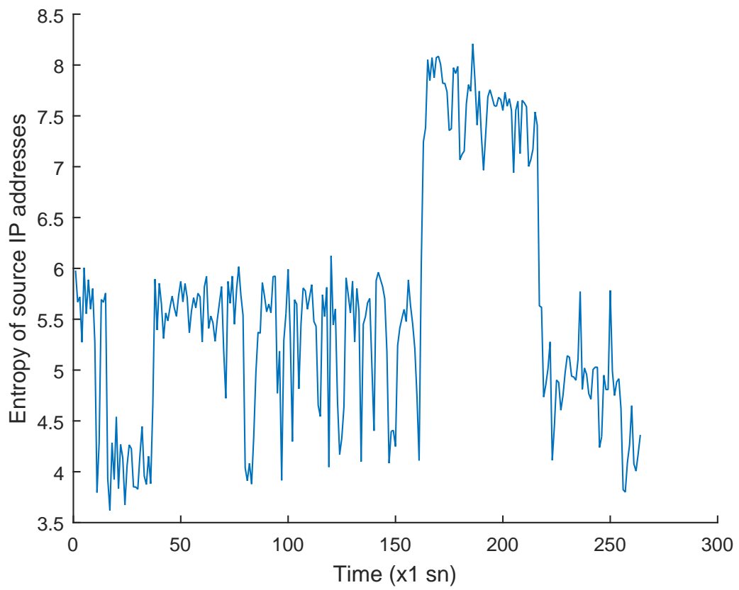
Figure 4.1. Entropy of source IP addresses for the attack maintains between 161-215 seconds.
