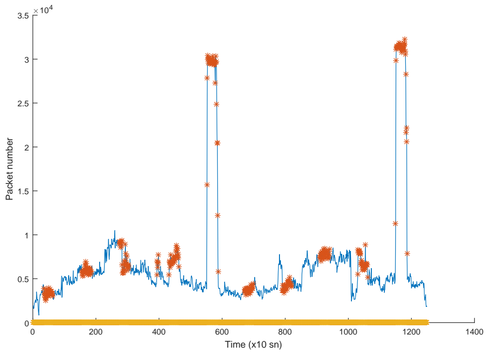
Figure 5.1. NUST TCP Syn flood dataset packet number (stars indicate attack exists in that time interval).
