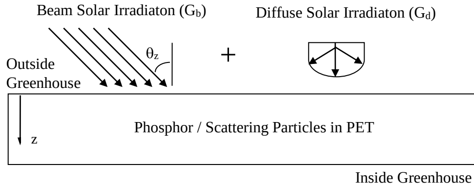
Figure 3.1. Sketch of the greenhouse coating for total solar irradiation.
