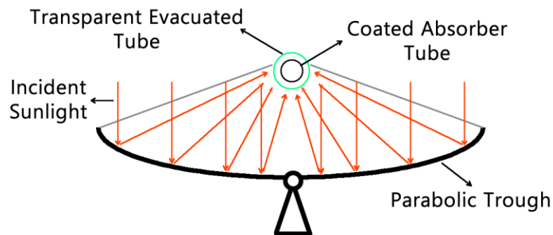
Figure 1.3. Parabolic through collector and its absorber tube
