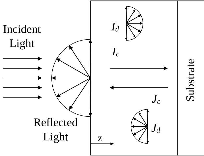
Figure 2.2. Sketch of the spectrally selective coating on a substrate.
