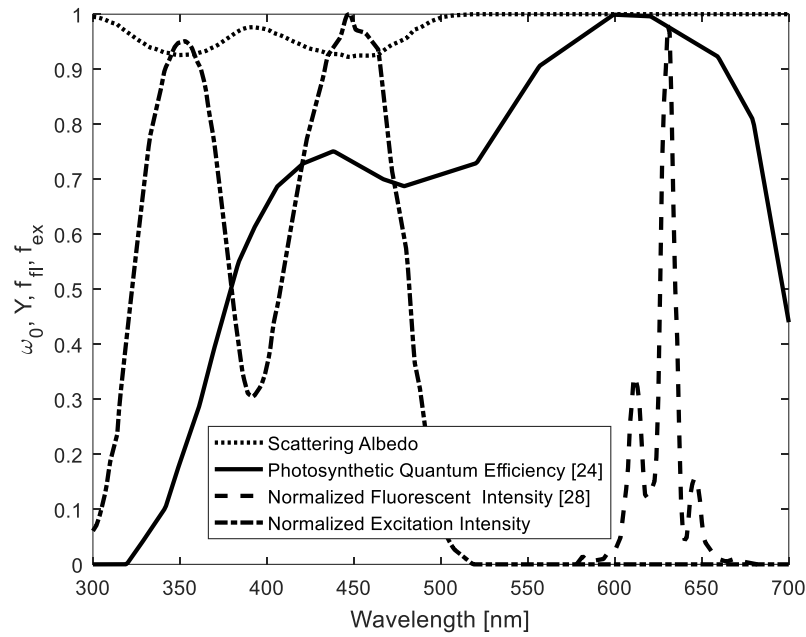
Figure 4.6. Excitation and emission [76] properties of \text{K}_2\text{SiF}_6:\text{Mn}^{4+} phosphor, photosynthetic quantum efficiency change of crop plants with respect to incident wavelength [73] and scattering albedo.
