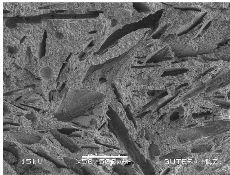
Figure 12.23 Scanning electron micrograph of %40 naphthalene added specimen implant ( secondary electron mode with magnification X50)
