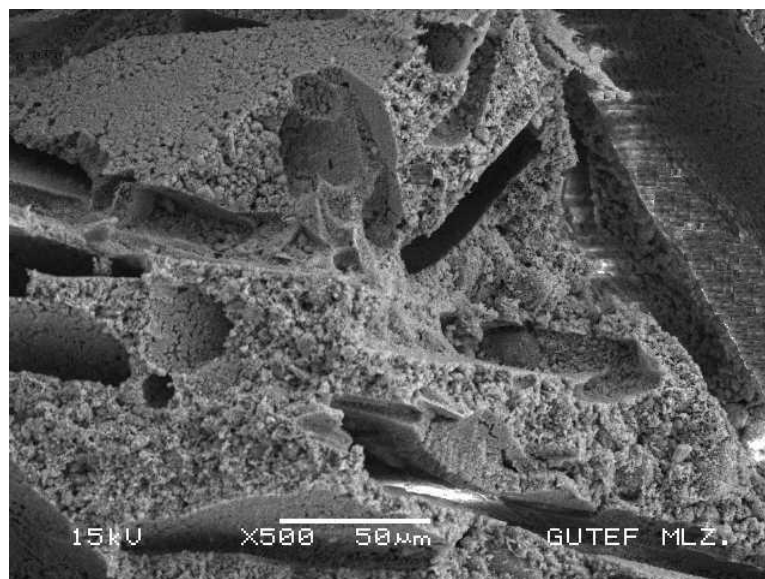
Figure 12.26 Scanning electron micrograph of %45 naphthalene added specimen implant ( secondary electron mode with magnification X500)
