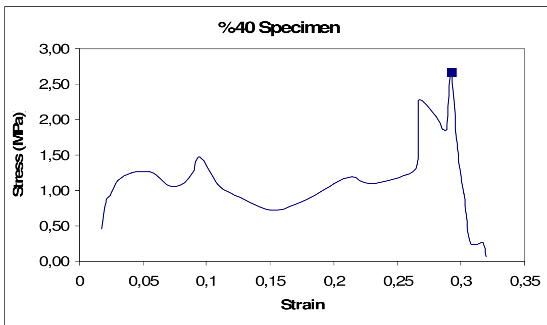
Figure 12.9 Stress versus strain graph of %40 naphthalene added cylindrical specimen.
