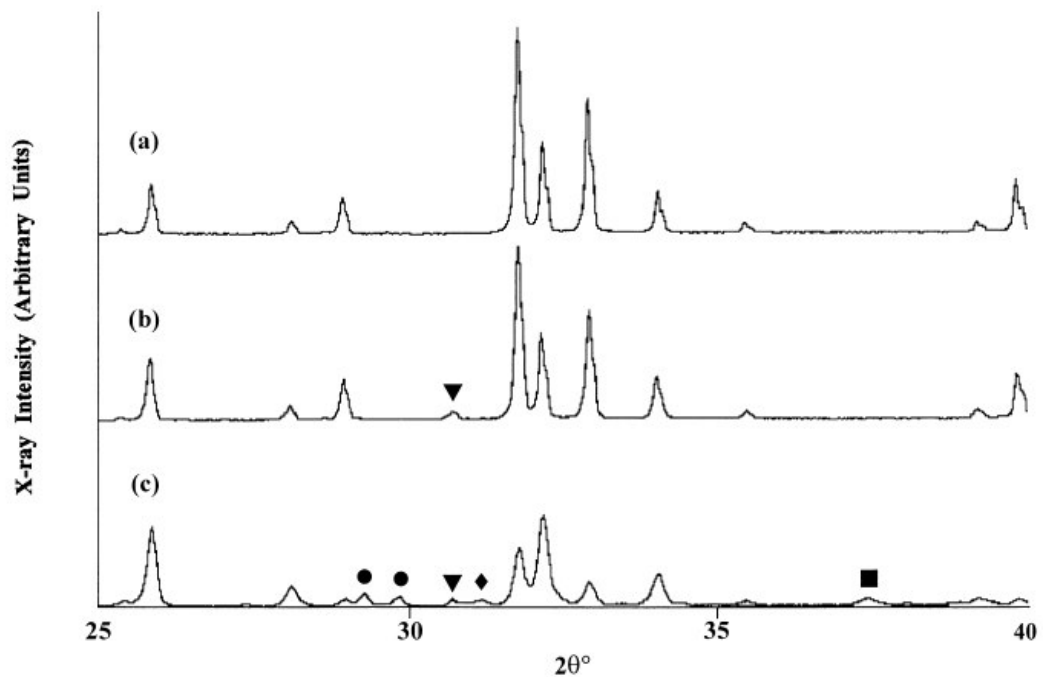
Figure 12.16 a) Normal XRD pattern of HAp b) Over critical temperature \alpha -TCP appears c) Further temperature increase result in the formation of \beta -TCP, TTCP and CaO (Key: ●= TTCP, ◆= \beta -TCP; ▼= \alpha -TCP and ■ =CaO) [71].
