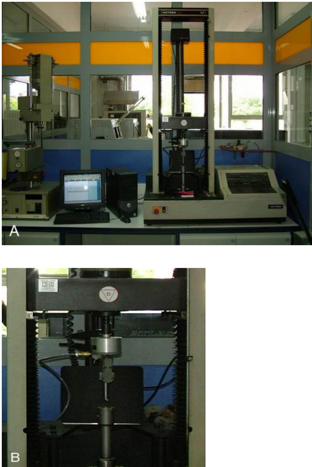
Figure 11.8 A. Specimen compression tests were carried out by using a servo-electrical universal testing system (Instron) B. Part of the compression test device on which the specimens placed and the force applied.
