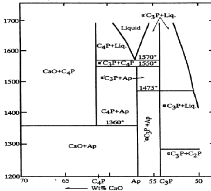
Figure 3.2 Phase diagram of the quasi-binary system CaO-P 2 O 5 -H 2 O at a water partial pressure of 65.5 kPa [4]
