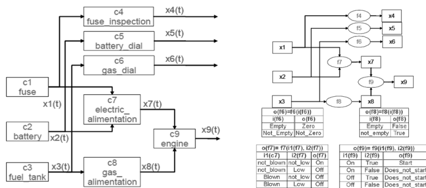
Fig. 5 The functional model of a car subsystem
