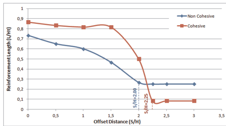
Figure 6.24. Influence of offset distance on the required reinforcement length to obtain a factor of safety equals to 1.5.
