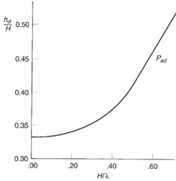
Figure 4.11. Location of dynamic thrust at instant of maximum overturning moment for k_h=0.2 (after Steedman and Zeng, 1990).
