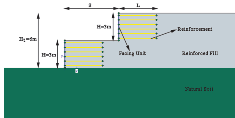
Figure 5.1. Tiered reinforced soil retaining wall.
