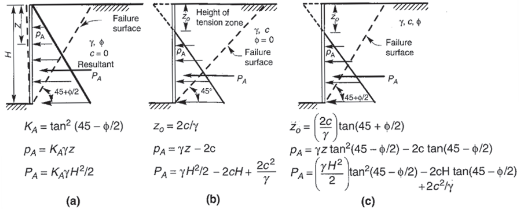
Figure 4.3. Minimum Rankine active earth pressure distributions for backfills with various combinations of frictional and cohesive strength: (a) frictional resistance, no cohesion; (b) cohesive soil, no frictional resistance; (c) combined cohesion and friction (Kramer, 1996).
