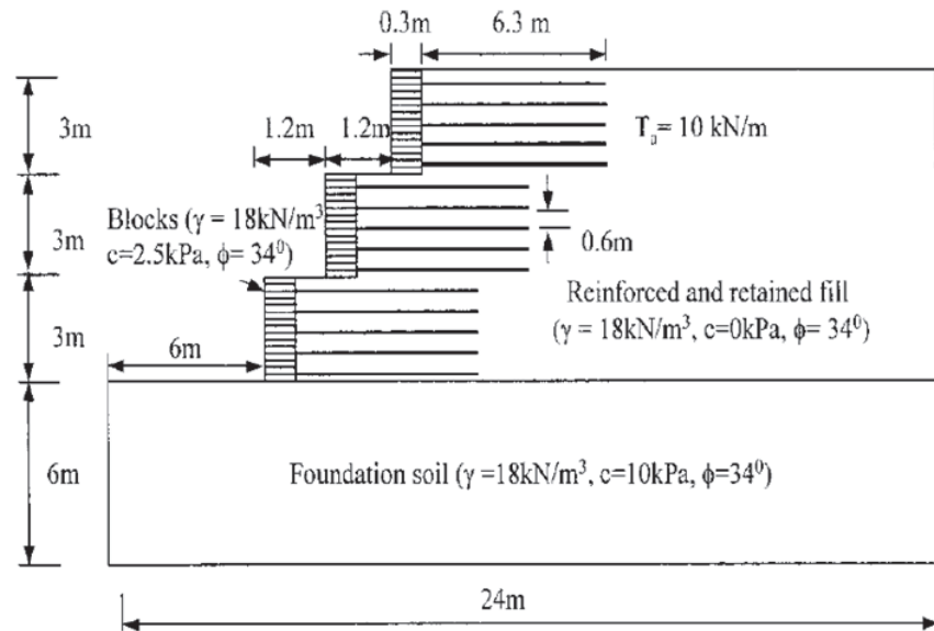
Figure 4.42. Baseline model for limit equilibrium and numerical analyses (Leshchinsky et al. , 2004).
