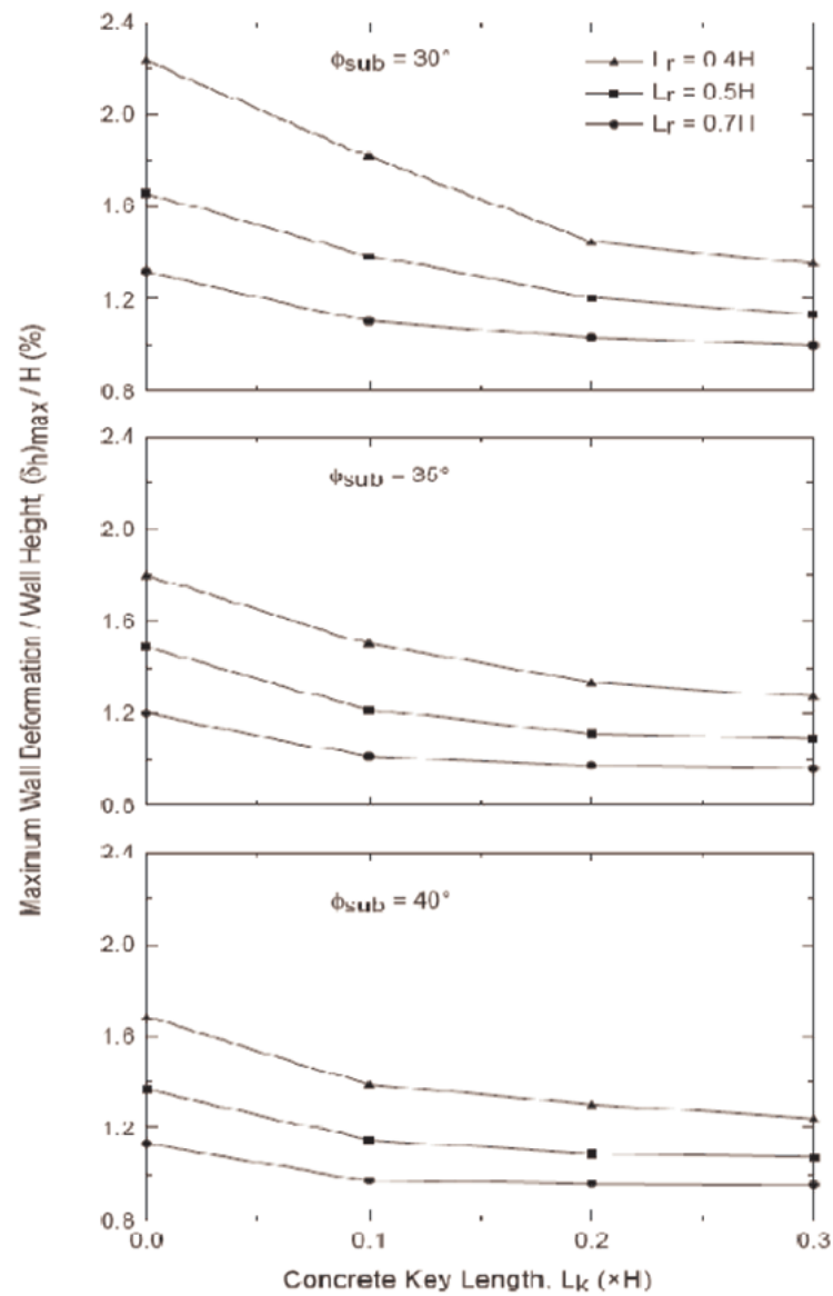
Figure 4.41. Effect of concrete key length on maximum wall deformations (Kim and Bilgin, 2007).
