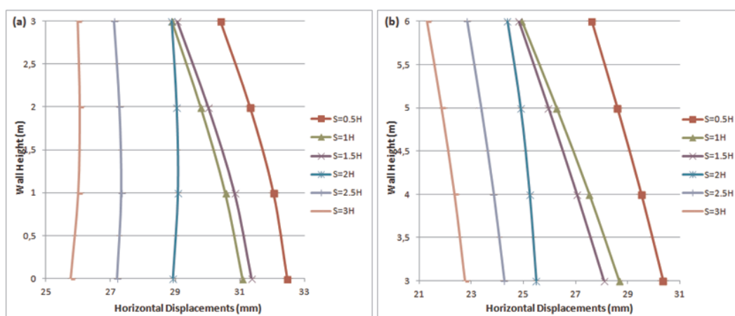
Figure 6.14. Permanent displacements with respect to offset distance for non cohesive soils and L=1.0H_t (a) Tier 1 (b) Tier 2.
