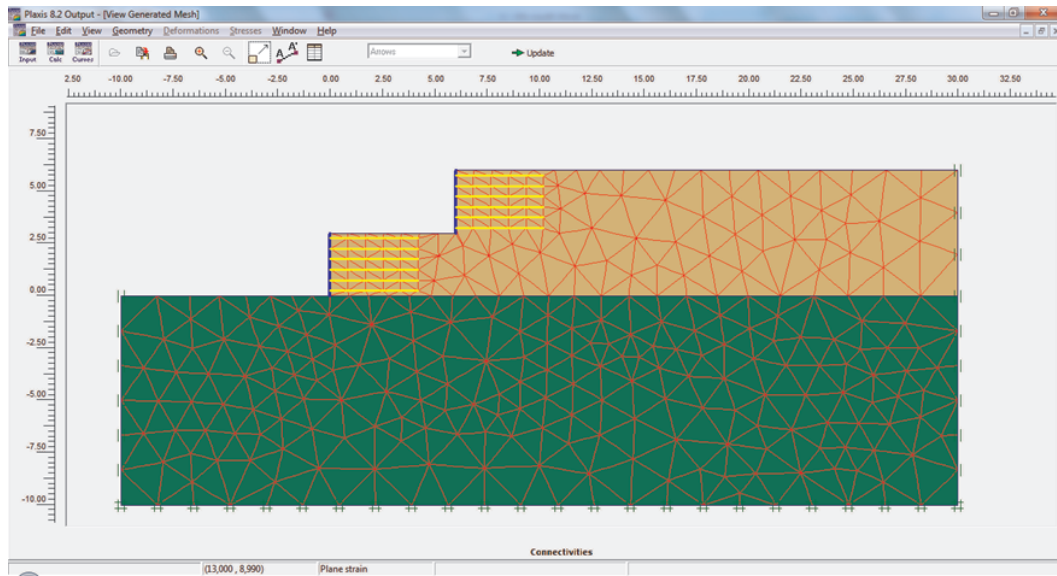
Figure 5.4. Finite element mesh of a model.
