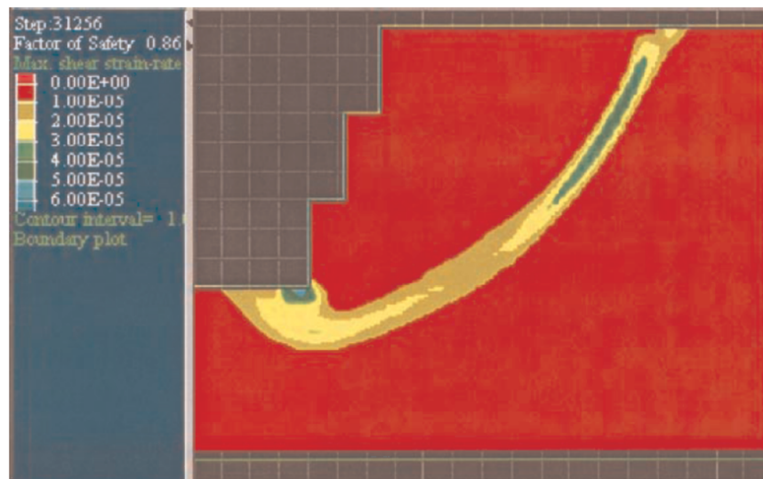
Figure 4.47. Bearing failure of multi-tiered mechanically stabilized earth wall in FLAC (Leshchinsky et al. , 2004).
