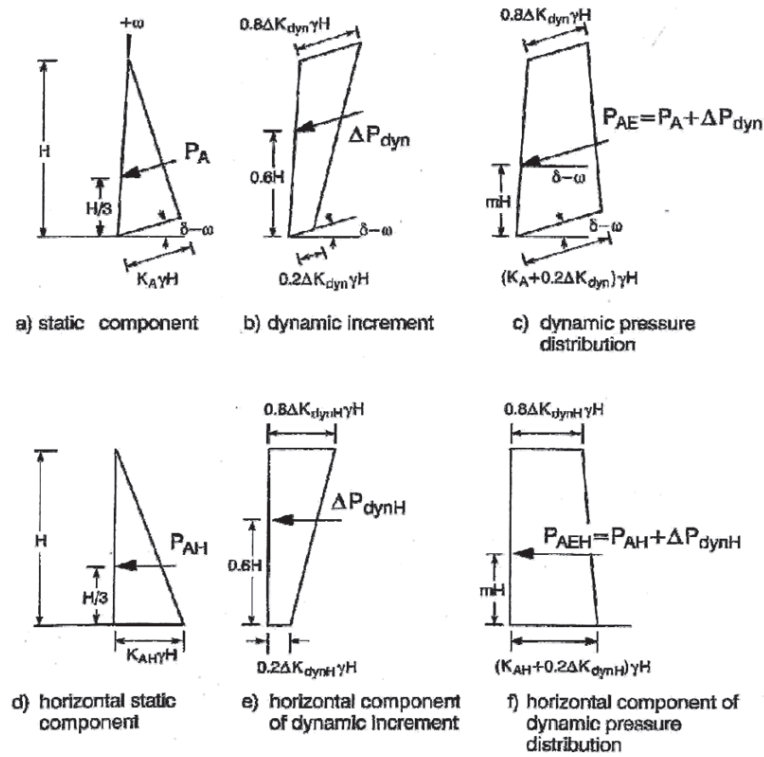
Figure 4.19. Earth pressure distributions due to soil self-weight.
