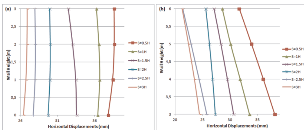
Figure 6.2. Permanent displacements with respect to offset distance for non cohesive soils and L=0.5H_t (a) Tier 1 (b) Tier 2.
