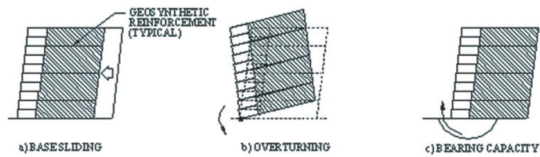
Figure 4.16. Potential external failure mechanisms of MSE wall.
