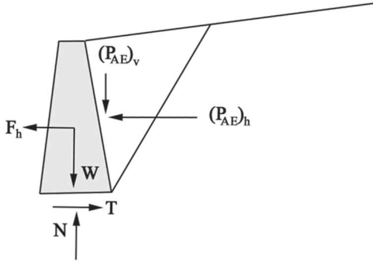
Figure 4.15. Gravity wall acted upon by gravity and pseudo-static accelerations.
