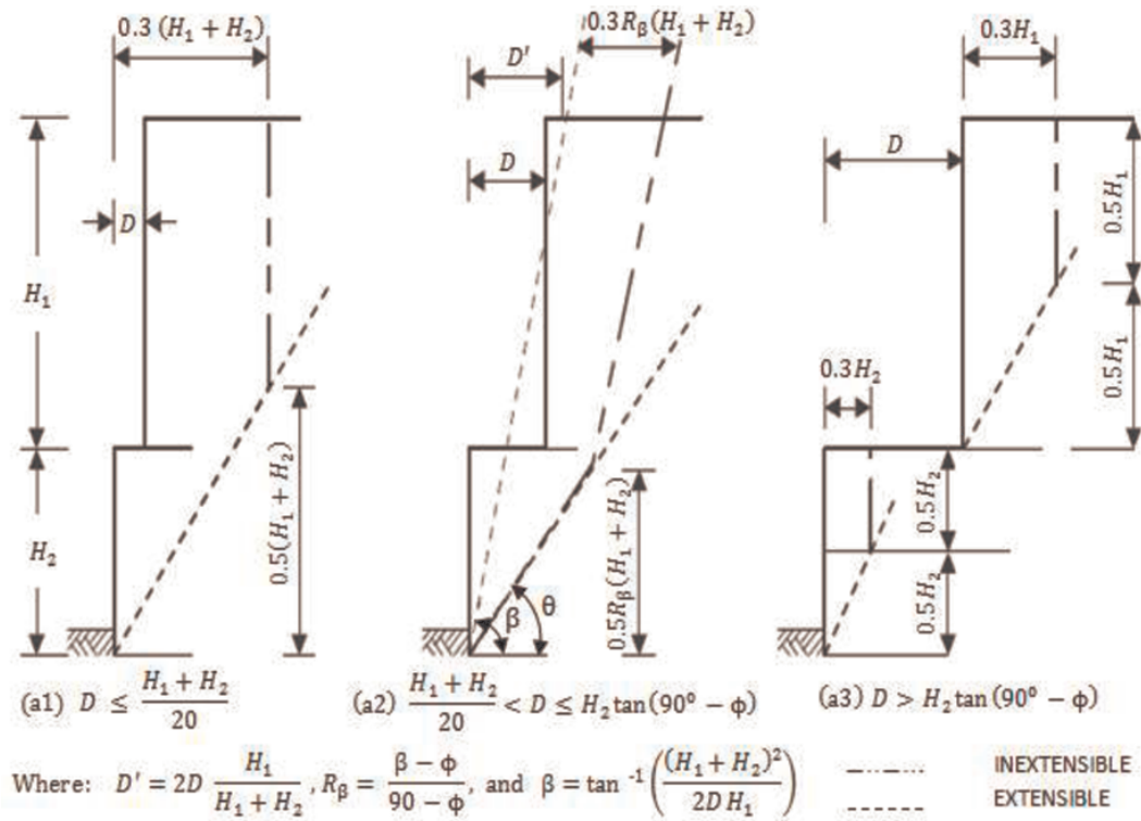
Figure 4.26. Maximum tension lines assumed in FHWA Guidelines (2009).
