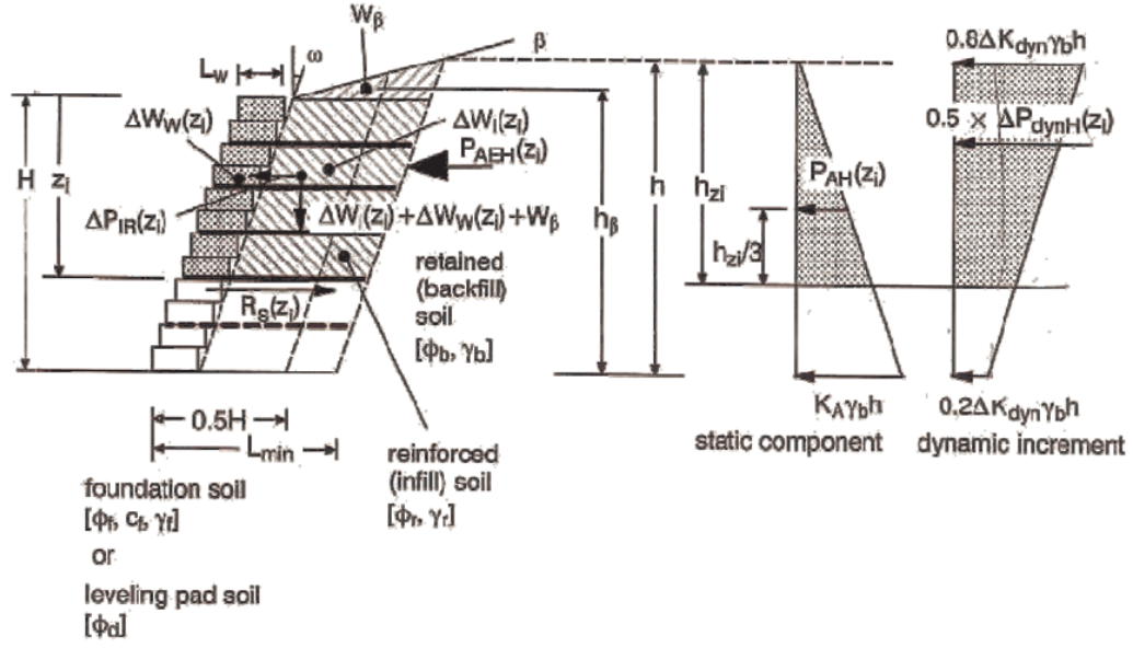
Figure 4.25. Geometry and forces used to calculate interface shear (bulging) and overturning of the facing column for reinforced SRW structures.
