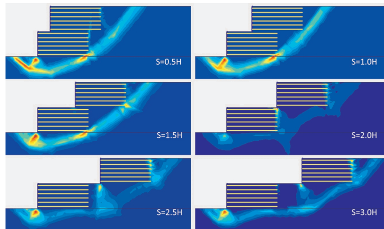
Figure 6.18. Failure surfaces for non cohesive fill.
