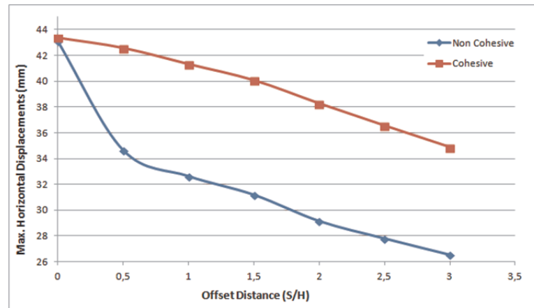
Figure 6.10. Factor of safety with respect to offset distance for L=0.7H_t .
