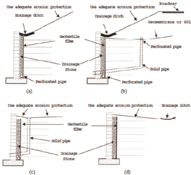
Figure 4.33. Drainage of run-off water at the top of a MSE wall using: (a) lined ditch directly behind the blocks; (b) low-permeability layer to catch infiltrating water; (c) drainage pipe at suitable intervals along the wall; (d) drainage away from wall face (Narejo and Ramsey, 2001).
