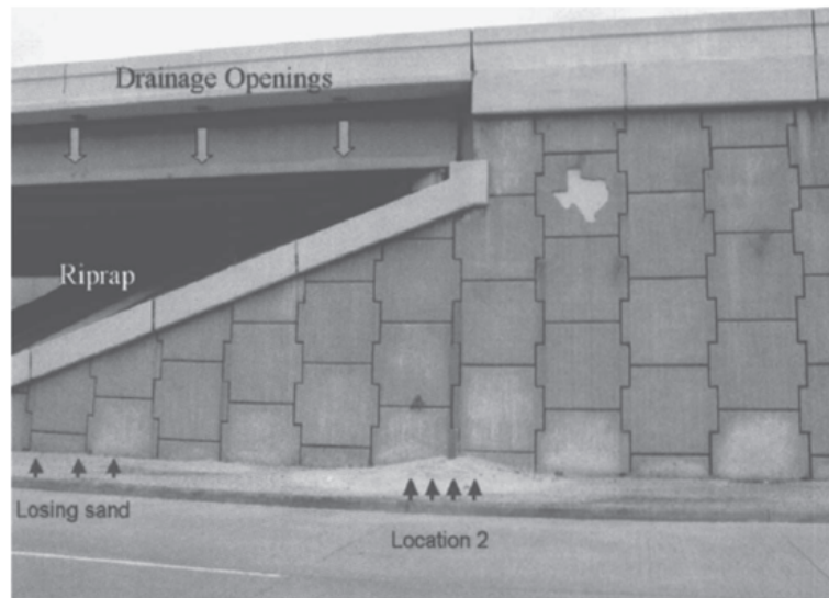
Figure 4.38. Drainage opening on bridge deck that permits water to fall straight through riprap joint (Chen et al. , 2007).
