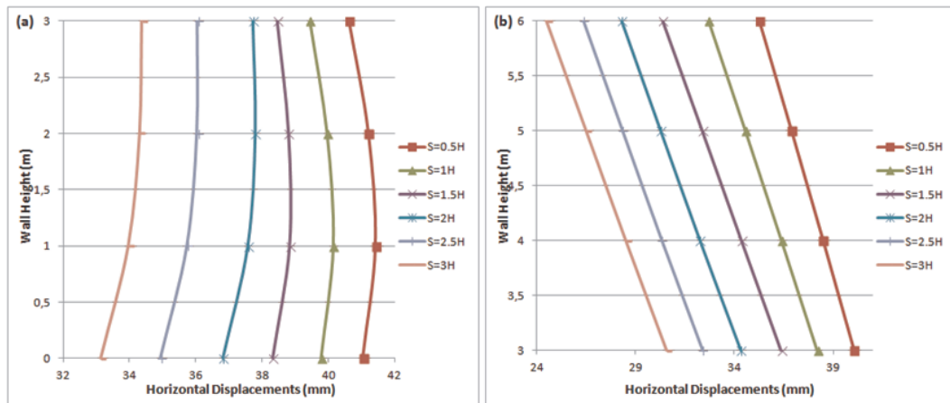
Figure 6.15. Permanent displacements with respect to offset distance for cohesive soils and L=1.0H_t (a) Tier 1 (b) Tier 2.
