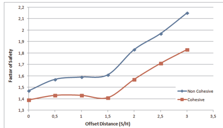
Figure 6.11. Factor of safety with respect to offset distance for L=0.7H_t .
