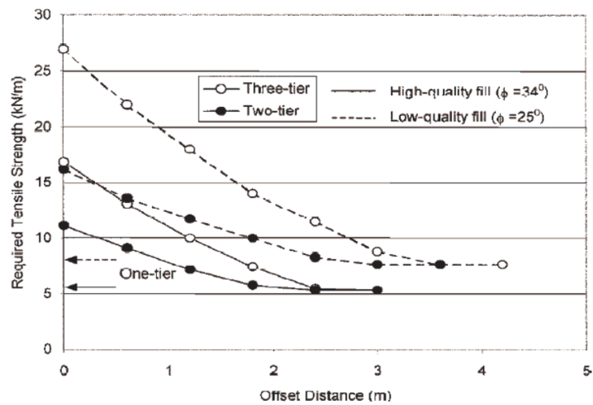
Figure 4.44. Effect of fill quality on required reinforcement strength (Leshchinsky et al. , 2004).
