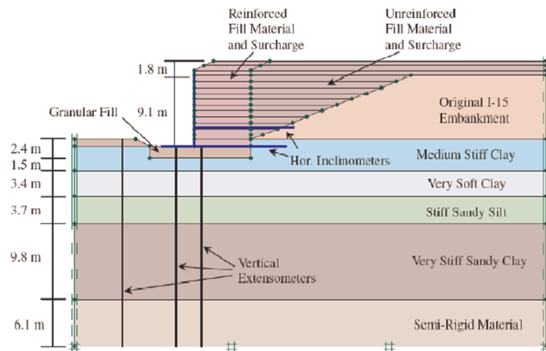
Figure 4.29. Soil profile and selected instrumentation for MSE wall on I-15 (Budge et al. , 2006).
