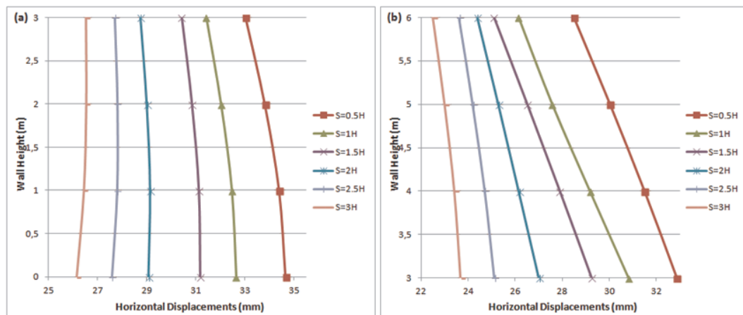
Figure 6.8. Permanent displacements with respect to offset distance for non cohesive soils and L=0.7H_t (a) Tier 1 (b) Tier 2.
