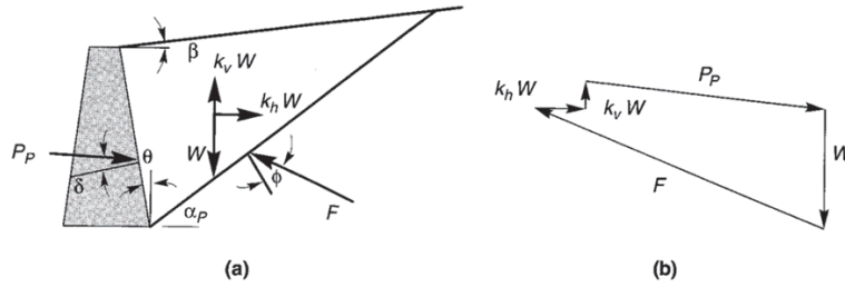
Figure 4.8. (a) Forces acting on passive wedge in Mononobe-Okabe analysis; (b) force polygon illustrating equilibrium of forces acting on passive wedge (Kramer, 1996).
