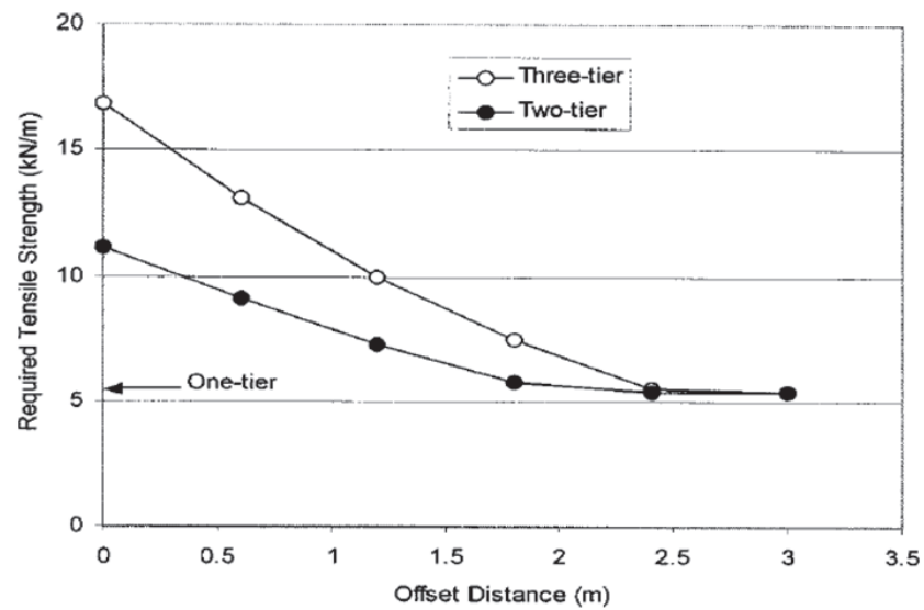
Figure 4.43. Effect of offset distance on required reinforcement strength (Leshchinsky et al. , 2004).
