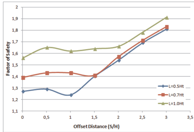
Figure 6.23. Factor of safety values for cohesive reinforced fill.
