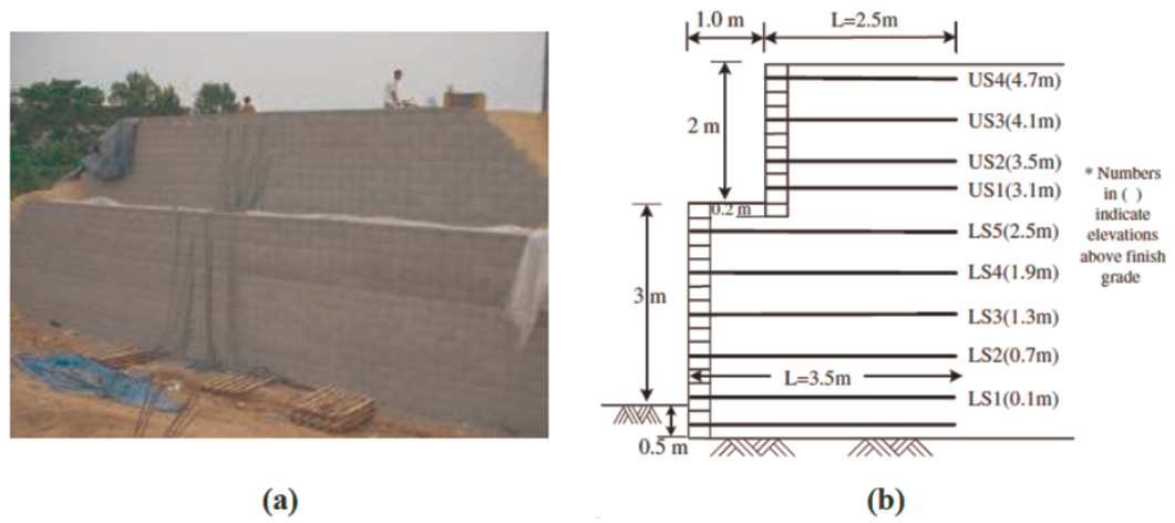
Figure 4.49. Test wall configuration: (a) photo of completed wall; (b) sectional view (Yoo and Kim, 2008).
