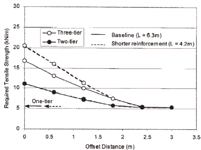
Figure 4.45. Effect of reinforcement length on required reinforcement Strength (Leshchinsky et al. , 2004).
