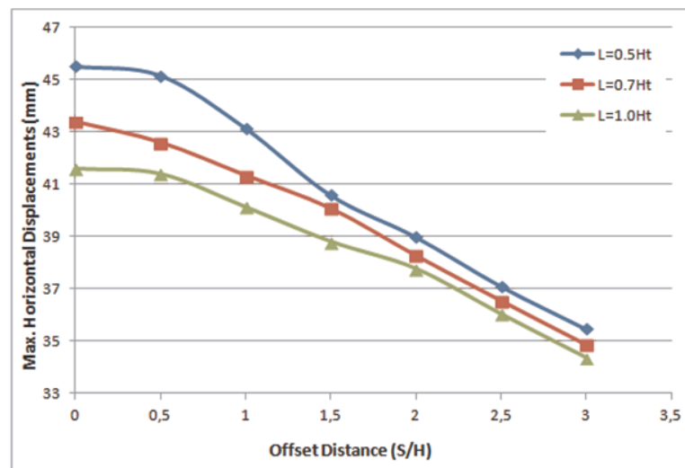
Figure 6.21. Maximum horizontal wall displacements for cohesive reinforced fill.
