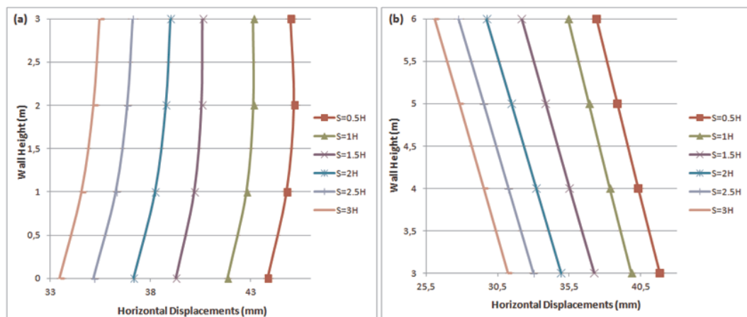
Figure 6.3. Permanent displacements with respect to offset distance for cohesive soils and L=0.5H_t (a) Tier 1 (b) Tier 2.
