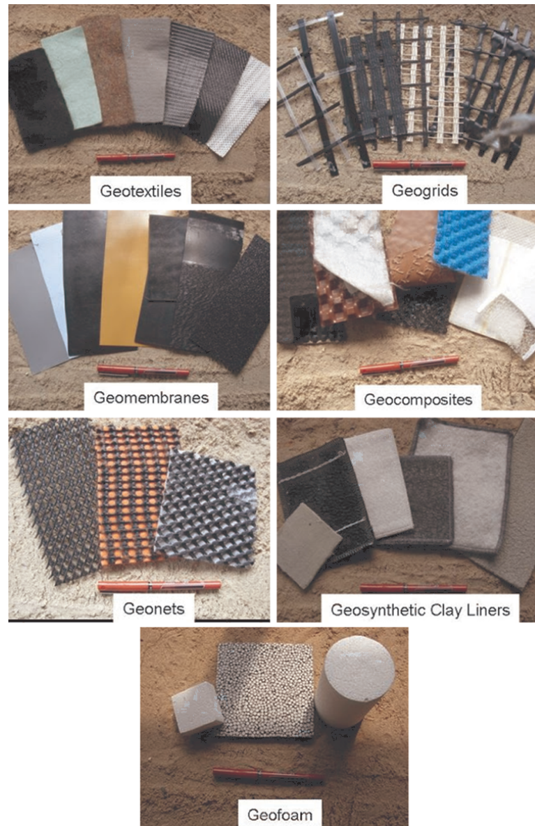
Figure 2.2. Typical Geosynthetic Materials.
