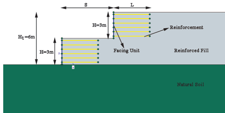
Figure 6.1. Multi tiered reinforced soil retaining wall.
