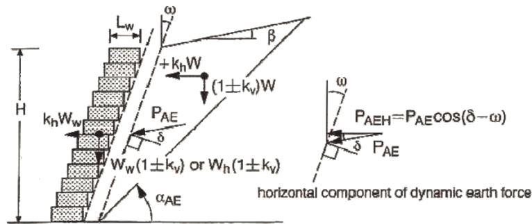
Figure 4.21. Resisting moments for base overturning in external stability calculations for reinforced SRW structures..
