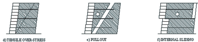
Figure 4.17. Potential internal failure mechanisms of MSE wall.
