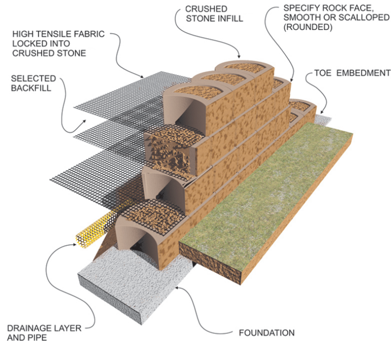
Figure 3.2. Schematic view of geosynthetic reinforced retaining wall (Terraforce, 2013).
