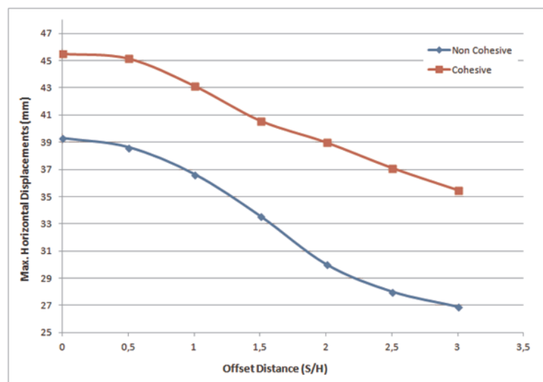
Figure 6.4. Maximum horizontal wall displacements with respect to offset distance for L=0.5H_t .
