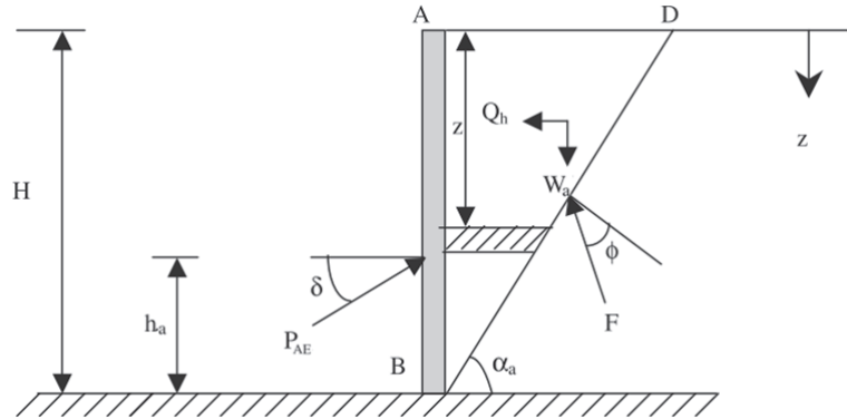
Figure 4.9. Model retaining wall considered for computation of pseudo dynamic active earth pressure (after Choudhury and Nimbalkar, 2006).
