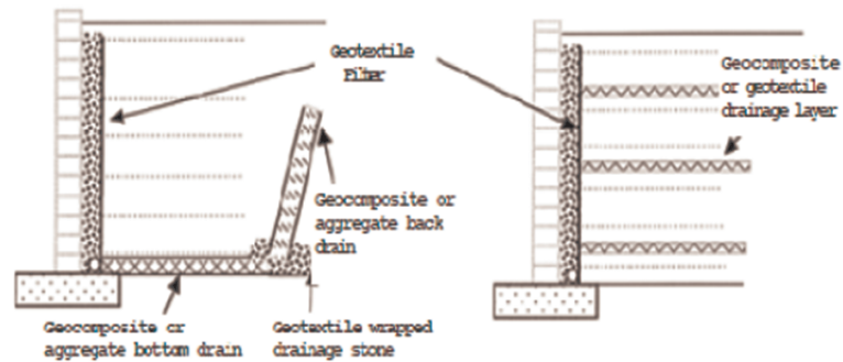
Figure 4.34. Drainage alternatives for seepage and infiltrating water: (a) chimney and bottom drains; (b) horizontal drains (Narejo and Ramsey, 2001).
