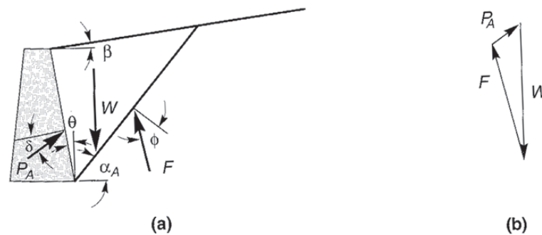
Figure 4.5. (a) Triangular active wedge bounded by planar backfill surface, failure surface and wall; (b) force polygon for active Coulomb wedge. The critical failure surface is that which gives the largest value of P_A (Kramer, 1996).
