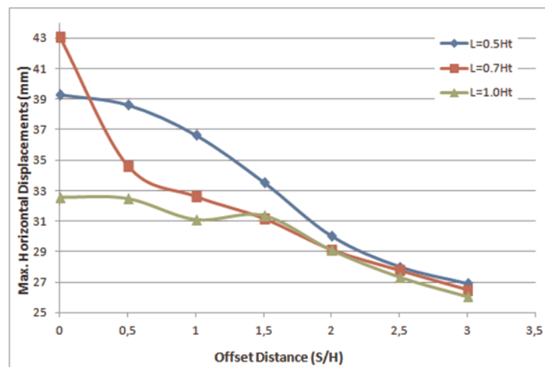
Figure 6.20. Maximum horizontal wall displacements for non cohesive reinforced fill.
