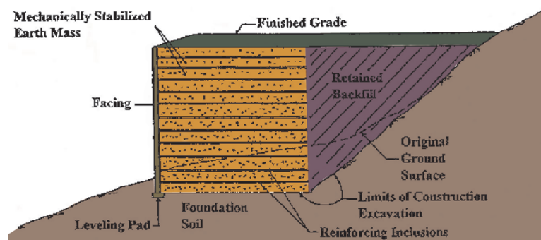
Figure 3.1. Generic cross-section of a MSE wall (Elias et al. , 2001).
