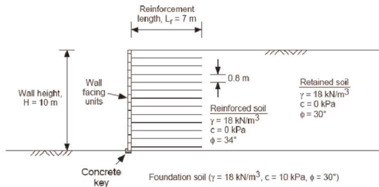
Figure 4.39. Baseline model of MSE wall for numerical analysis (Kim and Bilgin, 2007).
