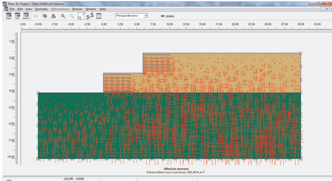
Figure 5.5. Initial conditions of a model.
