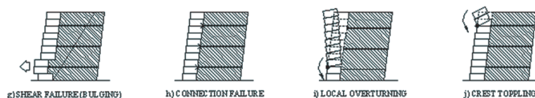
Figure 4.18. Potential facing failure mechanisms of MSE wall.
