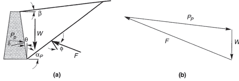
Figure 4.6. (a) Triangular passive wedge bounded by planar backfill surface, failure surface and wall; (b) force polygon for passive Coulomb wedge. The critical failure surface is that which gives the largest value of P_P (Kramer, 1996).
