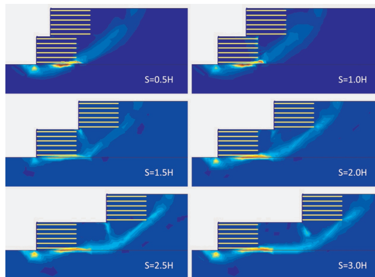
Figure 6.13. Failure surfaces for cohesive fill.
