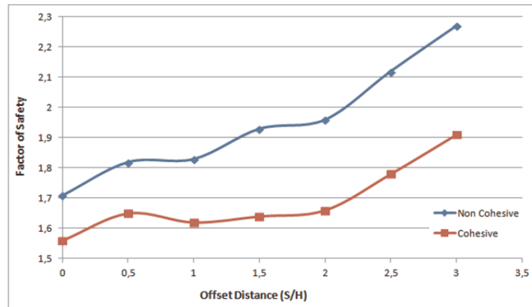
Figure 6.17. Factor of safety with respect to offset distance for L=1.0H_t .
