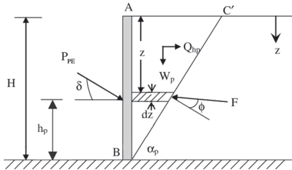
Figure 4.12. Model retaining wall considered for computation of pseudo dynamic active earth pressure (after Choudhury et al. , 2006).
