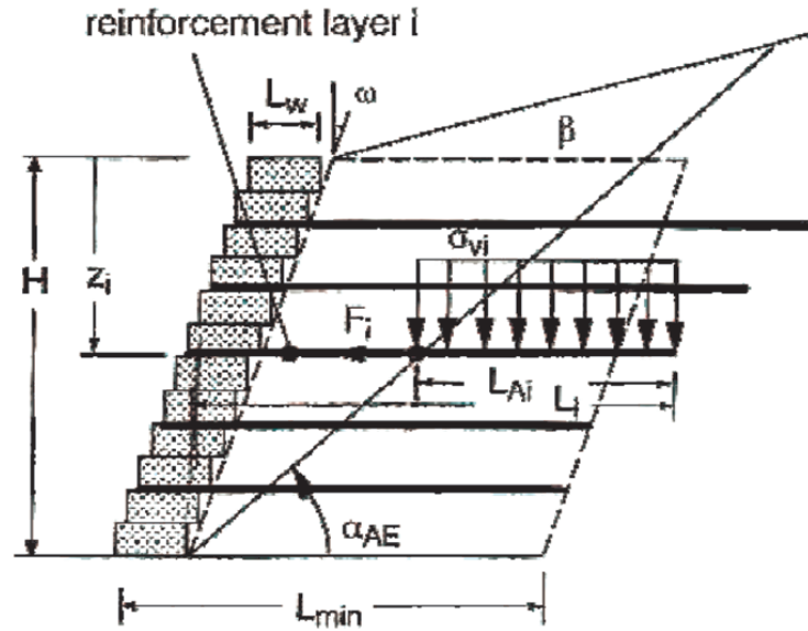
Figure 4.23. Geometry and forces used to calculate anchorage capacity of reinforcement layers in SRW structures.
