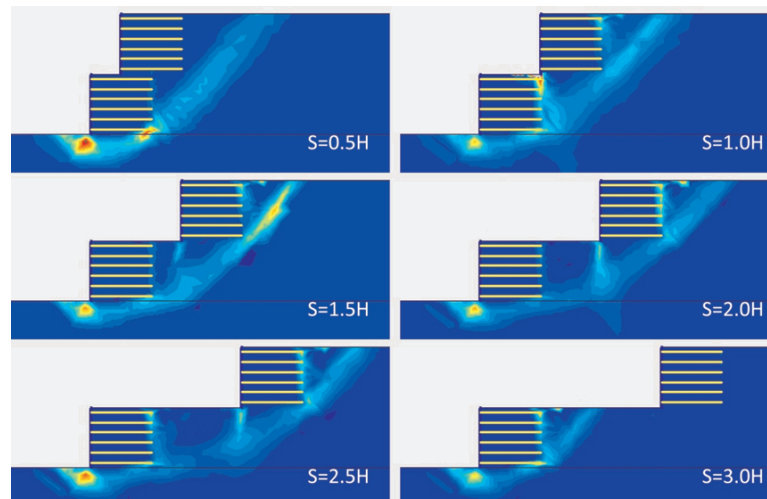
Figure 6.6. Failure surfaces for non cohesive fill.
