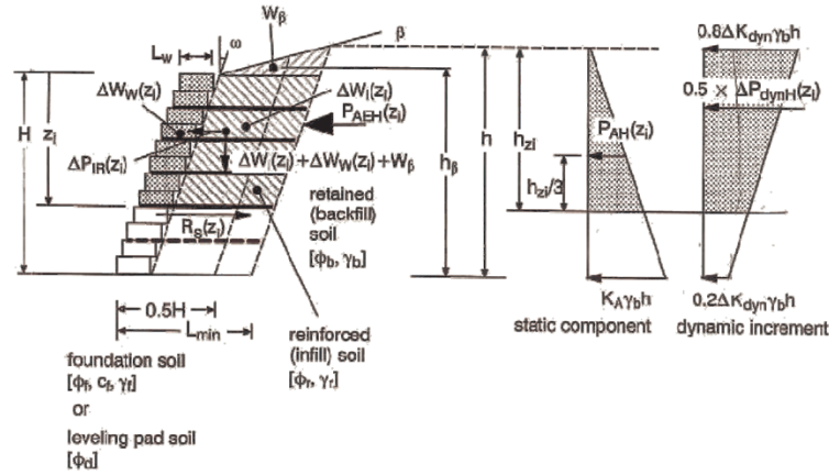
Figure 4.24. Geometry and forces used to calculate internal sliding of reinforcement layers in SRW structures.
