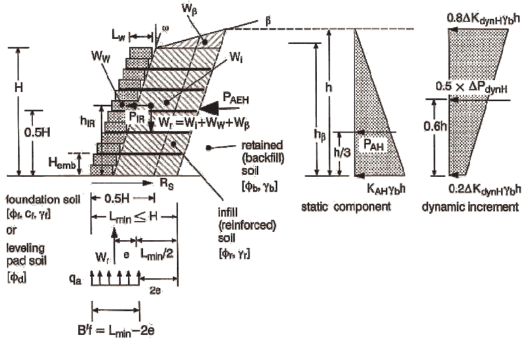
Figure 4.20. Earth pressure distributions due to soil self-weight.
