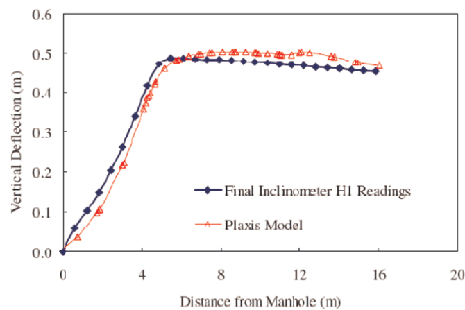
Figure 4.31. Comparison of horizontal inclinometer data to PLAXIS model data (Budge et al. , 2006).
