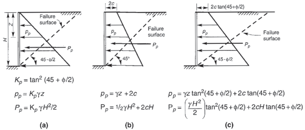
Figure 4.4. Maximum Rankine passive earth pressure distributions for backfills with various combinations of frictional and cohesive strength: (a) frictional resistance, no cohesion; (b) cohesive soil, no frictional resistance; (c) combined cohesion and friction (Kramer, 1996).
