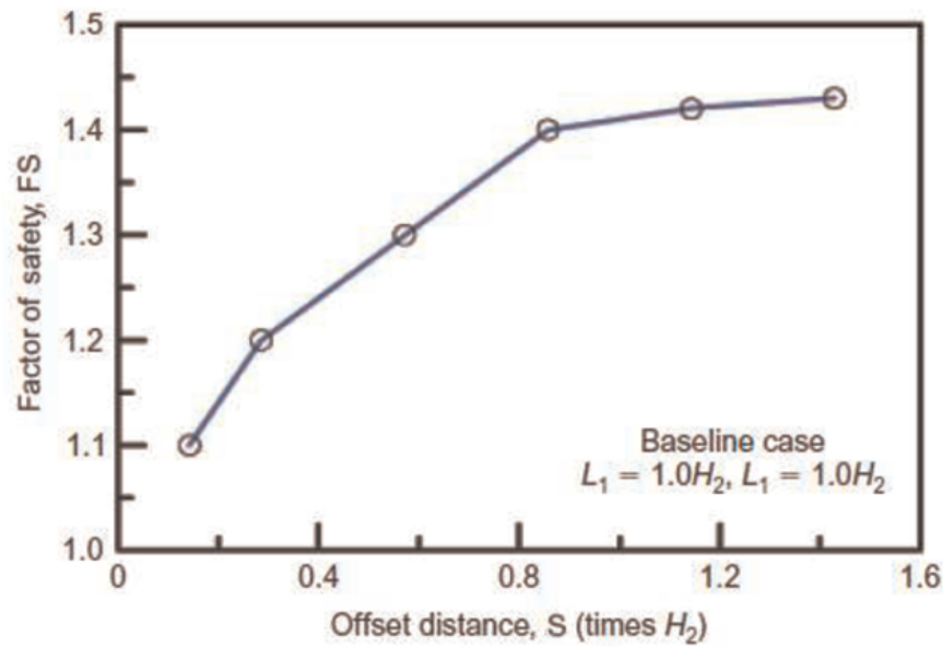
Figure 4.48. Variation of FS with offset distance S (Yoo et al. , 2011).
