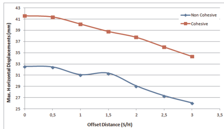
Figure 6.16. Maximum horizontal wall displacements with respect to offset distance for L=1.0H_t .
