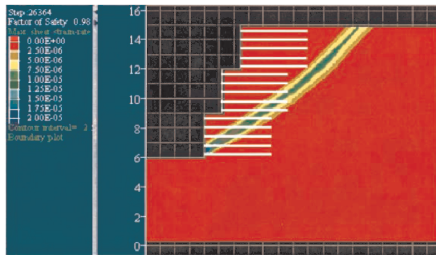
Figure 4.46. Critical surfaces for short reinforcement in FLAC, Predicted shear zone superimposed over reinforcement layout (Leshchinsky et al. , 2004).
