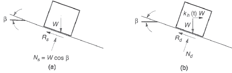
Figure 4.14. Forces acting on a block resting on an inclined plane: (a) static conditions, (b) dynamic conditions.
