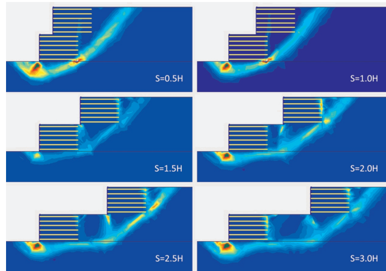
Figure 6.12. Failure surfaces for non cohesive fill.
