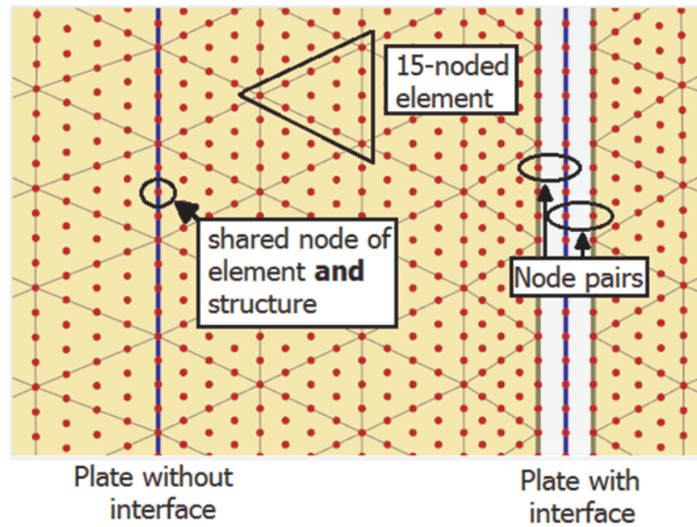
Figure 5.3. Interface elements used in models.
