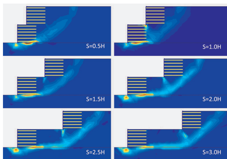
Figure 6.7. Failure surfaces for cohesive fill.
