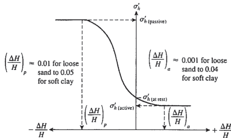
Figure 4.2. Nature of variation of lateral earth pressure at a certain depth (Das, 2007).
