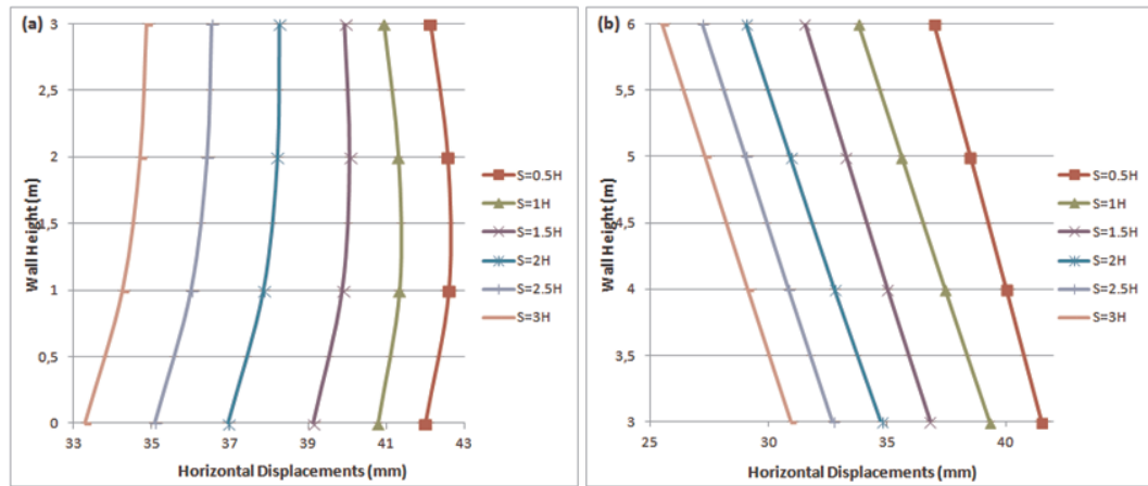
Figure 6.9. Permanent displacements with respect to offset distance for cohesive soils and L=0.7H_t (a) Tier 1 (b) Tier 2.
