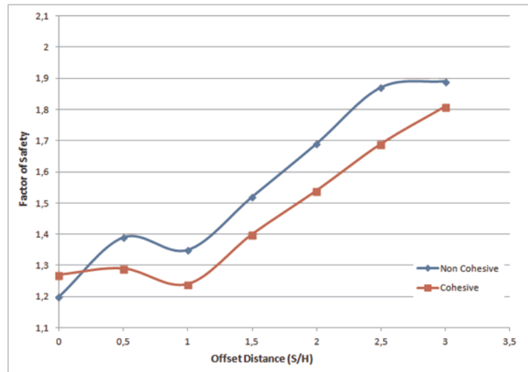
Figure 6.5. Factor of safety with respect to offset distance for L=0.5H_t .
