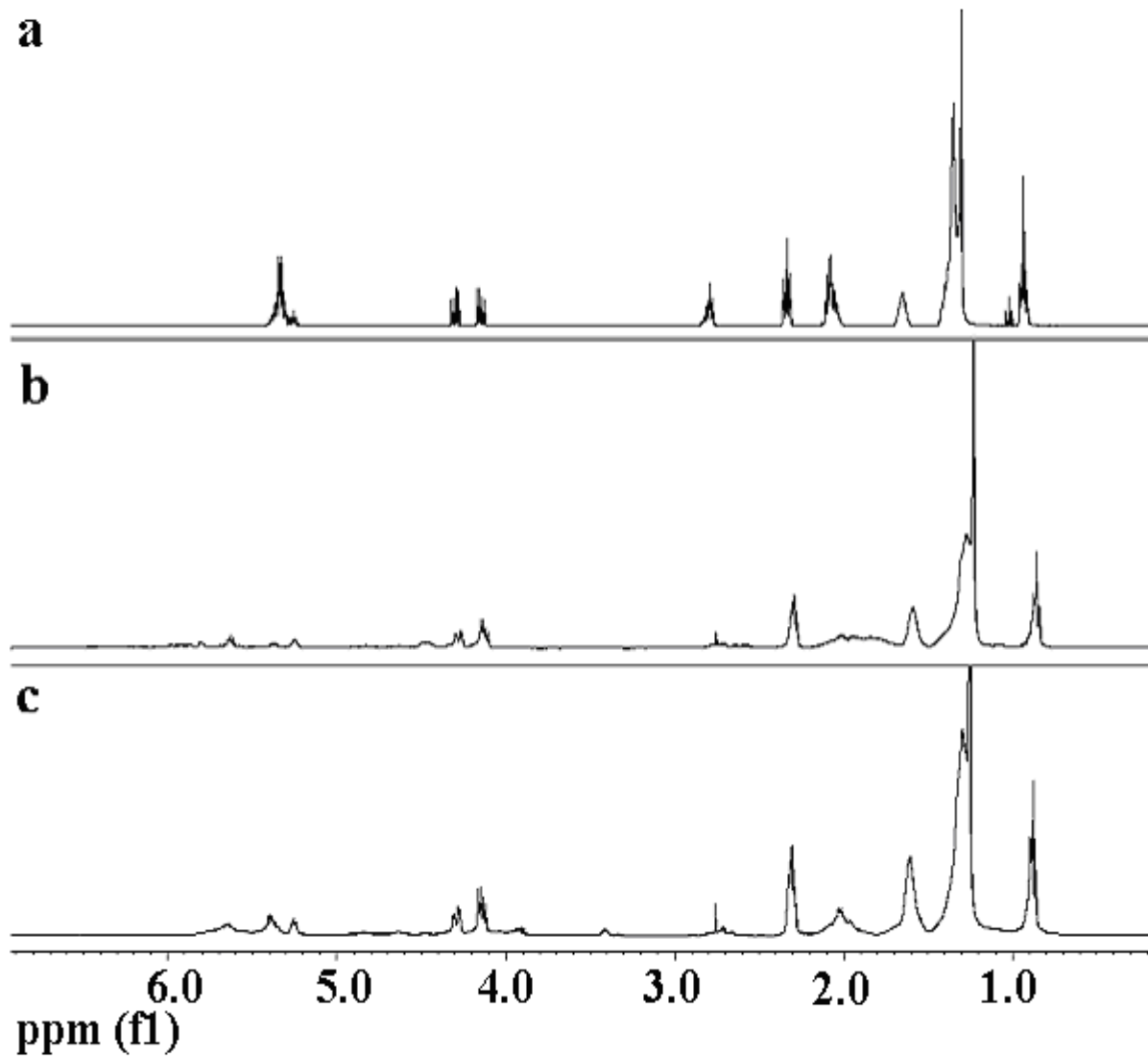
Figure 3.41. ^1\text{H} NMR spectrum of a-) Soybean oil b-) Allylic brominated soybean oil c-) Isocyanated soybean oil (SONCO)
