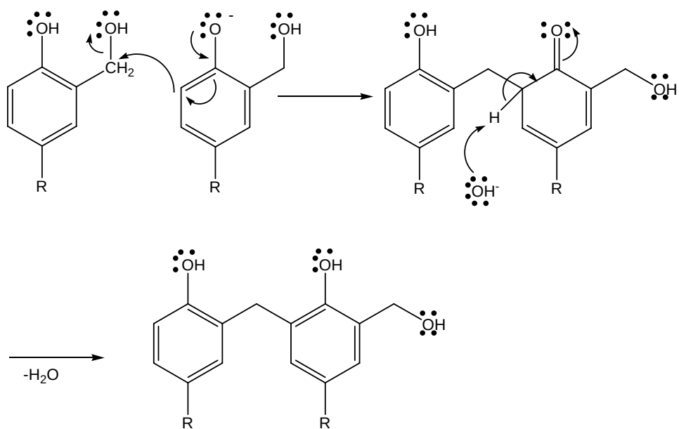
Figure 1. 16. Self condensation reaction of monomethylol phenol resoles.
