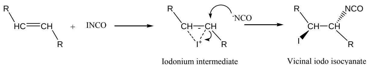
Figure 1. 7. Addition of iodo isocyanate to olefinic double bond
