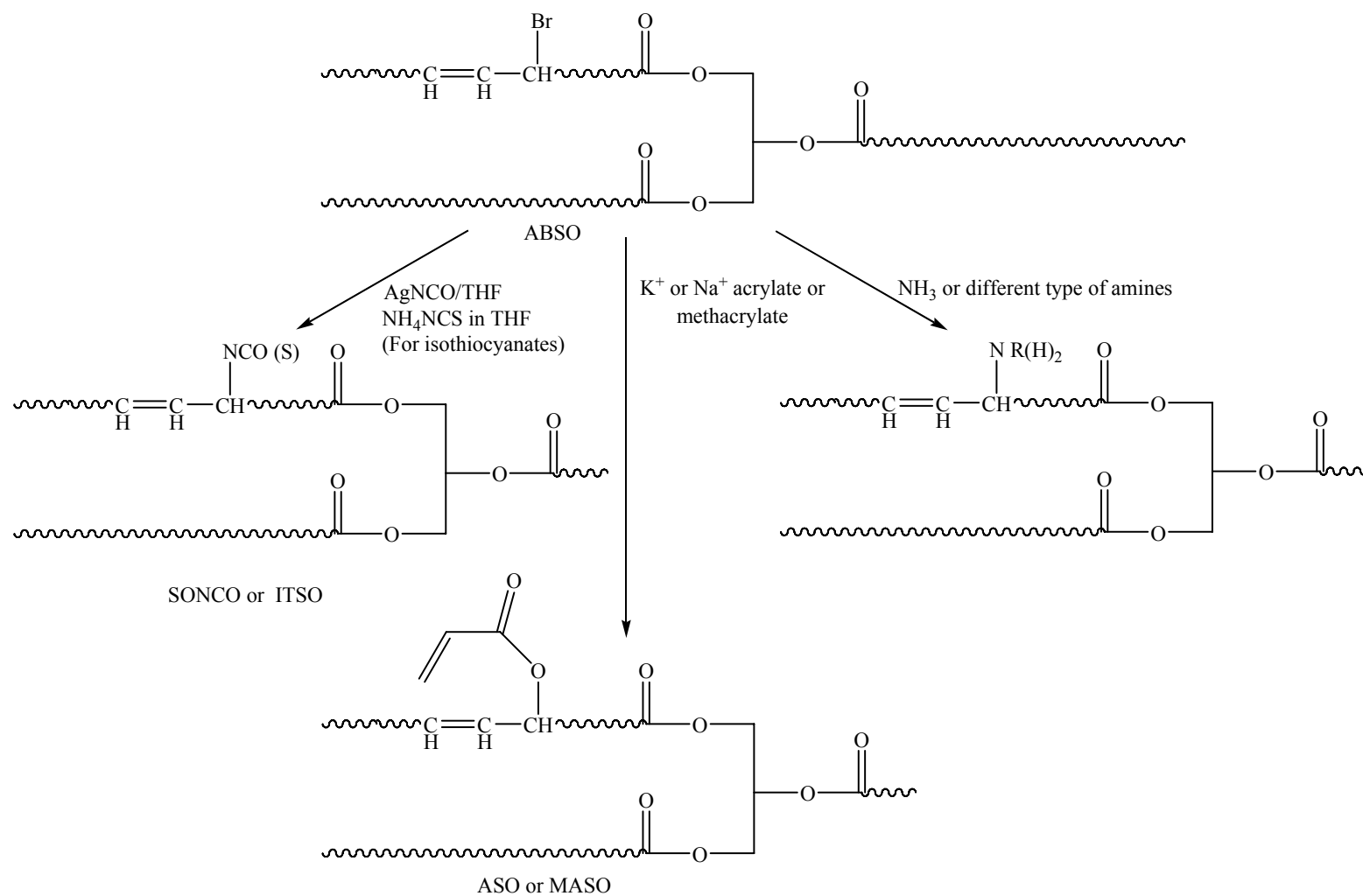
Figure 2.4. Substitution reaction of ABSO with different type of nucleophiles.
