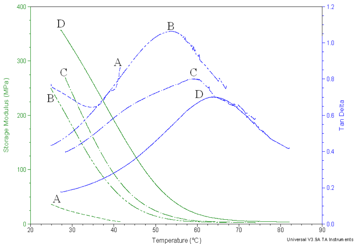
Figure 3.19. Storage modulus and \tan \delta values of polymers of linseed oil with 40 per cent (A) PTIOP (B) PTBP (C) PPP (D) PEP resoles.
