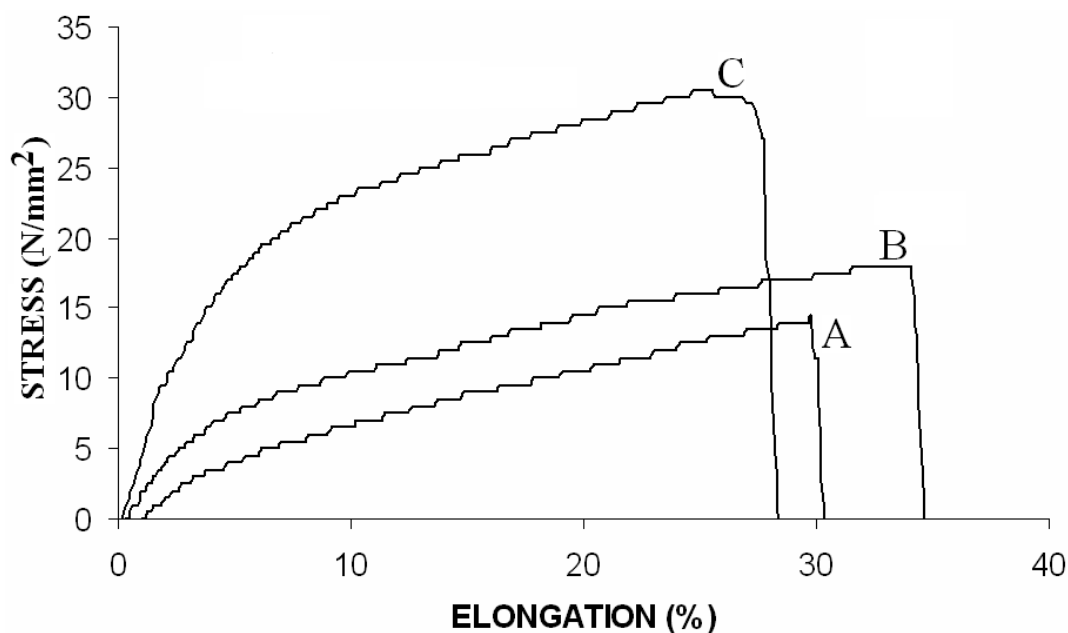
Figure 3.15. . Stress-Elongation curves of the polymers of linseed oil with (A) 10 per cent, (B) 20 per cent, (C) 30 per cent of p . phenyl phenol resole after 24 hours curing.
