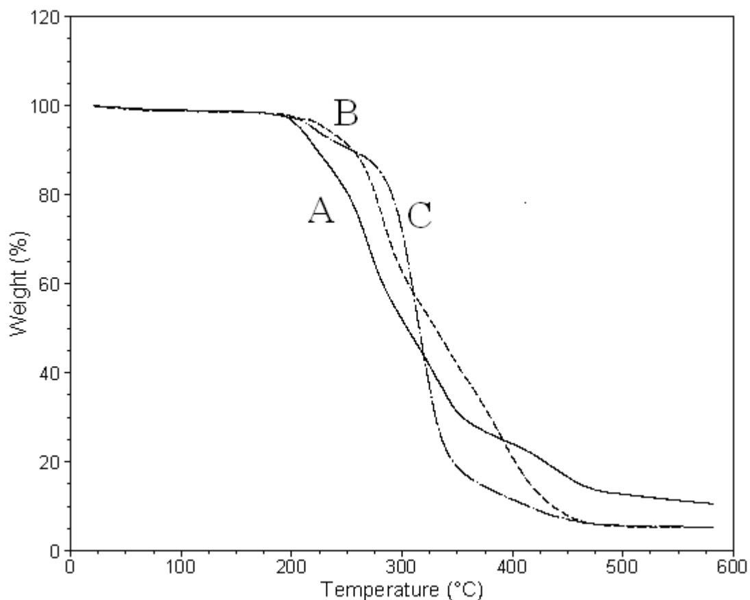
Figure 3.55. TGA curves of polyureas of ISONCO with (A) ethylene diamine (B) hexamethylene diamine (C) triethylene tetraamine.
