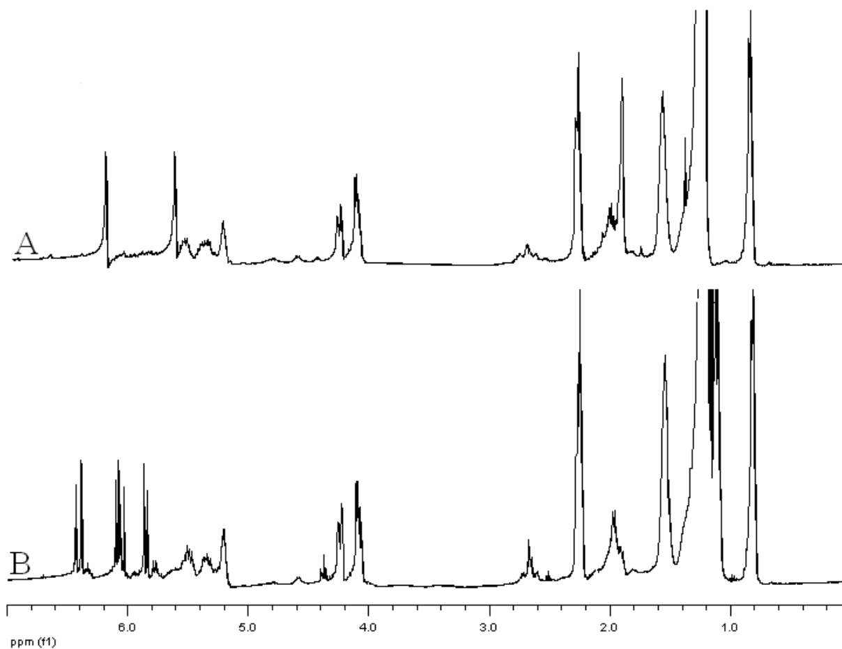
Figure 3.72. ^1\text{H} NMR spectra of (A) Allylicmethacrylate of soybean oil (MACSO) and (B) Allylicacrylate of soybean oil (ACSO)
