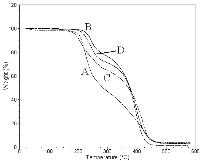
Figure 3.74. TGA traces of (A) homopolymers of allylic methacrylates of methyl oleate (ACMO) and (B) n butyl acrylate (C) methacrylic acid and (D) styrene copolymers
