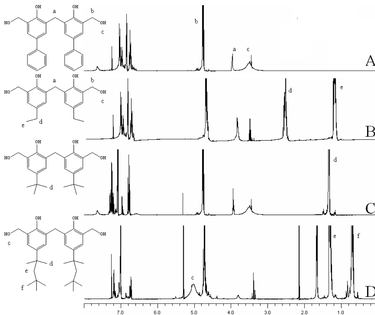
Figure 3.9. ^1\text{H} NMR spectra of (a) p. Phenyl phenol (b) p. Ethyl phenol (c) p tertiary butyl phenol (d) p tertiary octyl phenol resoles.
