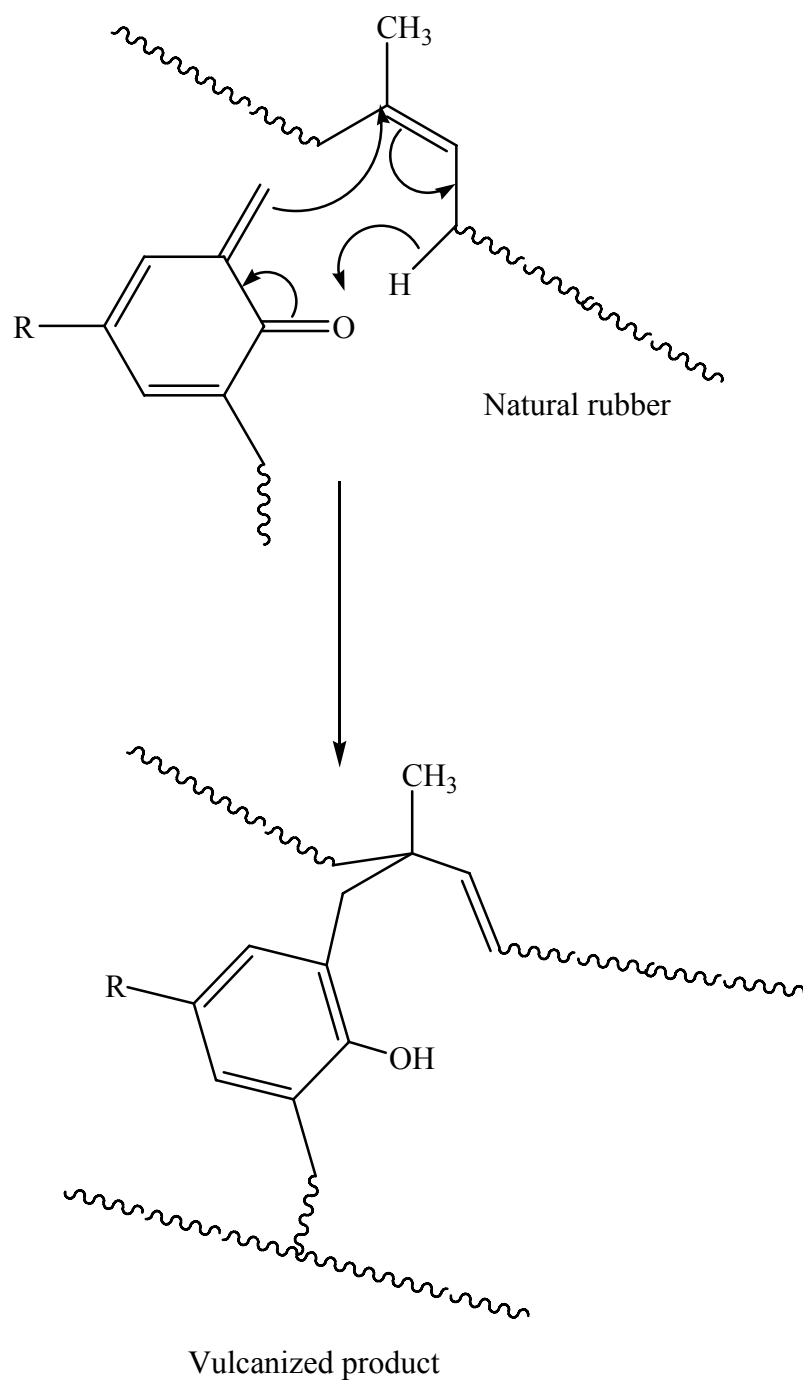
Figure 1. 12. Reaction of quinone methide with natural rubber
