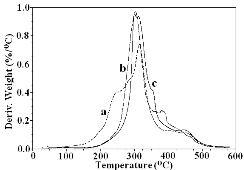
Figure 3.66. DTGA traces of a-) ethylene glycol, b-) glycerol, and c-) castor oil polythiourea.
