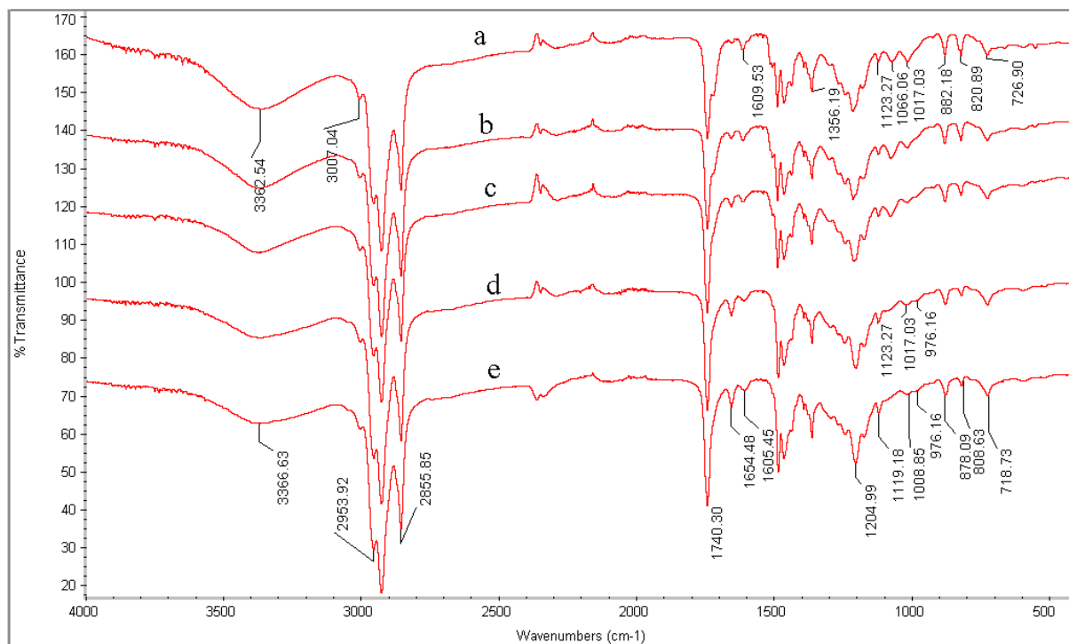
Figure 3. 13. IR spectra of methyl oleate and p. tertiary butyl phenol resoles (a) at starting, after (b) 10 minutes (c) 20 minutes (d) 30minutes and (e) 40 minutes at 190 °C.
