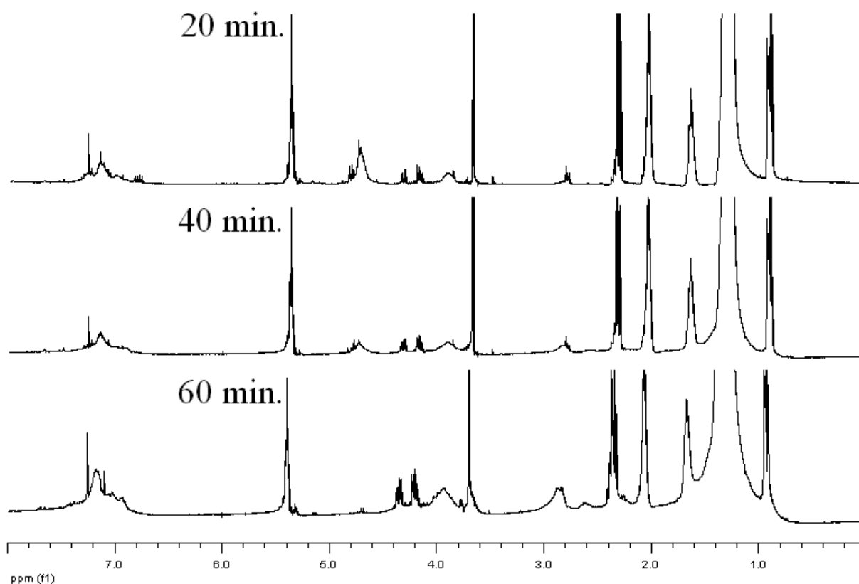
Figure 3.14. ^1\text{H} NMR s of the reaction mixture of methyl oleate and p. tertiary butyl phenol resole at 195 °C
