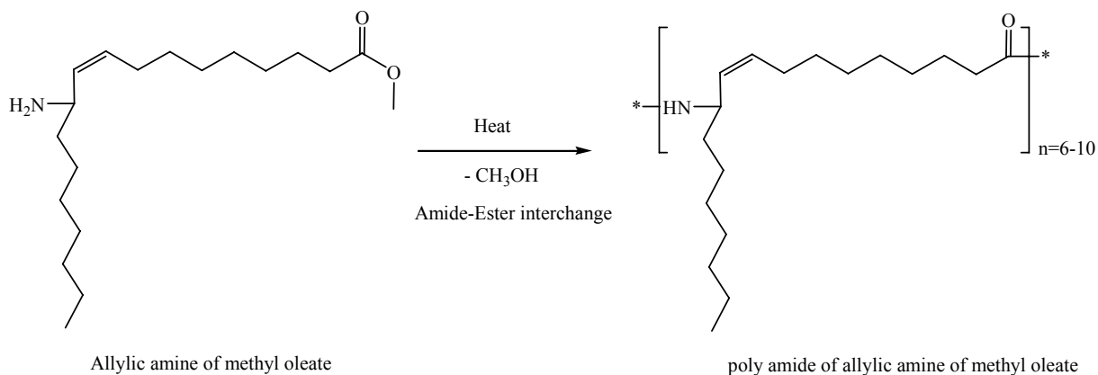
Figure 3.85. Polymerization of allyl amine of methyl oleate.
