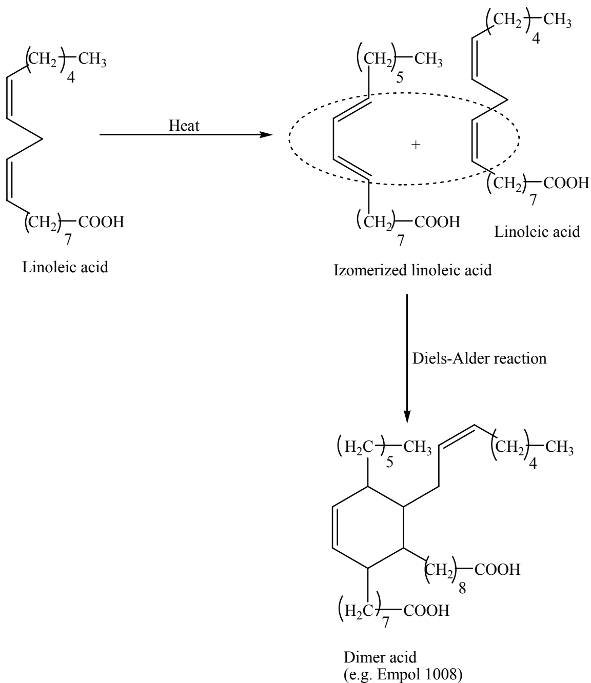
Figure 1. 13. Synthesis of dimer acids from linoleic acid [75].
