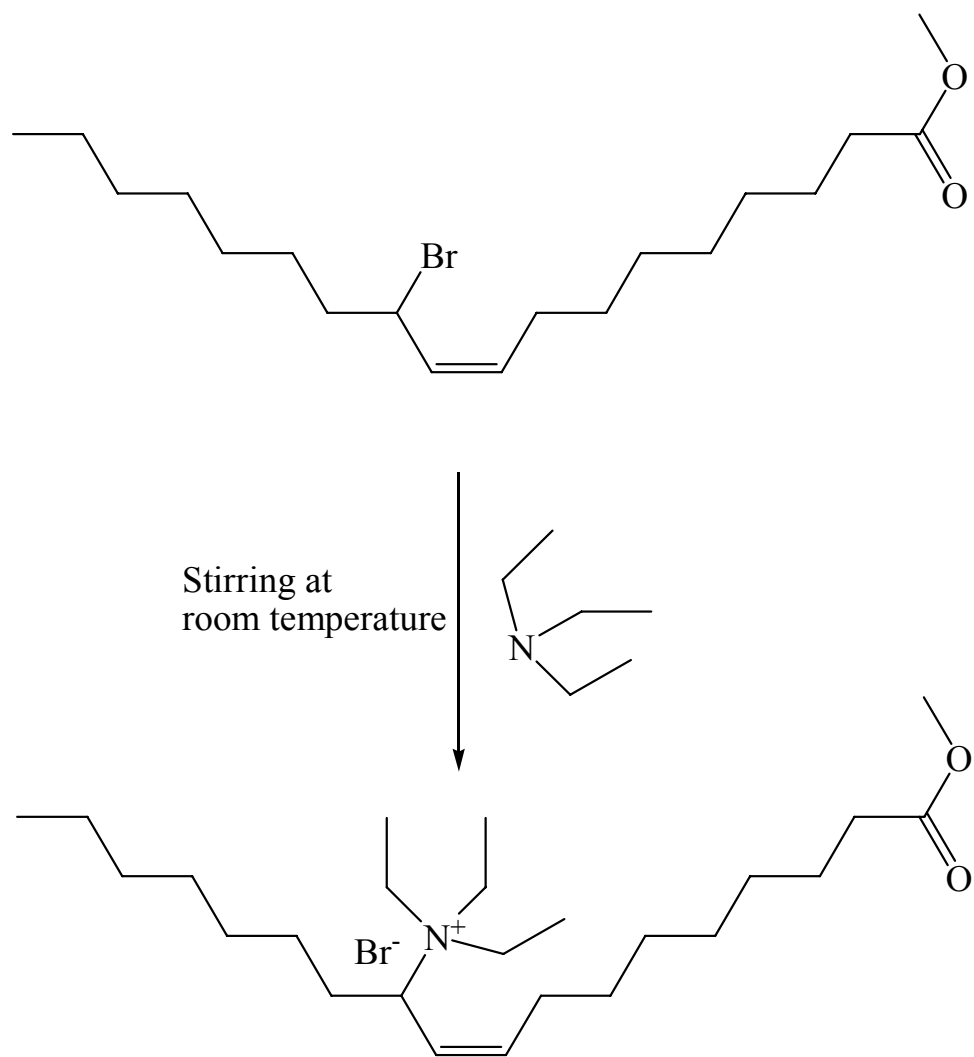
Figure 3.79. presentation of quaternarization of allylic bromines by using methyl oleate as a model compound.
