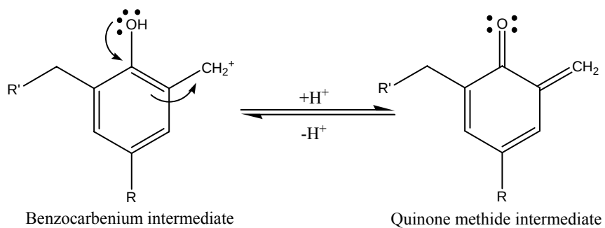
Figure 3.12. Transformation of quinine methide and benzocarbenium intermediates.
