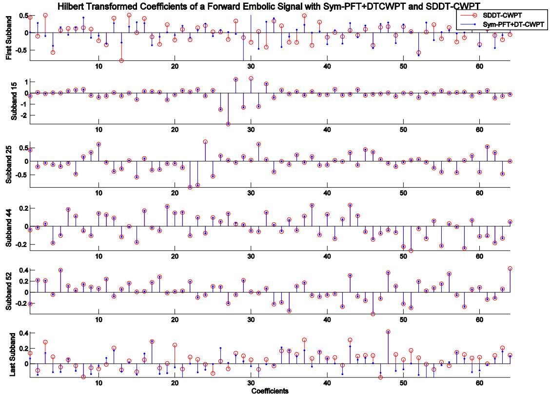
Figure 4.18 Hilbert transformed coefficients of a forward emboli signal obtained with proposed SDDT-CWPT and traditional method.
