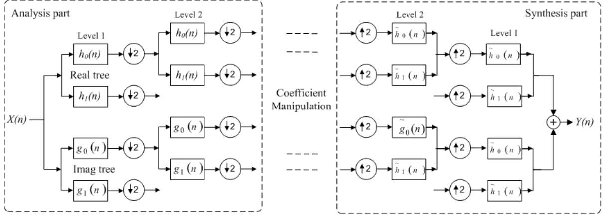
Figure 2.4 Block diagram for a 2-level DTCWT which demonstrates both analysis and synthesis parts. X(n) is the input signal and Y(n) is the processed signal.
