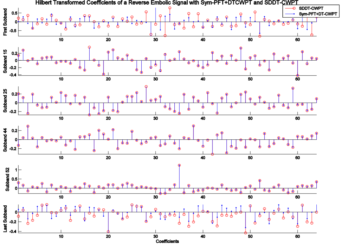
Figure 4.20 Hilbert transformed coefficients of a reverse emboli signal obtained with proposed SDDT-CWPT and traditional method.
