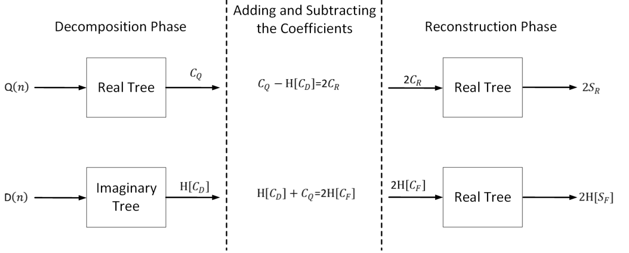
Figure 5.5 The structure of proposed directional DT-RADWT.
