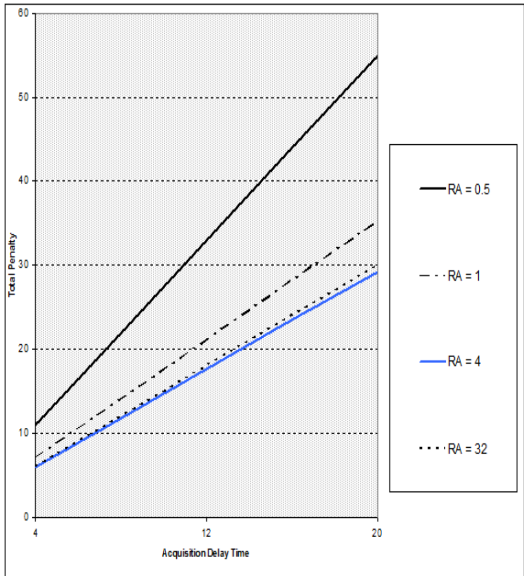
Figure 3.9. Acquisition Delay Time vs. Total Penalty when Weight of Supply Line = 0.75 and Delay is Discrete (Continuous Time) .
