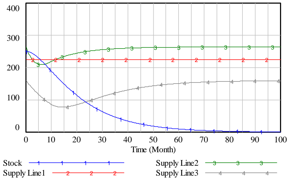
Figure 4.3. Stock and Supply Line Behaviors in a Three-Supplier System when Loss Flow is Constant and Stock does not start at its Desired Level.
