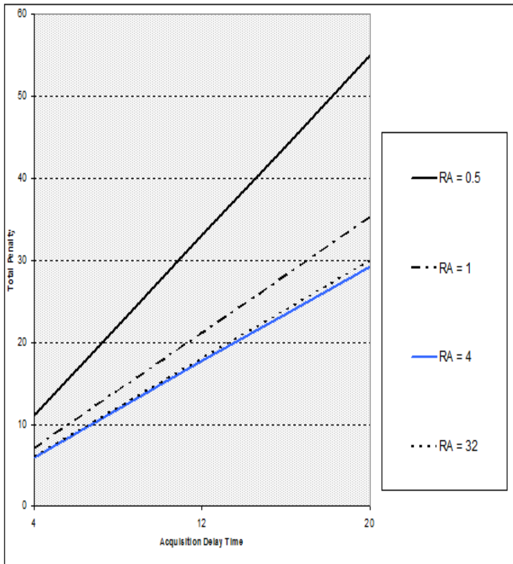
Figure 3.8. Acquisition Delay Time vs. Total Penalty when Weight of Supply Line = 0.75 and Delay Order is 1.
