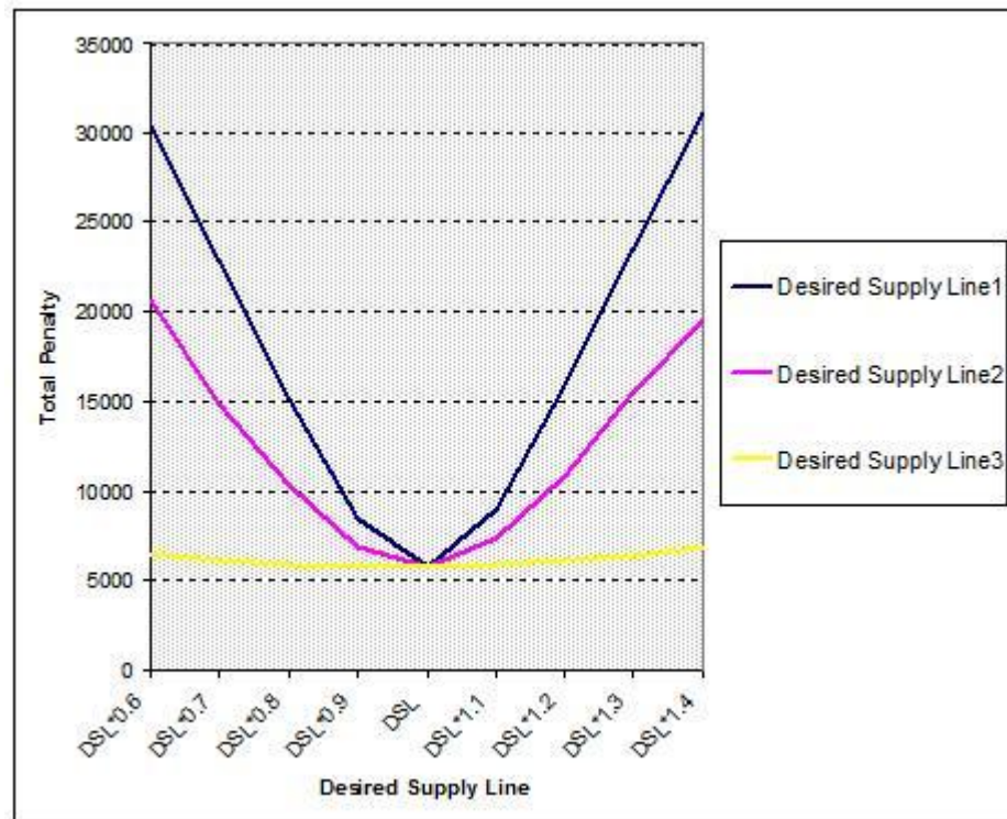
Figure 4.4. Total Penalty vs. Desired Supply Line Values.
