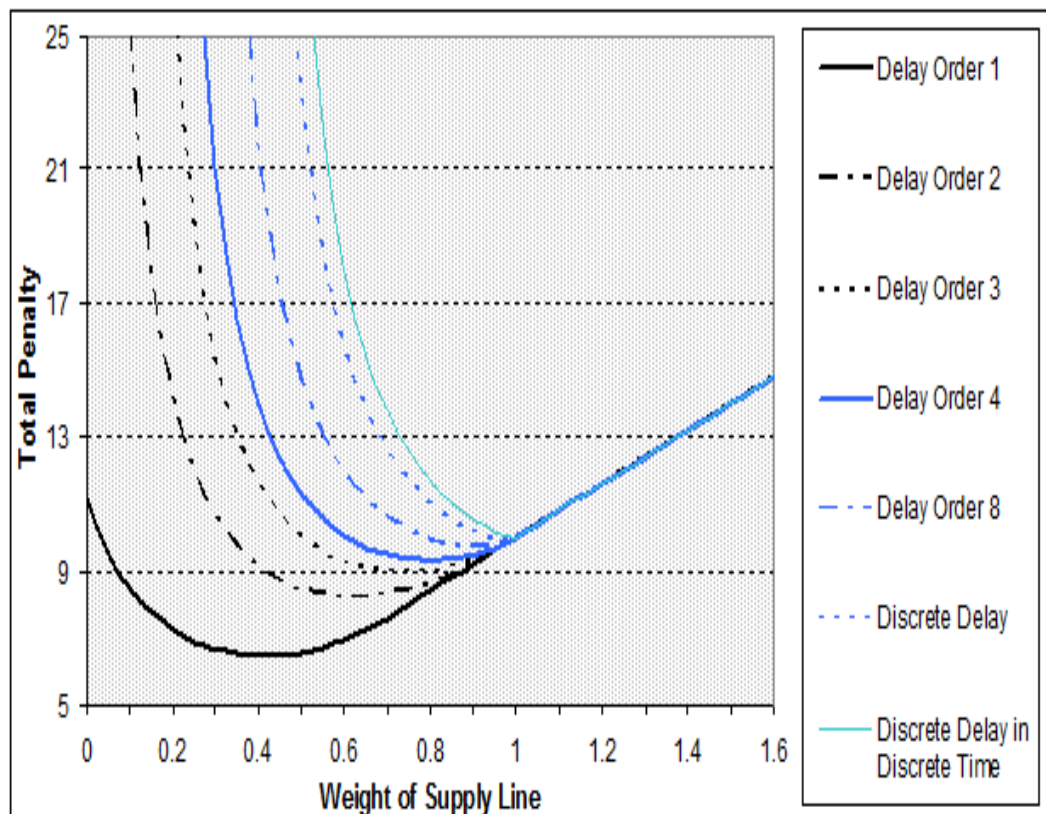
Figure 3.7. Total Penalty plotted against Weight of Supply Line when Relative Aggressiveness = 4.
