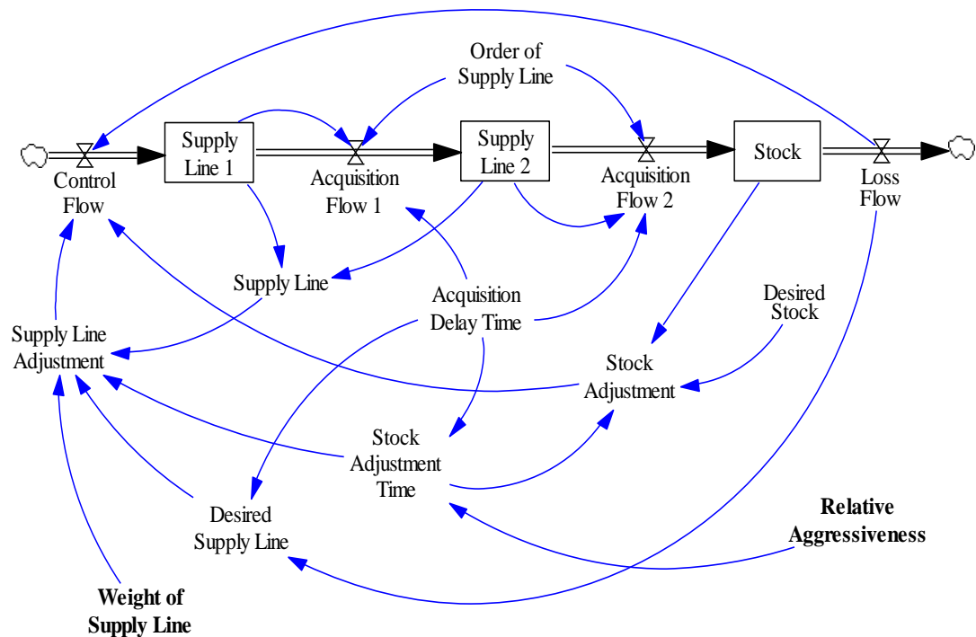
Figure 3.2. Stock-Flow Diagram of the Stock Management Task with a 2 nd Order Supply Line.
