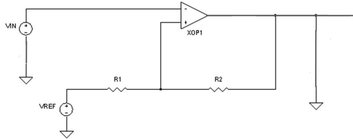
Figure 2.2 A sample comparator circuit with a hysteresis. In this thesis the reference voltage input ( V_{REF} ) was determined with the potentiometer on the device by user . The other input voltage V_{IN} produced by physical factor(infrared light) that was sensed by the detector.
