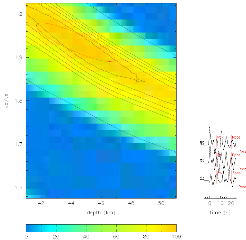
Figure 4.51. The H - \kappa stacking result for ANTB station.
