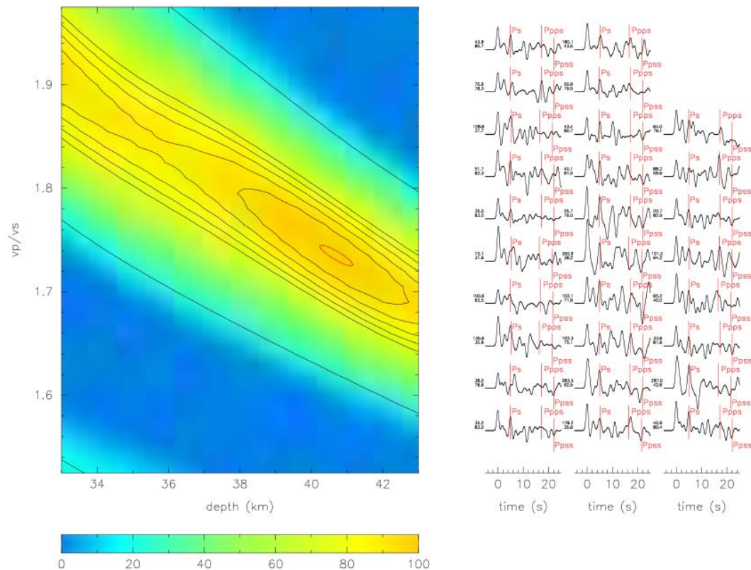
Figure 4.15. The H - \kappa stacking result for SALD station.
