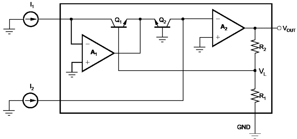
Figure 3.3 Log-ratio amplifier. [4]
