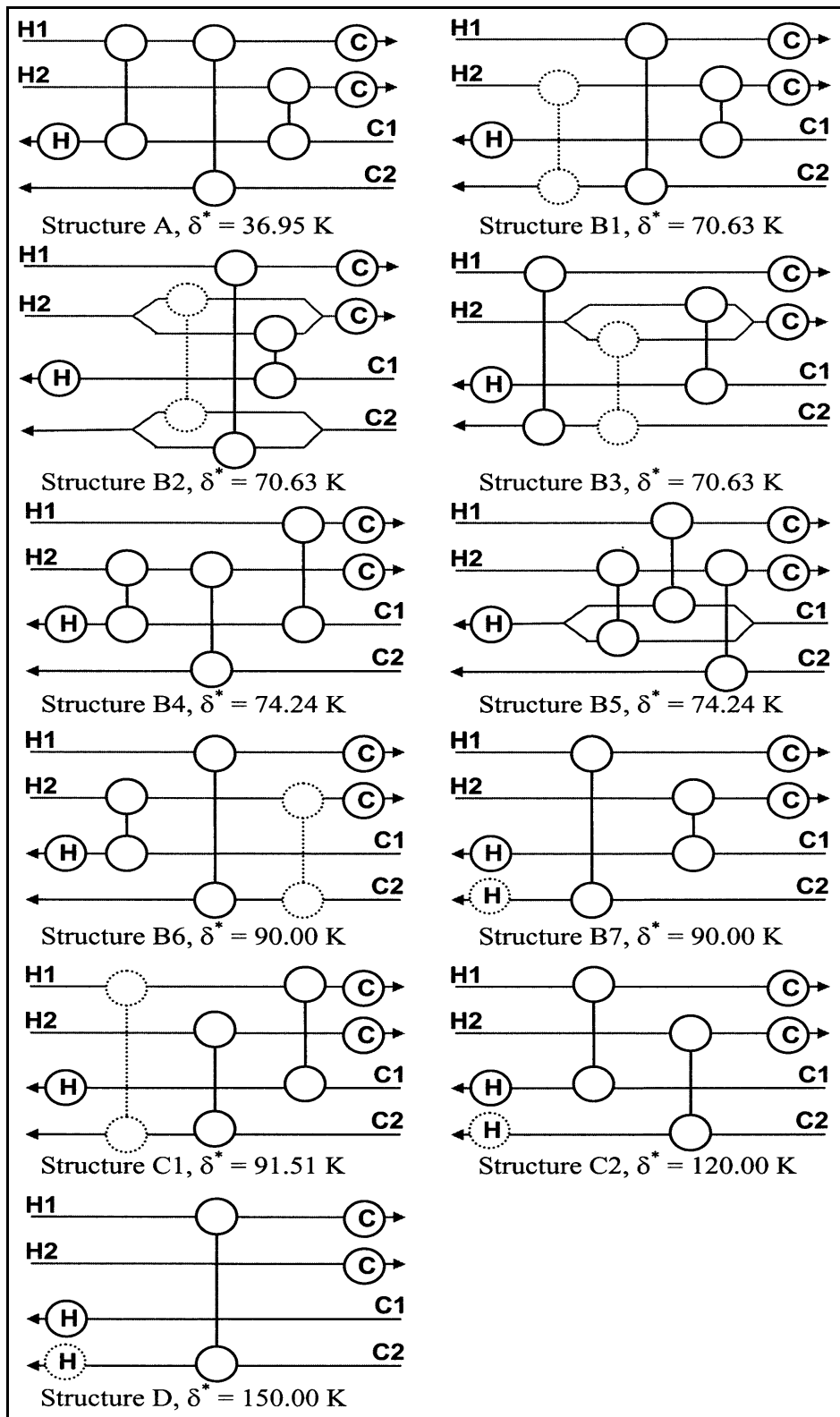
Figure 3.1. HEN structures (Konukman et al. , 2001)
