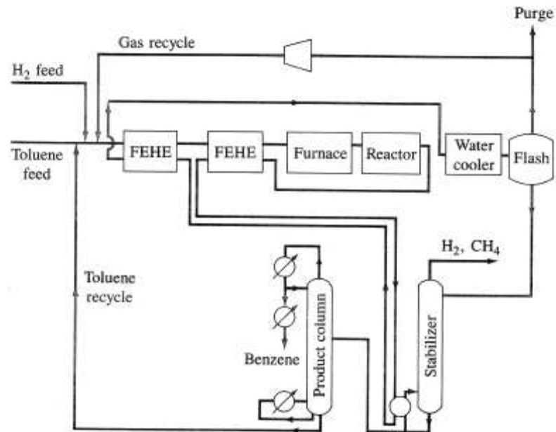
Figure 3.11. Flowsheet alternative 2 for the HDA process (Douglas, 1988)
