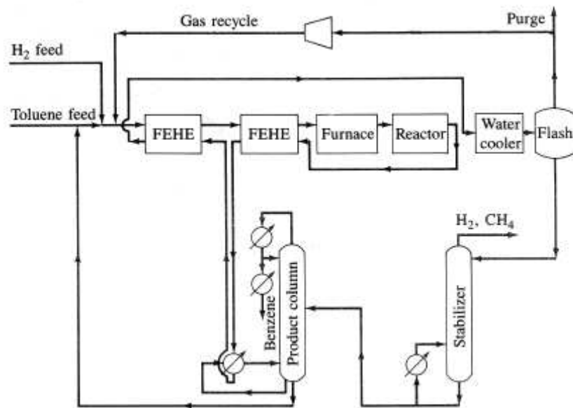
Figure 3.12. Flowsheet alternative 3 for the HDA process (Douglas, 1988)
