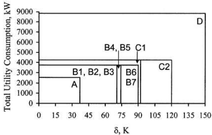
Figure 3.2. Total utility consumption versus the flexibility ranges of HEN structures (Konukman et al. , 2001)
