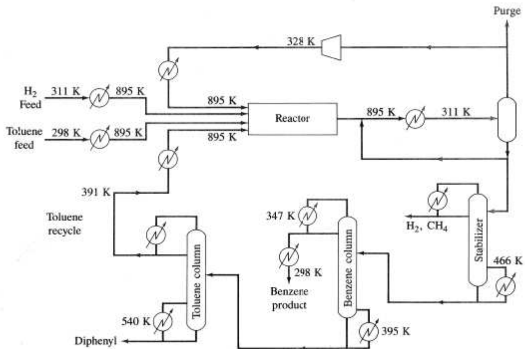
Figure 3.9. Flowsheet of the base-case HDA process (Douglas, 1988)
