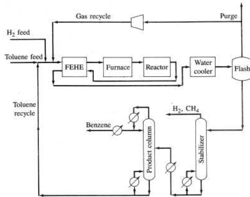
Figure 3.10. Flowsheet alternative 1 for the HDA process (Douglas, 1988)
