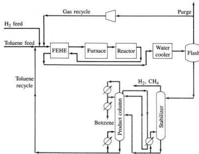
Figure 3.14. Flowsheet alternative 5 for the HDA process (Douglas, 1988)
