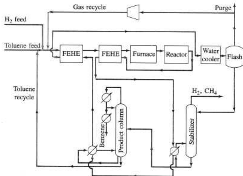
Figure 3.13. Flowsheet alternative 4 for the HDA process (Douglas, 1988)
