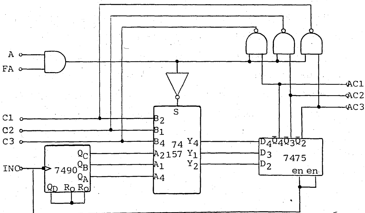
Figure 19: Channel incremter and channel selector circuit
