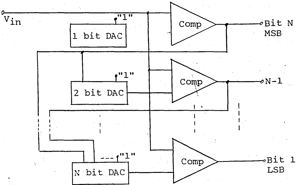
Figure 9: Variable threshold flash ADC
