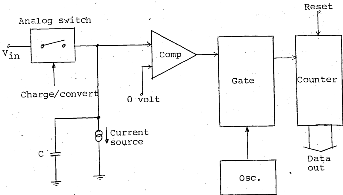
Figure 10: Wilkinson ADC
