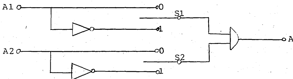
Figure 13: Address Sense circuit
