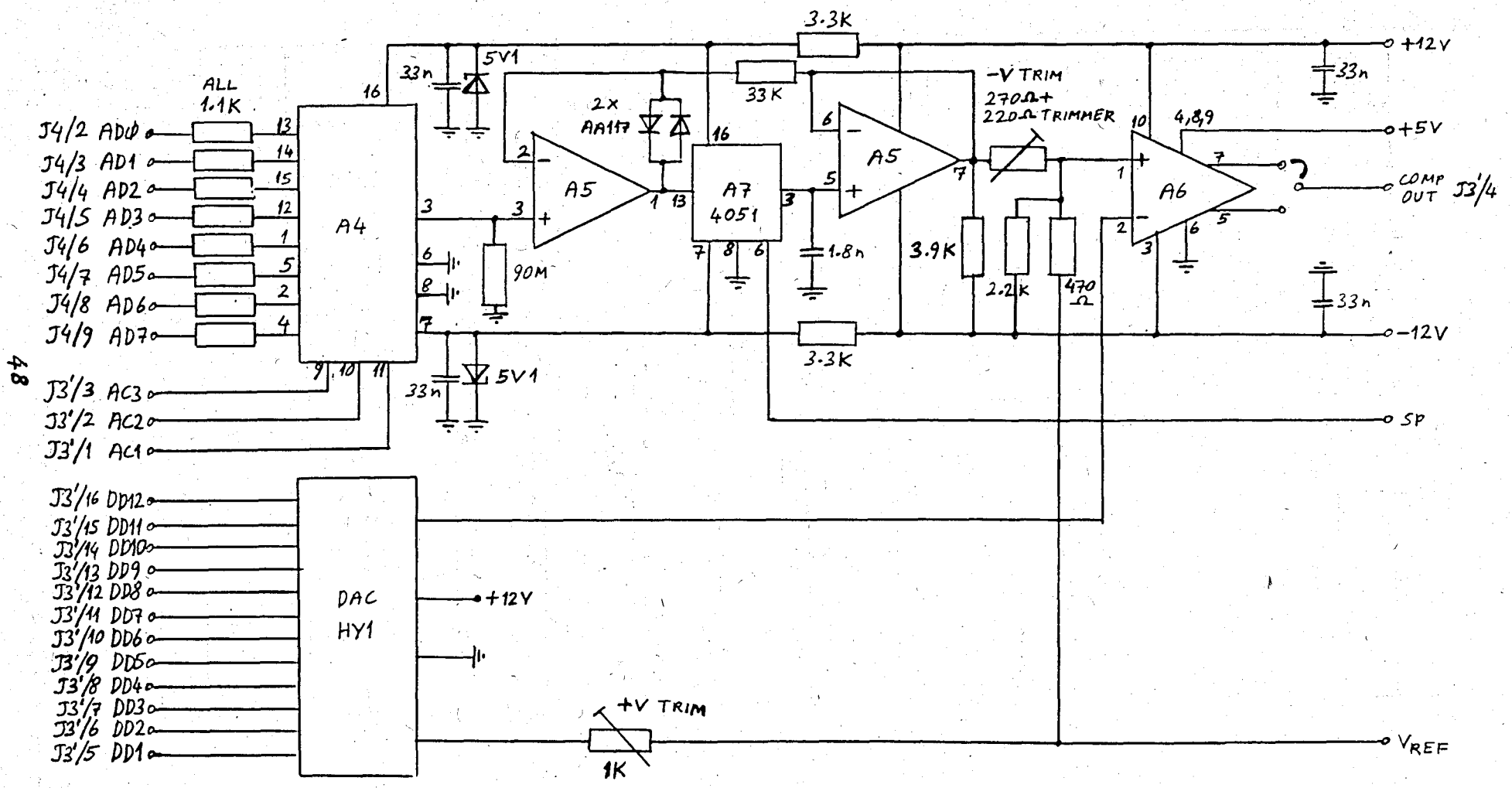
ANALOG MUX AND S/H
