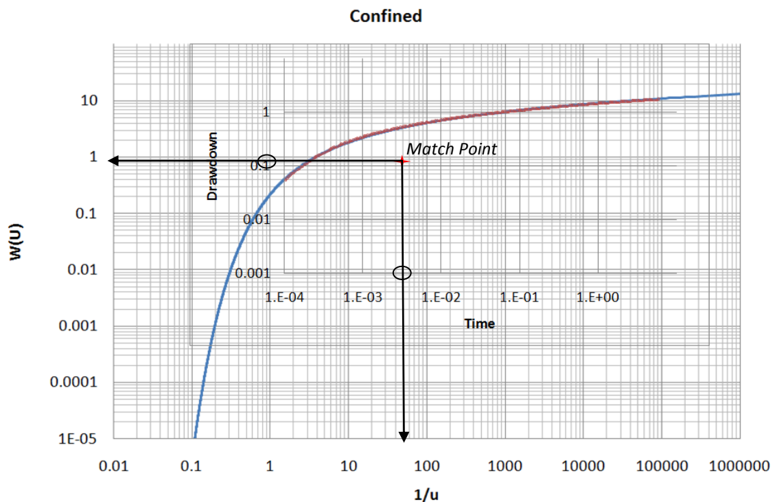
Figure 4.2. Theis graphical method, drawdown stated in red line
