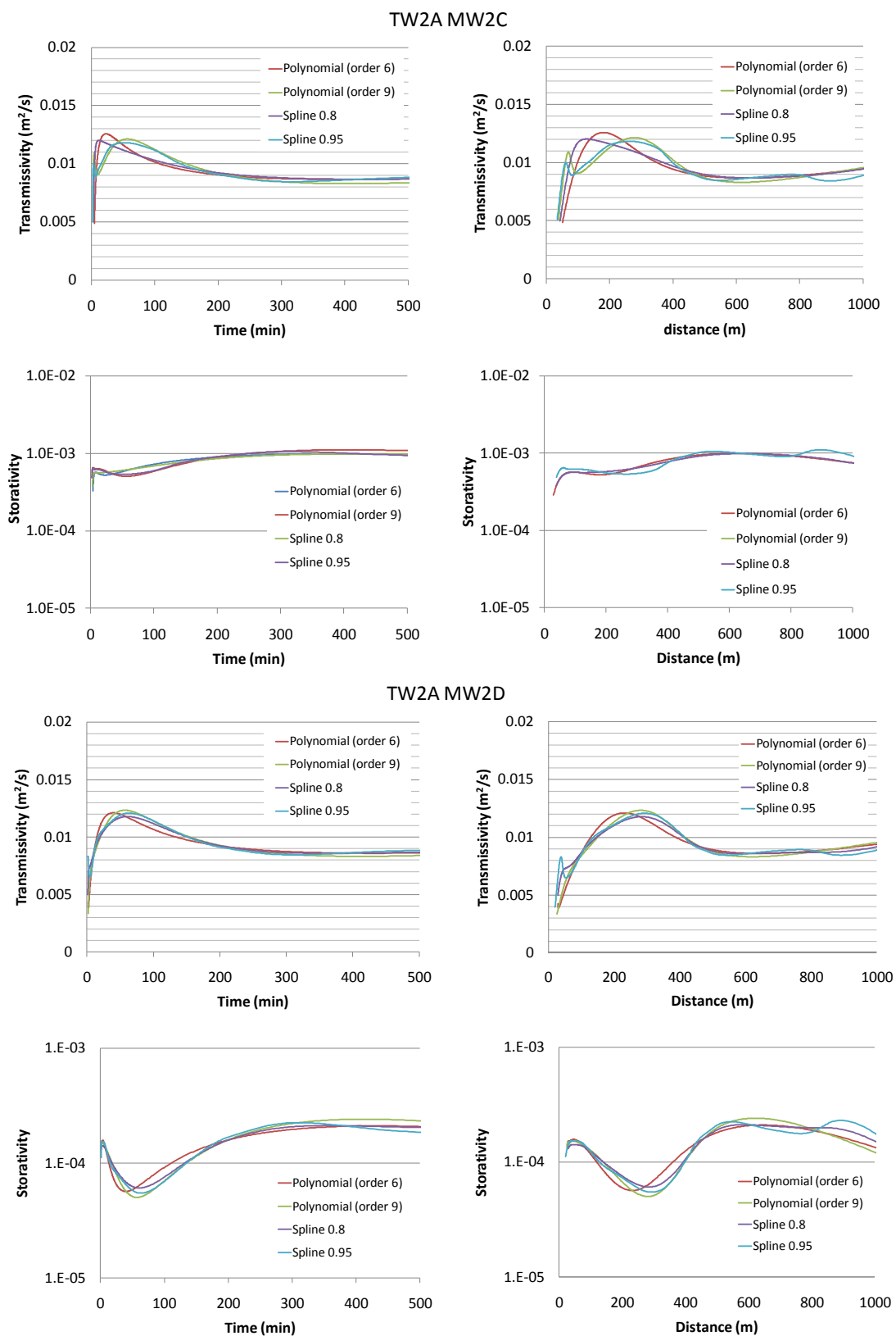
Figure 7.19. Estimation of flow parameters using the CD-Confined method for test wells 2C and 2D and for different drawdown fitting methods
