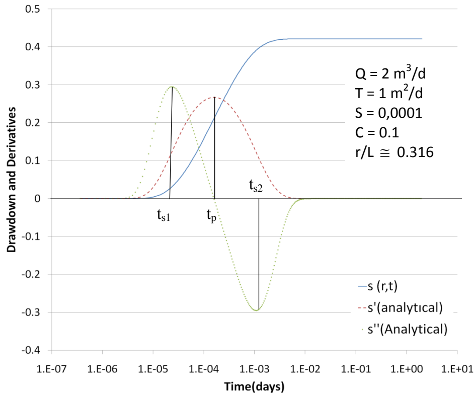
Figure 4.10. Drawdown and its first and second derivatives as a function of log time based on homogeneous assumption (from Trinchero et al., 2008)
