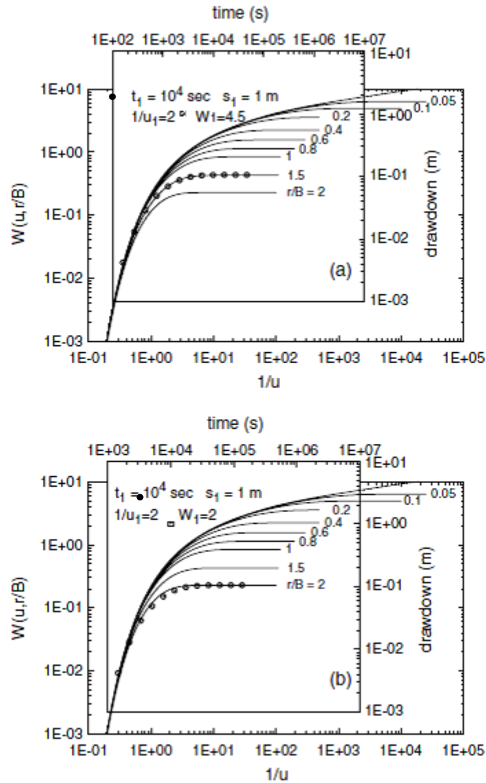
Figure 4.6. Interpretation of the synthetic pumping test using the type-curve method of Walton. Fit curves are a) r/B = 1.5 and b) r/B = 2.0 . (Trinchero et al., 2008)
