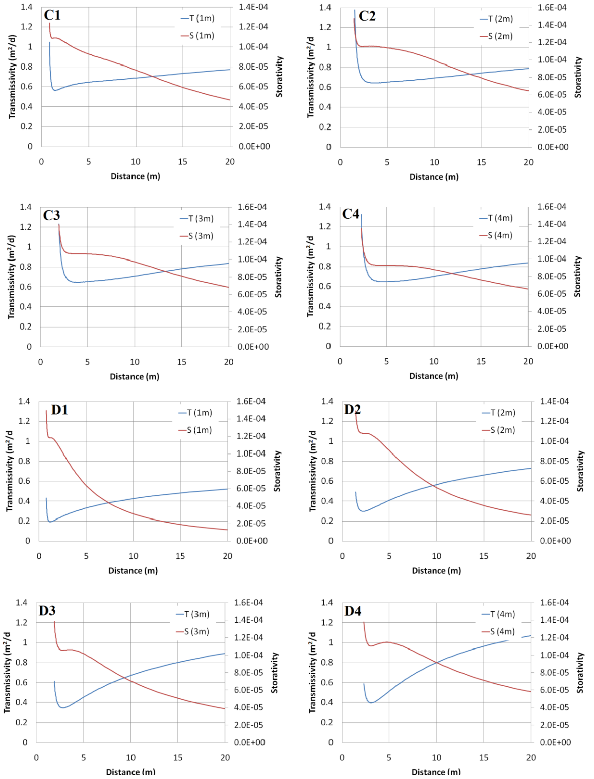
Figure B. 2. Estimations of CD-confined method from synthetic data for realizations C and D
