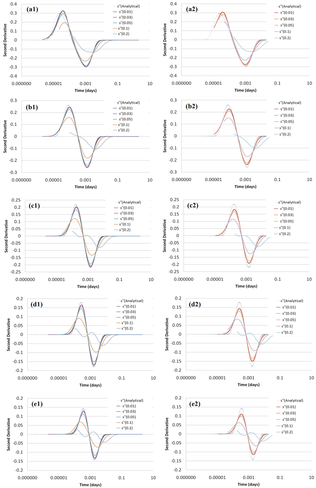
Figure 7.5. Comparison of second derivations calculated with the Spane method for (a):1 m, (b):2 m, (c):3 m, (d):4 m, (e): 5 m radius and. 1) L: 0.007; 2) L: 0.05
