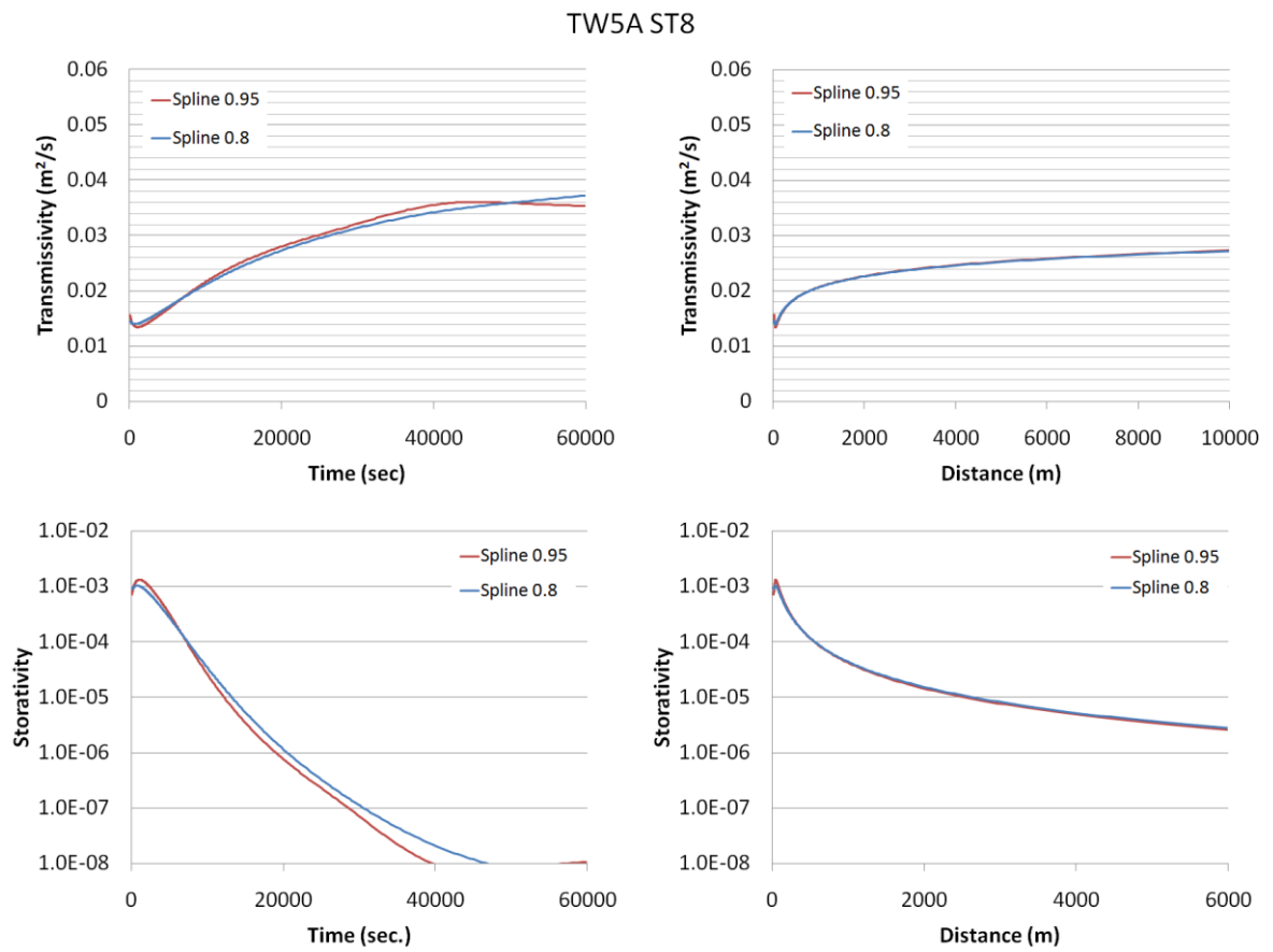
Figure C. 6. Estimations of CD-confined method from real data for ST8
