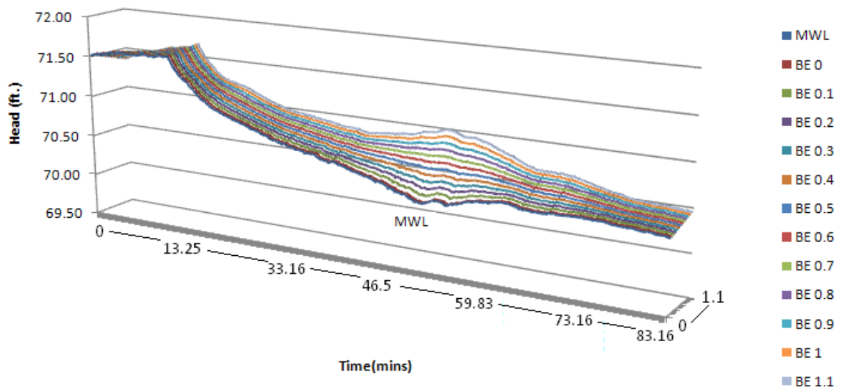
Figure 6.4. Elevation data from a monitoring well for different BE values to correction [The first line is MWL (Monitoring well level) also equal to BE = 0 curve, the best fit for this elevation data is BE = 0.6]
