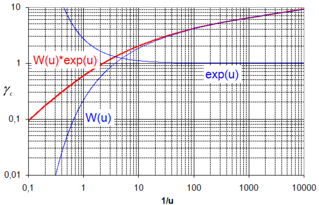
Figure 5.1. Plot of \gamma_c , ratio of drawdown to drawdown rate, as a function of 1/u (from Coptý et al., 2011)
